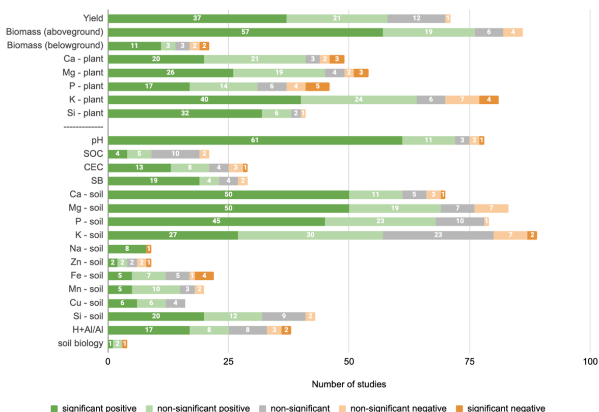
Figure 2. Summarized agronomic effects of 54 silicate agromineral experiments in Brazil. The count for significant positive (dark green), non-significant positive (light green), non-significant (gray), non-significant negative (light orange), significant negative (orange), and refers to comparisons to the negative control treatment. Various studies evaluated several rock, soil, and/or plant species, therefore the count exceeds 54 for some parameters.
