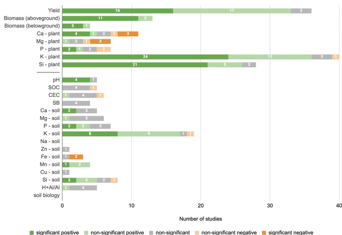
Figure 4. Summarized agronomic effects of 16 studies with potassium silicate agrominerals (ASiK) in Brazil. The count for significant positive (dark green), non-significant positive (light green), non-significant (gray), non-significant negative (light orange), significant negative (orange), and refers to comparisons to the negative control treatment.
