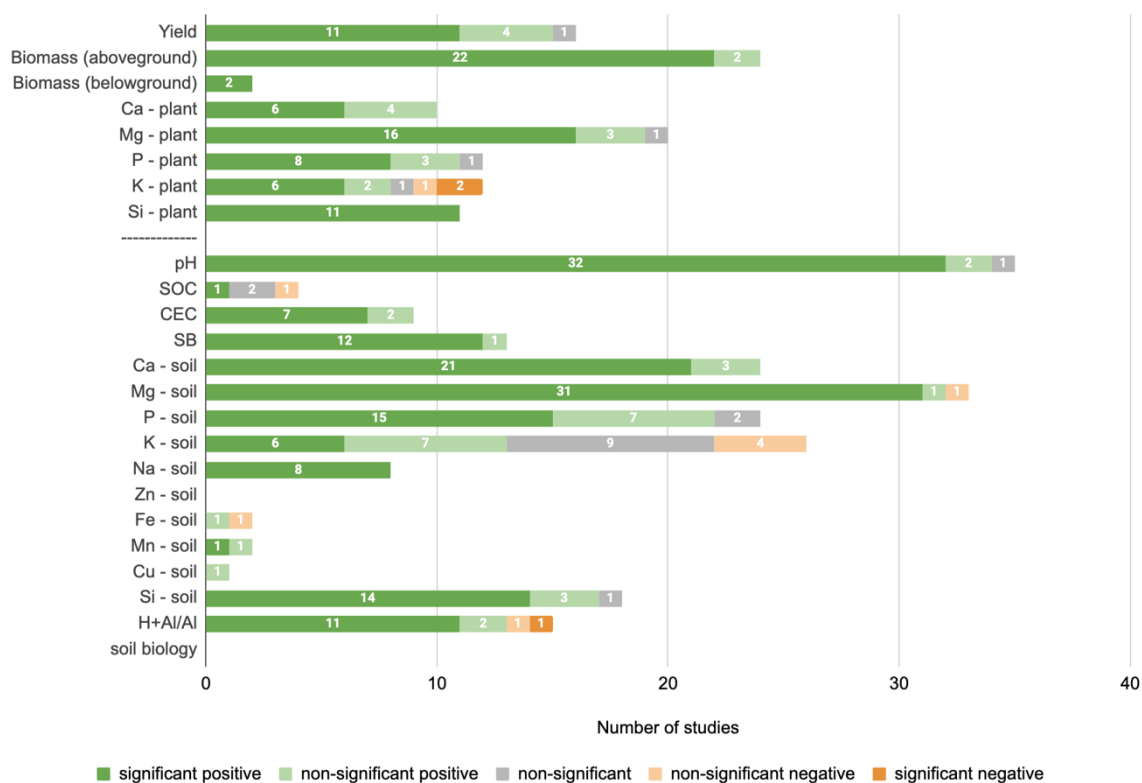
Figure 3. Summarized agronomic effects of 14 studies with silicate agrominerals (ASi) containing more than 20% sum of bases (SB r ) in Brazil. The count for significant positive (dark green), non-significant positive (light green), non-significant (gray), non-significant negative (light orange), significant negative (orange), and refers to comparisons to the negative control treatment.
