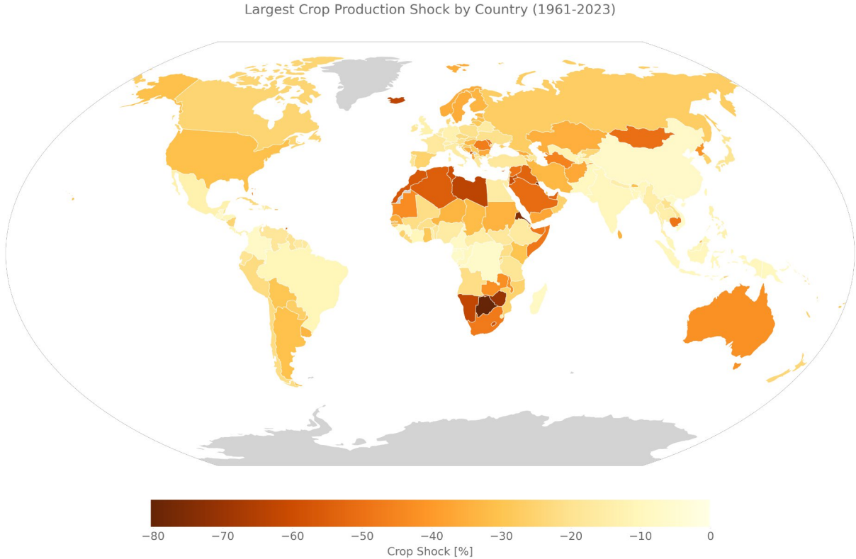
Figure 2: Largest crop production shock in all present-day countries. Darker colors indicate larger shocks. Grey indicates no data. The shocks are calculated as deviations from expected yield in a given year and are based on the combined calories from all assessed crops.
