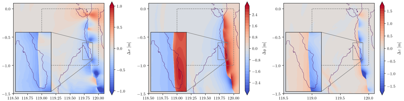
Fig. S5 Final horizontal ( \Delta x and \Delta y ) and vertical ( \Delta z ) surface displacements as computed by the earthquake model.
