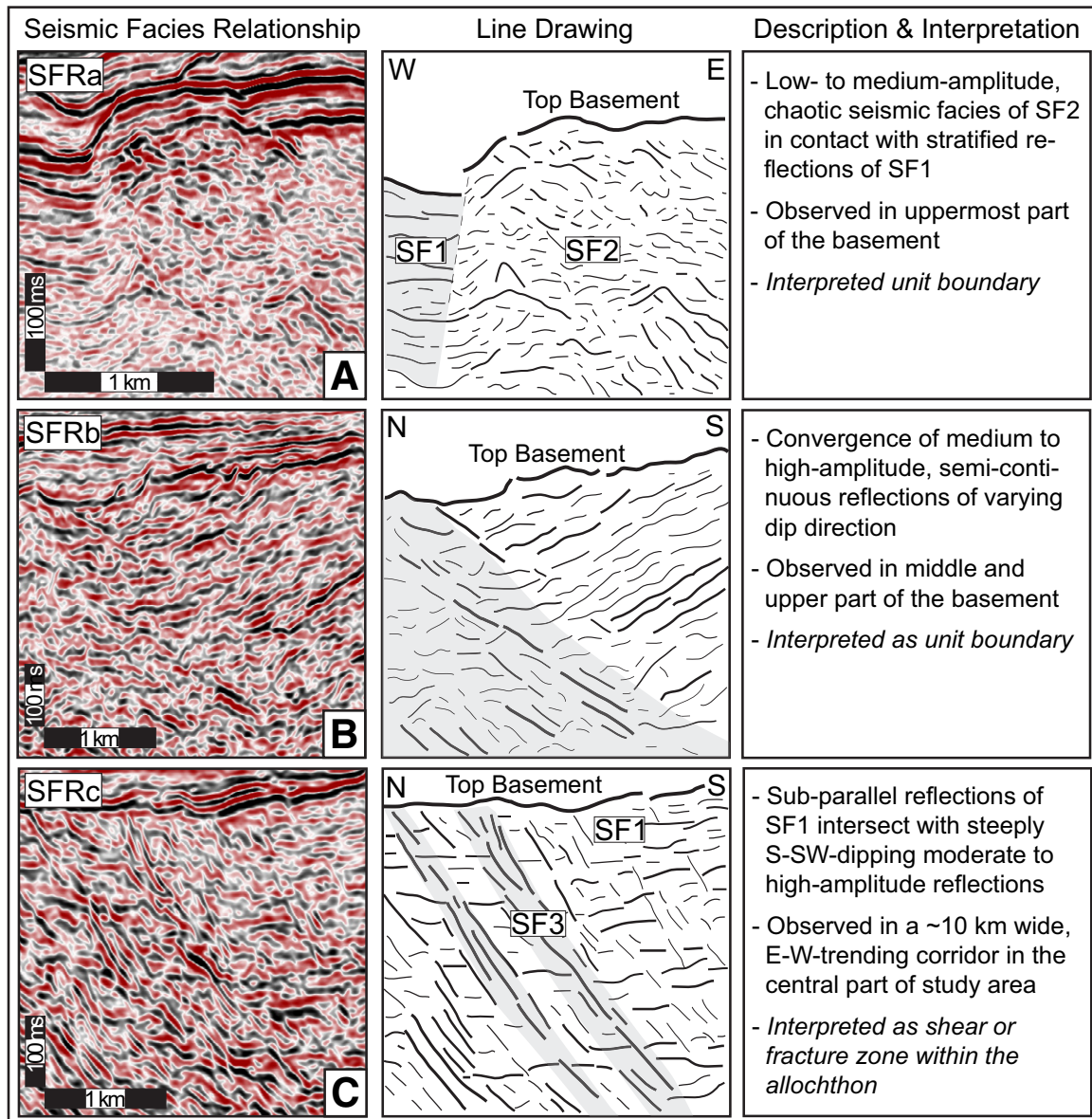
Figure 5. Seismic character, line drawing, and interpretation of geometrical relationships between different seismic facies relationships (SFRa, SFRb, SFRc). SF1–SF4—seismic facies 1–4.
