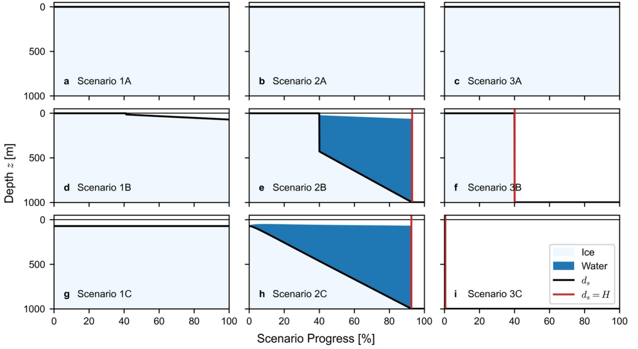
Figure 4. LEFM modelling scenarios. (a-i) Time-series evolution of crevasse and water depths under R_{xx} forcing scenarios A-C (from top-bottom) and d_w forcing scenarios 1-3 (from left-right). Vertical red lines mark the timing of full-depth fracture ( d_s = H ). Panel represent scenarios: (a) 1A; (b) 2A; (c) 3A; (d) 1B; (e) 2B; (f) 3B; (g) 1C; (h) 2C; and (i) 3C. Scenarios are presented graphically in Supplementary Fig. S6.
