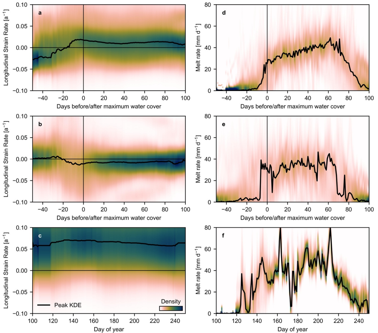
Figure 3. Aggregated longitudinal strain rates (left column) and runoff values (right column) for draining crevasses (top row), draining supraglacial lakes (middle row), and ‘dry’ crevasses that do not express surface water (bottom row). Colour scale represents Gaussian density estimates, and black line represents time series of highest Gaussian density estimate.
