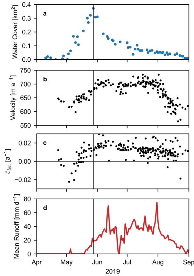
Figure 2. Evolution of exemplar crevasse field (lower-right field in Fig. 1c) over the 2019 season. (a) Total water cover. (b) Mean ITS_LIVE velocity. (c) Longitudinal strain rate, derived from ITS_LIVE velocity. (d) Mean RACMO daily runoff. Vertical black line marks maximum observed water cover.
