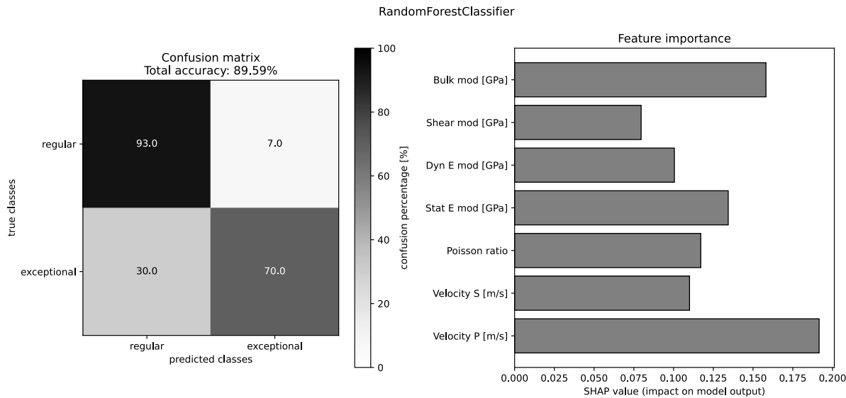
Figure 12: Performance of a Random Forest Classifier for binary rock classification (regular vs. exceptional). (Left) Confusion matrix showing per-class prediction rates; overall accuracy is 89.59%. (Right) SHAP-based feature importance indicating that seismic P wave velocities and elastic Bulk modulus are the dominant predictors.
