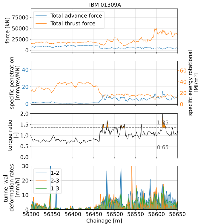
Figure 9: Detail view of the TBM operational data where favorable rock mass conditions are encountered up to ca. chainage 56450 und less favorable ones afterwards.
