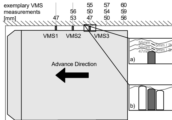
Figure 5: Graphical representation of how tunnel wall deformation rates can be derived from the VMS. a) detailed view with exemplary measurements and time differences between TBM advances of 2 and 3 hours respectively. b) sensitivity of the VMS to tunnel wall roughness.
