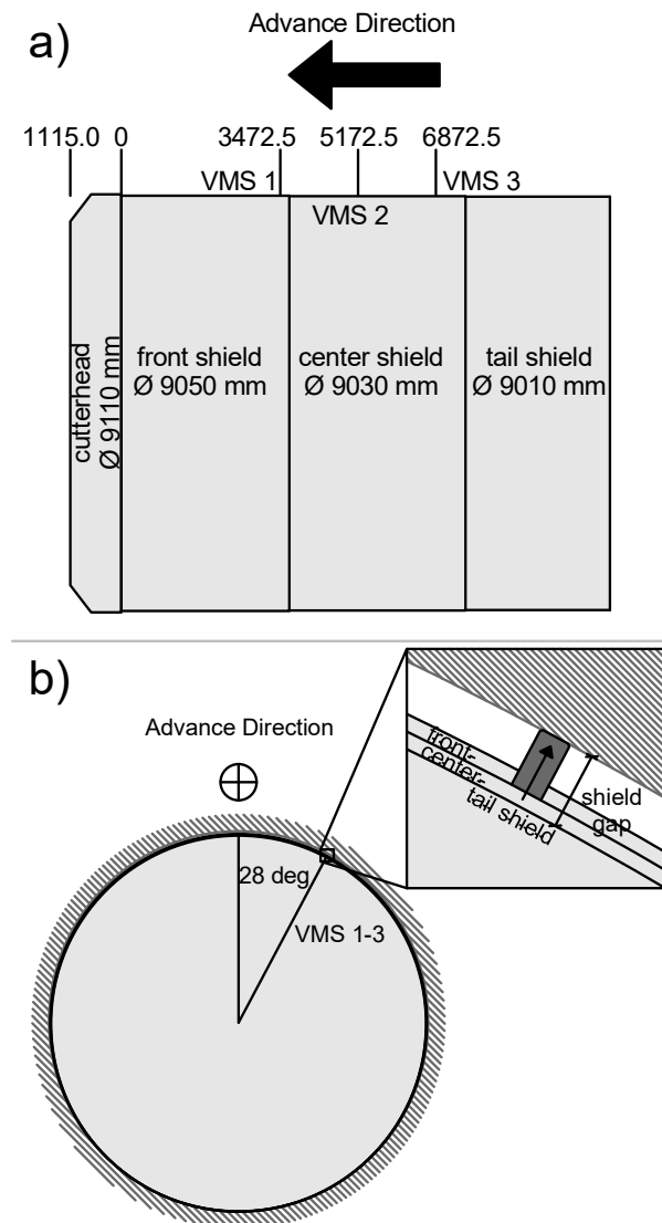
177 Figure 4: a) sideview of the TBM geometry and positions of the void measuring system (VMS). b) view in advance 178 direction showing the position of the VMS and a detailed view that shows VMS 3 fully extended.
