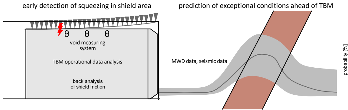
Figure 1: Schematic of the two data-driven development goals for the Rishikesh-Karnaprayag project. Left: an early detection system for squeezing in the shield area, right: a system to predict exceptional conditions ahead of the TBM.
