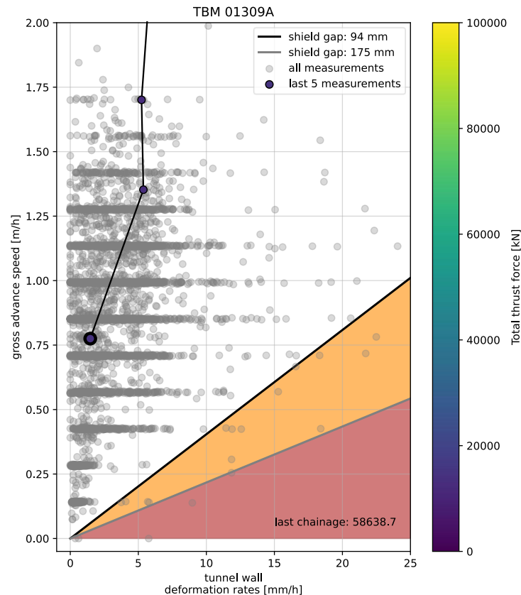
Figure 10: Novel methodology to predict the risk of squeezing in the shield area of a hard rock TBM, that relates the parameters tunnel wall deformation rate, TBM gross advance speed, length of the TBM shield and size of the shield gap. Orange and red areas indicate zones of elevated squeezing risk
