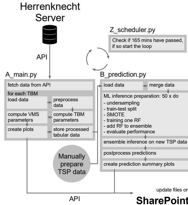
Figure 7: Detailed view of the computational data analysis framework.
