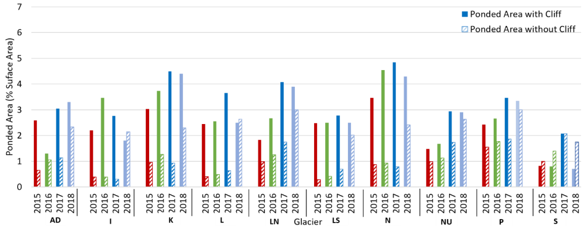
689 690 FIGURE 9: PERCENTAGE OF PONDS WITH AND WITHOUT ICE-CLIFFS, DISPLAYED AS PERCENTAGE OF TOTAL GLACIER 691 SURFACE AREA. AD- AMA DABLAM GLACIER, I- IMJA GLACIER, K- KHUMBU GLACIER, N- NGOZUMPA GLACIER, NU- 692 NUPTSE GLACIER, L- LHOTSE GLACIER, LN- LHOTSE NUP GLACIER, LS- LHOTSE SHAR GLACIER, P- PANGBUNG GLACIER, 693 S- SUMNA GLACIER.
