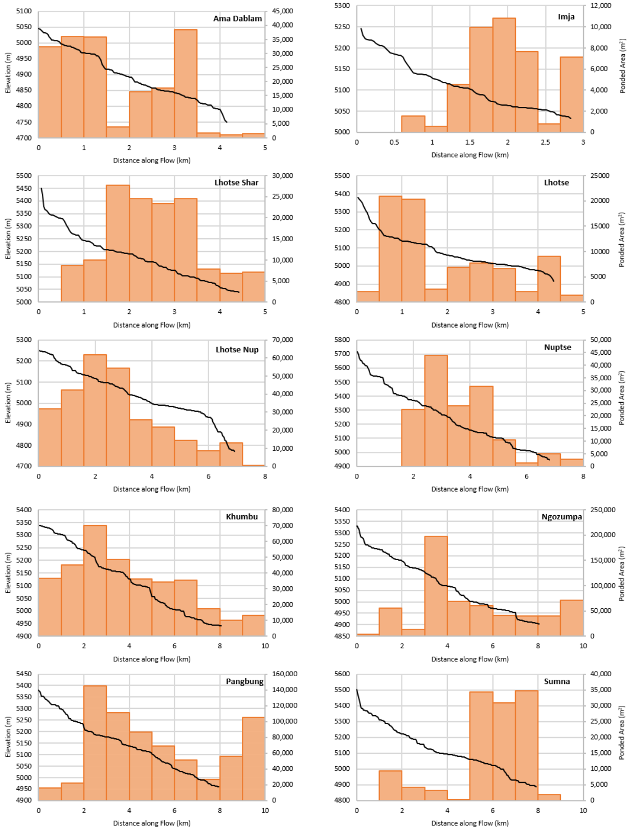
FIGURE 6: PONDED AREA FOUND ON THE GLACIER SURFACE APRIL 2018 COMPARED TO GLACIER ELEVATION/SLOPE AT 10% GLACIER AREA DISTANCE BANDS (0-10 = BAND 1, 10-20= BAND 2 ETC.)
