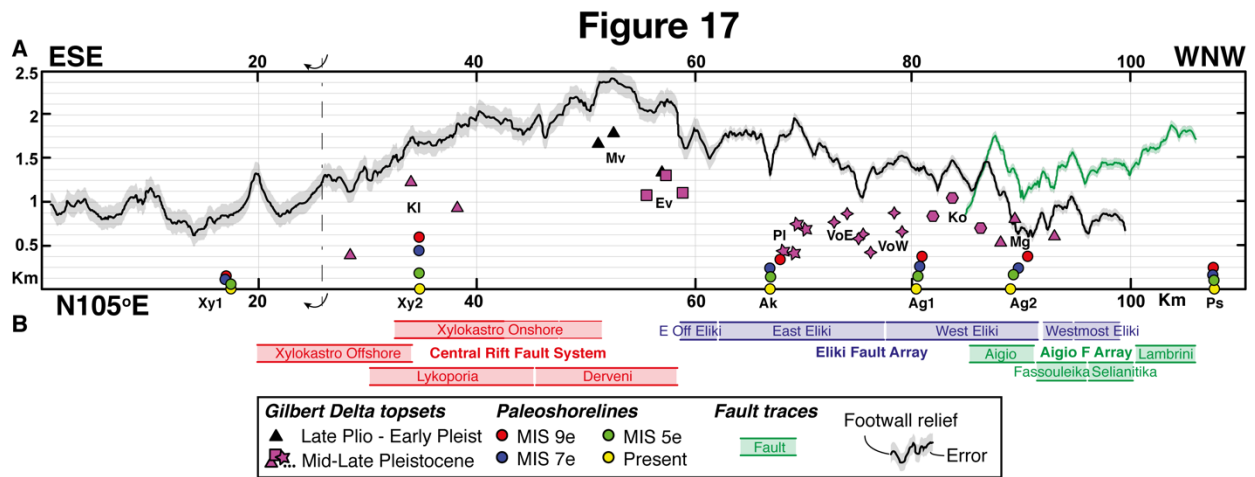
Fig. 17. Projection along master fault strike (N105E) of major morphotectonic features with known or correlated age with regards to the location of main fault segments. (A) Major morphotectonic elements of the master fault footwall and footwall relief. Filled circles represent the location of paleoshoreline angles of the MIS 5e (green), MIS 7e (blue) and MIS 9e (red) highstands of flights of marine terraces grouped by location. From E to W; Xy1 and Xy2, for Xylokastro area (paleoshoreline angles at low and maximum heights); Ak, for Akrata area; Aigio area, with Ag1 (paleoshoreline angles at the footwall of the Eiliki FA) and Ag2 (with MIS 5e and MIS 7e at its hanging wall and MIS 9e at its footwall); and Ps for Psathopyrgos (based on Armijo et al., (1996); De Martini et al., (2004); Houghton et al., (2003); McNeill & Collier, (2004)). Circles with yellow fill are the present day shoreline angles simplified as modern sea level (at 0 m), and are used only as a reference for the reconstructions in Figs. 18 & 19. Distinct filled geometric symbols represent the projection of the highest, lowest, eastmost and westmost location of the topsets of each Gilbert delta, as mapped in Fig. 6. Gilbert-delta topsets of Pleistocene age are in purple, while black triangles represent the topsets of the Late Pliocene - Early Pleistocene Mavro Gilbert delta. Gilbert deltas are label from E to W as KI (Klimentj), Mv (Mavro), Ev (Evrostini), PI (Platanos), VoE and VoW (Vouraikos, east and west), Ko (Kolokotronis) and Mg (Meganitis). In all cases, symbols are larger than associated errors. Footwall relief is defined as in Fig. 15. (B) Approximate location and extent of the main fault segments in the direction of projection.
