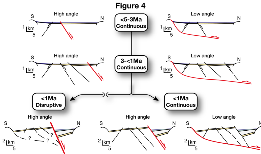
Fig. 4. Types of models proposed for the Corinth Rift in time, when classified by two key characteristics: mechanics at depth and evolutionary continuity.
