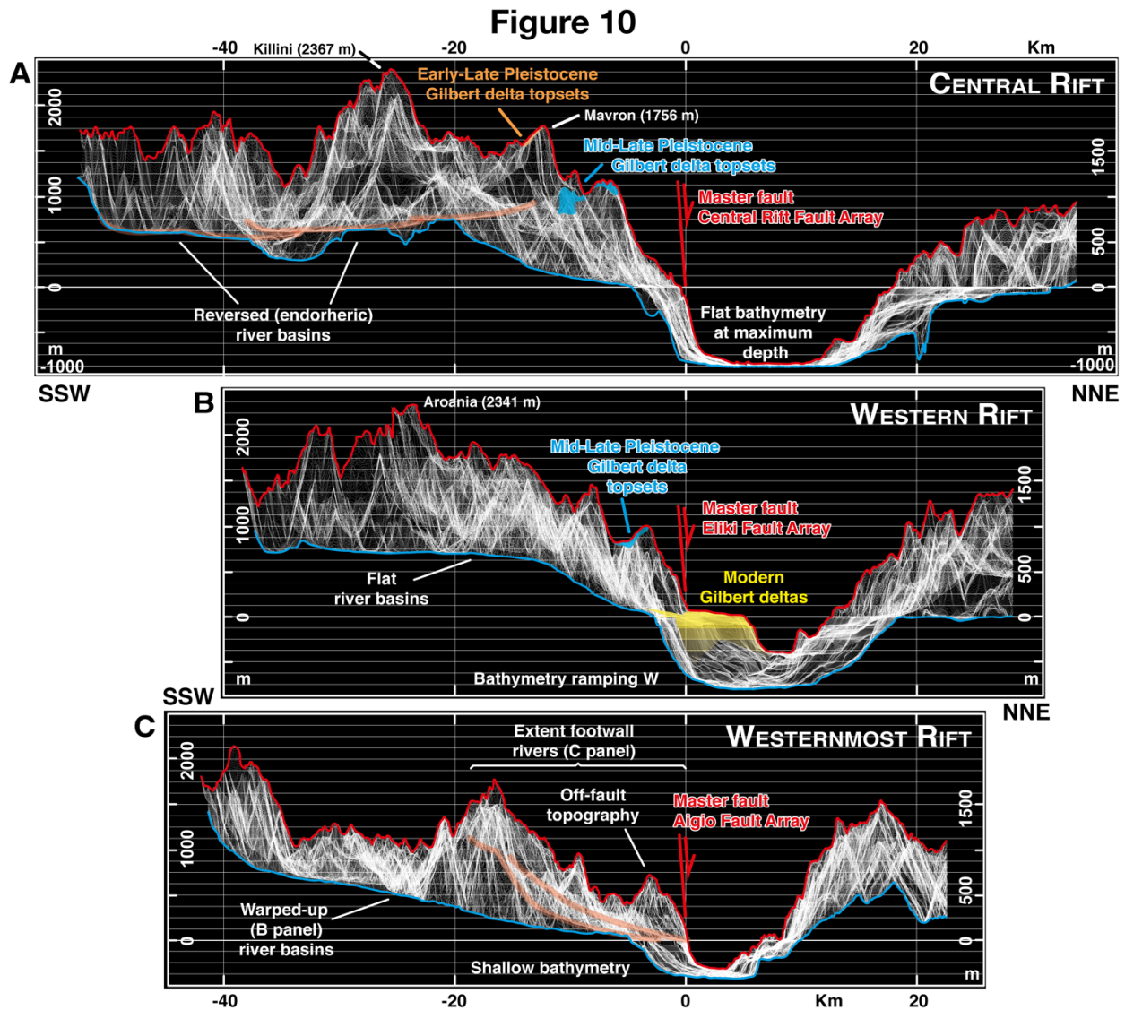
Fig. 10. Topobathymetry across the southern margin of the Corinth Rift in three “views” perpendicular to the current rift-bounding fault. Each ~26 km wide swath is composed of 400 swath profiles, stacked over a projection line perpendicular to the average strike of the main fault in each sector (see below). The width of each individual swath is calculated dynamically and of ~75 m. Relief is exaggerated ~8 times. Distance along each wide swath is measured from the master fault (positive northwards). (A) Topobathymetry associated with the Central Rift FA in a view looking towards N295°E. (B) Topobathymetry associated with the Eliki FA as seen looking in a N290°E direction. (C) Topobathymetry associated with the Aigio FA in a view looking towards N290°E. In all views the upper envelope (red line) and the lower envelope (blue line) represent the maximum and minimum topobathymetry, respectively. Each individual sector of the master fault is shown with a 55° north dip in red. Other associated features are shown: rivers and endorheic basins (dim red); topsets of Gilbert deltas in light brown (Late Pliocene - Early Pleistocene), blue (Mid-Late Pleistocene); and yellow for modern Gilbert Deltas.
