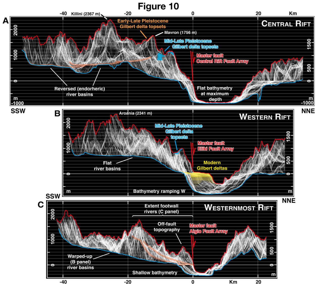
Fig. 10. Topobathymetry across the southern margin of the Corinth Rift in three “views” perpendicular to the current rift-bounding fault. Each \sim 26 km wide swath is composed of 400 swath profiles, stacked over a projection line perpendicular to the average strike of the main fault in each sector (see below). The width of each individual swath is calculated dynamically and of \sim 75 m. Relief is exaggerated \sim 8 times. Distance along each wide swath is measured from the master fault (positive northwards). (A) Topobathymetry associated with the Central Rift FA in a view looking towards N295^\circ E . (B) Topobathymetry associated with the Eliki FA as seen looking in a N290^\circ E direction. (C) Topobathymetry associated with the Aigio FA in a view looking towards N290^\circ E . In all views the upper envelope (red line) and the lower envelope (blue line) represent the maximum and minimum topobathymetry, respectively. Each individual sector of the master fault is shown with a 55^\circ north dip in red. Other associated features are shown: rivers and endorheic basins (dim red); topsets of Gilbert deltas in light brown (Late Pliocene - Early Pleistocene), blue (Mid-Late Pleistocene); and yellow for modern Gilbert Deltas.
