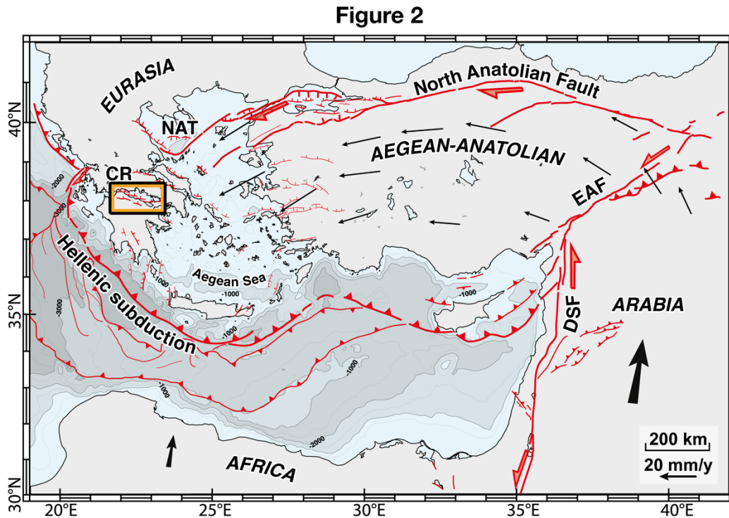
Fig. 2. Active tectonic faults and GPS velocities of the W Turkey-Greece region. The map shows the main tectonic units, plate boundaries and active faults in the region, and the location of the Corinth Rift (CR). The bathymetry is modified from Huguen et al. (2004). The GPS vectors, with a fixed Eurasian Plate, are simplified from Le Pichon and Kreemer (2010). The map of active faults comes from Armijo et al. (1999) and Flerit et al. (2004) for the Aegean and North Anatolian areas, and Kreemer & Chamot-Rooke (2004) for the Mediterranean Ridge area. Line thickness and arrow size represent amount of slip to a first-order. NAF and EAF are the North and East Anatolian faults.
