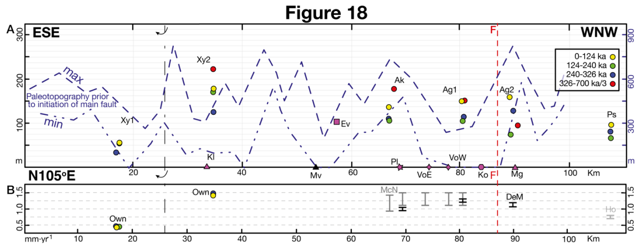
Fig. 18. Flexure geometry and evolution in time of the rift-forming fault of the Corinth Rift along strike, marked by relative elevation and age constraints of footwall morphotectonic elements, and pre-fault paleotopography. (A) Reconstruction in time-frames of main fault relative vertical motions. Symbols represent the relative elevations between two consecutive sets of morphotectonic markers formed at sea level. We applied specific corrections to consecutive markers that represent longer time-steps to plot roughly equivalent time-steps (~110 ka). Yellow circles: Present to 124 ka (124 ka). Green: 240 ka to 124 ka (115 ka). Blue: 326 ka to 240 ka (91 ka). Red: ~700 ka to 326 ka / 3 (~123 ka). Purple symbols: ~1 Ma to ~700 ka / 3 (~100 ka). Envelopes of estimated maximum and minimum paleotopography prior to the formation of the main fault are shown as a blue line with triple vertical scale. (B) Uplift rates of the marine terraces during aforementioned time frames and equivalent colors to those in panel (A) for own analysed terraces, and proposed ranges of uplift rates from Houghton et al., 2003 (Ho), McNeill and Collier, 2004 (McN) and DeMartini et al., 2003 (DeM).
