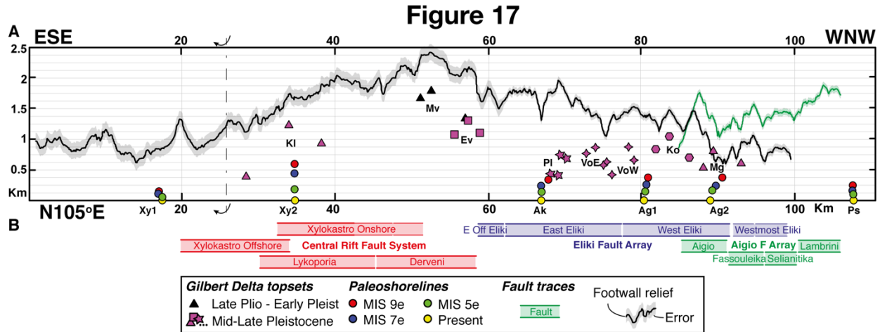
Fig. 17. Projection along master fault strike (N105°E) of major morphotectonic features with known or correlated age with regards to the location of main fault segments. (A) Major morphotectonic elements of the master fault footwall and footwall relief. Filled circles represent the location of paleoshoreline angles of the MIS 5e (green), MIS 7e (blue) and MIS 9e (red) highstands of flights of marine terraces grouped by location. From E to W; Xy1 and Xy2, for Xylokastro area (paleoshoreline angles at low and maximum heights); Ak, for Akrata area; Aigio area, with Ag1 (paleoshoreline angles at the footwall of the Eliki FA) and Ag2 (with MIS 5e and MIS 7e at its hanging wall and MIS 9 at its footwall); and Ps for Psathopyrgos (based on Armijo et al., (1996); De Martini et al., (2004); Houghton et al., (2003); McNeill & Collier, (2004)). Circles with yellow fill are the present day shoreline angles simplified as modern sea level (at 0 m), and are used only as a reference for the reconstructions in Figs. 18 & 19. Distinct filled geometric symbols represent the projection of the highest, lowest, eastmost and westmost location of the topsets of each Gilbert delta, as mapped in Fig. 6. Gilbert-delta topsets of Pleistocene age are in purple, while black triangles represent the topsets of the Late Pliocene - Early Pleistocene Mavro Gilbert delta. Gilbert deltas are label from E to W as Kl (Klimenti), Mv (Mavro), Ev (Evrostini), Pl (Platanos), VoE and VoW (Vouraikos, east and west), Ko (Kolokotronis) and Mg (Meganitis). In all cases, symbols are larger than associated errors. Footwall relief is defined as in Fig. 15. (B) Approximate location and extent of the main fault segments in the direction of projection.
