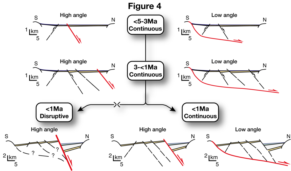
Fig. 4. Types of models proposed for the Corinth Rift in time, when classified along two main topics: mechanics at depth and evolutionary continuity.
