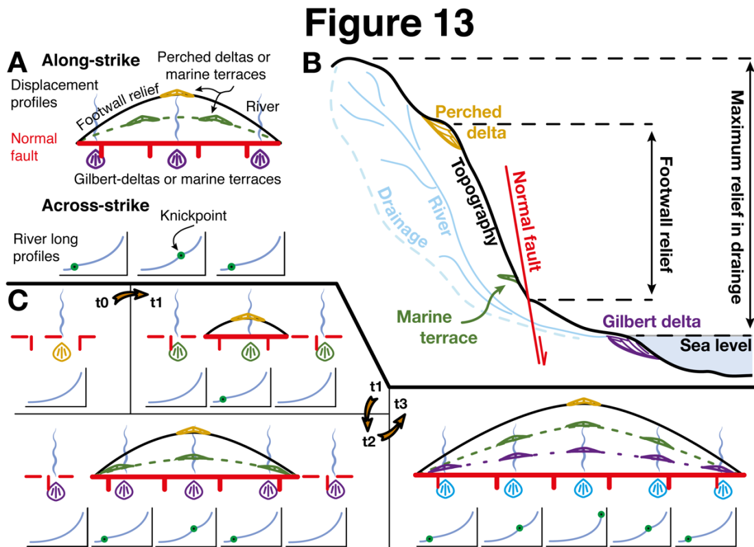
Fig. 13. (A) Schematic representation of elements in extensional footwalls in relation with their active faults in an along-strike view and footwall rivers and their tectonic knickpoints in across-strike view. (B) Elements of an extensional footwall and their relation with the proxies of relief used in this study. (C) Self-similar growth of a normal fault, as shown by geomorphic features in its footwall, in four time-steps: (t0) steady-state of a river network - Gilbert delta system; (t1) initiation of normal fault activity and footwall flexural uplift propels formation of a tectonic knickpoint and uplifts former Gilbert deltas; (t2) lateral growth of the normal fault leads to inclusion of rivers in its footwall, and the formation of new tectonic knickpoints and uplift of new Gilbert-deltas; (t3) lateral self-growth and perpetuation of t2. Similar constraints by Gilbert-deltas on fault displacement profile (albeit more accurate) can be inferred using marine terraces. Other inferences on fault displacement profiles can be obtained from footwall relief and total topography. Assuming that geomorphic features formed at each time-step are not eroded and can be dated, their location and height provide key constraints on the fault growth and displacement profile in time.
