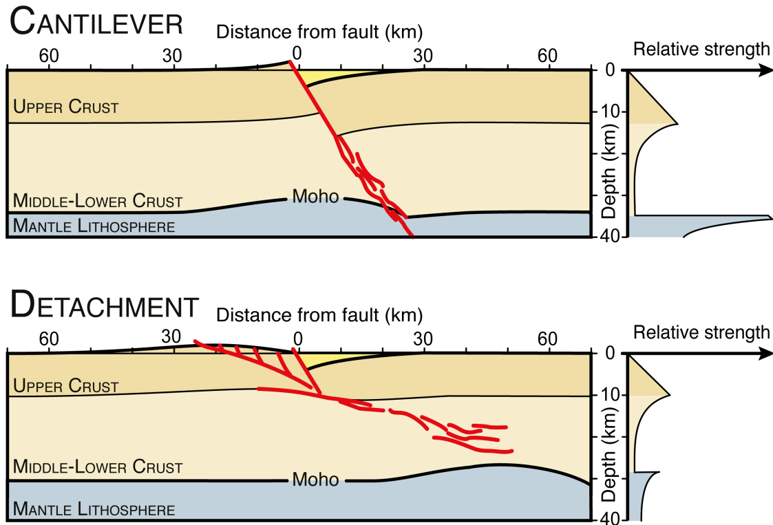
Fig. 1. End-member models for intracontinental rifts and representative strength profiles. In the upper section is the flexural-cantilever rift model (Kusznrir et al., 1991), and in the lower section is the core complex-detachment rift model (Buck, 1991). Their representative strength profiles are shown to the right of each model.
