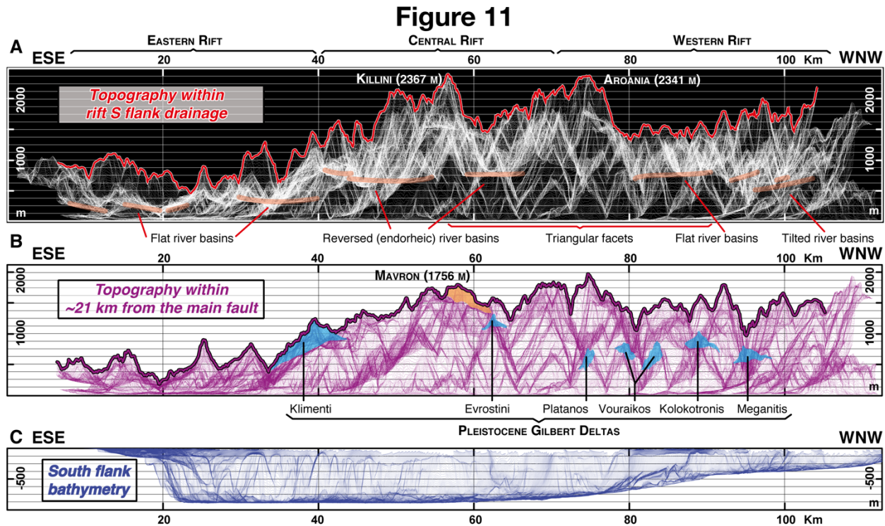
Fig. 11. Stacked swath profiles of topography and bathymetry along the southern flank of the Corinth Rift in a view parallel to the master fault. The “view” is looking SSW, with a projection line N105°E, defined to represent the average strike of the master fault. Plotted profiles are exaggerated ~8 times. Relief in A and B panels is defined by 500 stacked swath profiles of estimated width ~90 m, on a 20m-resolution DEM. (A) Maximum relief within the rift flank drainage is obtained clipping the DEM to the extent of the river networks draining the southern coast of the Gulf of Corinth, including the endorheic river basins; and (B) Maximum relief within ~21 km from the fault is obtained clipping the DEM at ~21 km from the main fault and aims to approximate to the relief related to the bounding fault system. In these panels, no bathymetric data is used and there is no correction on the basis of master fault position, i.e. plotted relief is a good approximation to footwall relief only in the area where the fault is at or near sea level (from Akrata eastwards for ~7 km, Fig. 6). River basins are marked in red in panel A, and the topsets of Gilbert delta are marked in blue (Mid-Late Pleistocene) and light brown (Calabrian) in panel (B). (C) Bathymetry from north of the lower bathymetry axis to the south coast of the gulf, as seen by 500 stacked swaths profiles in a 50-m resolution bathymetry (see section 3.1).
