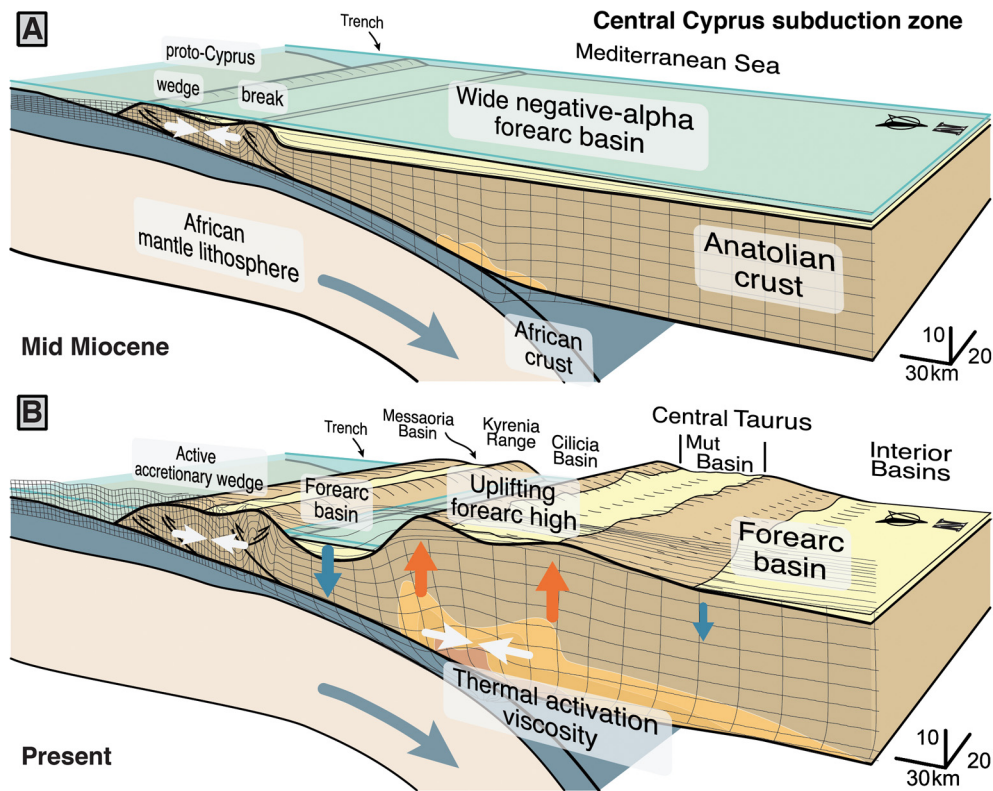
Fig. 9. Mechanism of thermo-viscous uplift. Box model representation of the mechanism of thermo-viscous forearc high uplift in two time-steps. Boxes show the evolution and forearc elements for a generic subduction wedge with forearc high (at the box model front) and for the Central Cyprus margin (at the box model back). Time steps are interpreted as representative of the Central Cyprus margin. Integrated deformation is shown using the Lagrangian mesh of the model. Note that the model is only two-dimensional.
