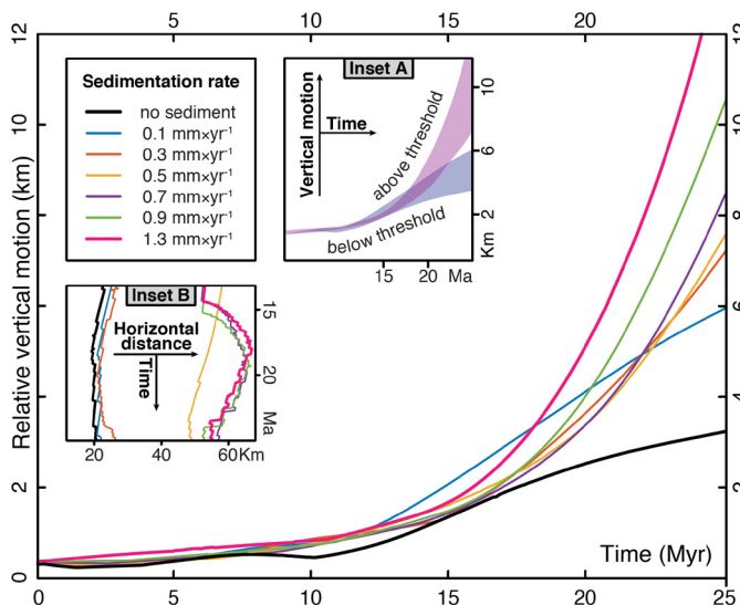
Fig. 6. Sedimentation rate influence on evolution of relative vertical motions in a forearc high. Each coloured line shows the height difference between the highest and lowest basement elevation in a 100 km strip centred around the S point. Models vary from no sedimentation (black) to a maximum rate of 1.3 mm/yr (magenta). Parameters specified are the maximum permissible sedimentation rate, but given that basins are underfilled, this rate characterizes the sedimentation rate over most of the basin. Note the nonlinearity in vertical displacement associated with different values of maximum sedimentation rate; for example, the change in vertical motions is roughly the same between 0.7 and 0.9 mm/yr that between 0.9 mm/yr and 1.3 mm/yr, even though the former sedimentation rate interval (0.2 mm/yr) doubles in the latter. Inset A is a schematic representation of vertical motions in time for the groups below and above the threshold in sedimentation rates. Inset B is the evolution in time of the horizontal distance between the highest and the lowest point in the basement surface for the last 12 Ma of model run.
