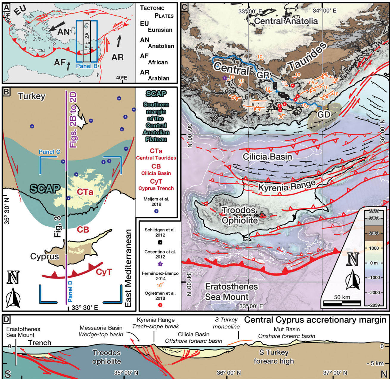
Fig. 1. Anatolian margin along the Central Cyprus subduction zone and its surrounding tectonic frame. (A) Regional map showing the motion of the African (AF), Arabian (AR) and Anatolian (AN) tectonic plates with respect to Eurasia (EU), and the location of panel B below and Fig. 2A. (B) Map of the northeast Mediterranean, showing the extent of the southern margin of the Central Anatolian Plateau (SCAP) and other key elements in the area. CTa = Central Taurides; CB = Cilicia Basin; CyT = Cyprus trench. Neogene rocks on Central Taurides and Cyprus are in yellow. Blue circles show the location of the part of the data set of Meijers et al. (2018) that falls within the map area. The location of panel C to the right and panel D below are also shown, as well as that of transects in Fig. 2B to 2D and Fig. 3. (C) Map of the Central Cyprus accretionary margin and surrounding regions. The offshore bathymetry shows shallowing in graded colours from purple to blue. Offshore structures come from Aksu et al. (2005) and Calon et al. (2005) and are classified into 4 hierarchical levels; the subduction megathrust in the south, regional structures in thick red, secondary structures in thin red and minor structures in black. The topography in the onshore, including the Central Taurides, is shown as (i) graded colours until 1.5 km, with the 1 km equal-height contour highlighted in black, (ii) in brown from 1.5 km to 2.5 km, and (iii) in grey for heights >2.5 km. Structural data from Fernández-Blanco (2014) is in orange and shows bedding dips in Late Miocene marine rocks and the S Turkey monocline delineated by them. The location of data sets of Cosentino et al. (2012), Schildgen et al. (2012) and Ögretmen et al. (2018) are shown as a purple star, black squares, and red circles, respectively. GR and GD stand for Göksu River and Göksu Delta. (D) Cross-section across the Central Cyprus accretionary margin showing the main elements along the margin and their correlation with elements of accretionary wedges. Modified from Fernández-Blanco et al. (2019). (For interpretation of the colours in the figure(s), the reader is referred to the web version of this article.)
