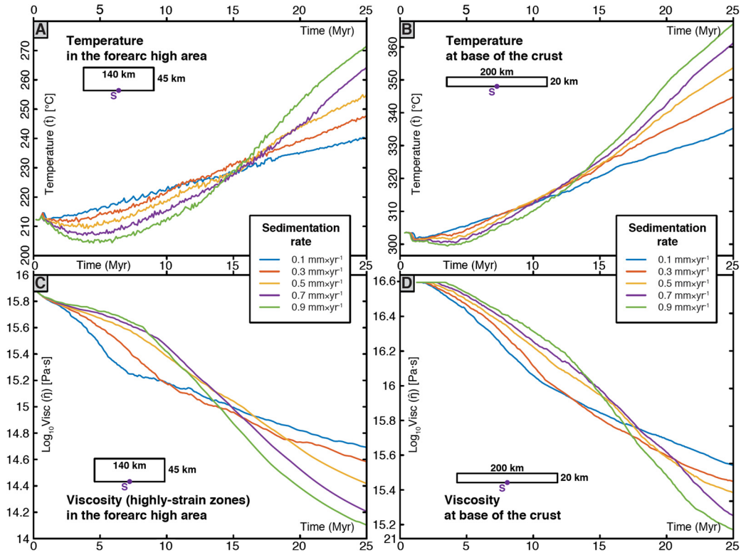
Fig. 8. Temperature and viscosity variation of the forearc high and crustal base with sediment fill level. Evolution of median ( \bar{T} ) temperature and median ( \bar{\eta} ) viscosity in the forearc high region (A; C) and base of the crust (B; D). Areas considered are centred in the S point; 140 km wide \times 45 km tall for the forearc high region and 200 km wide \times 20 km tall for the base of the crust. We assume a representative, non-parametric calculus, using the median for both temperature field and viscosity distribution. For the former, we compute median temperature values for each grid point, thereby avoiding potential complications related to multi-modal distributions in temperature fields of geodynamic models. For the latter, we compute the median viscosity of highly-strained regions. To avoid the tendency of average values to misrepresent power-law distributions, we calculate the strain rates for all grid elements and use the median viscosity of the 10% with larger strain rates. Different line colours represent the maximum sedimentation rates of 0.1 mm/yr (blue), 0.3 mm/yr (red), 0.5 mm/yr (yellow), 0.7 mm/yr (purple), and 0.9 mm/yr (green). Note the decrease in crustal viscosity due to crustal thickening, with sedimentation increasing the effect.
