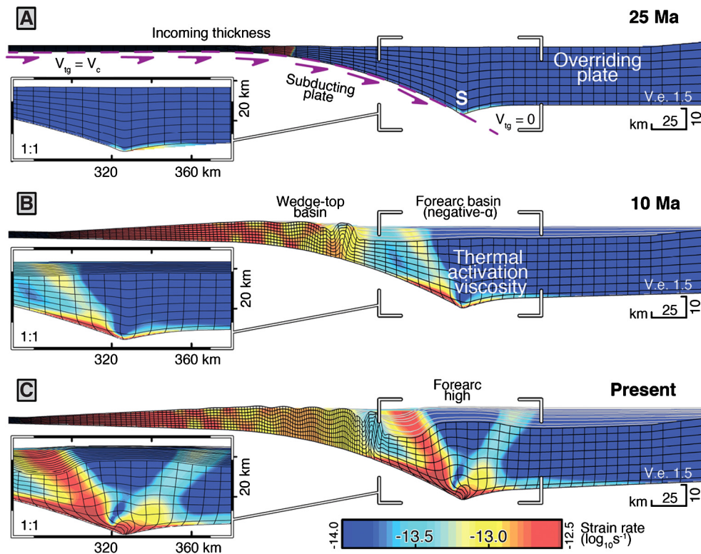
Fig. 5. Finite element models of accretion. Three time-steps (initiation at 25 Ma, 10 Ma and present) in the numerical thermo-mechanical model of viscous-plastic deformation for a convergent wedge undergoing basal traction to simulate subduction. Insets focus on the area where the forearc high develops. The colour shows the second invariant of strain rate tensor. The cumulative strain is shown by the Lagrangian mesh. Individual lines on top of the basement are isochrones (synthetic stratigraphy) originally plot horizontal (every 2.5 Ma in main plots and 1.5 Ma in insets) and later deformed with the Lagrangian mesh to reflect the overall geometric relationships. The upper panel represents a thermally stable subduction system without prior accretion or deformation. The middle panel at 10 Ma shows a wide forearc (negative-alpha) basin and a small zone of higher deformation near S point. The bottom panel at present shows a forearc high uplifted by lower crustal flow and two conjugate brittle shear zones. Note the upward motion undergone by the older stratigraphy and syn-tectonic thinning of younger layers over high. The model does not include erosion and sediments draping the forearc high are still present, but would be expected to erode quickly were this process included. See Video S2 in Supplementary Material.
