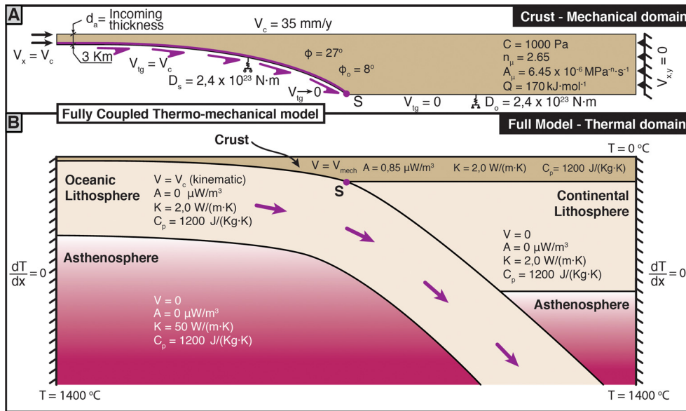
Fig. 4. Model setup, with mechanical and thermal parameters. S is the point of contact between subducting plate and upper plate Moho. V is velocity, with V_c = convergence velocity; V_{tg} = tangential velocity along the base of the mechanical model; V_x = velocity in horizontal axis; V_y = velocity in vertical axis; and V_{mech} = velocity in the mechanical domain, all defined in a reference frame fixed to the undeformed interior of the upper plate. d_a is the thickness of incoming sediments. D_s and D_o are the flexural rigidities of the subducting and overriding plates, respectively. The internal friction angle is represented by \phi , and \phi_b is the friction angle between the subducting and overriding plates. C is cohesion, A_{\mu} and n_{\mu} are the coefficient and exponent of the power-law viscosity and Q is the activation energy. A is heat production, K is the thermal conductivity, and C_p is specific heat. T stands for temperature.
