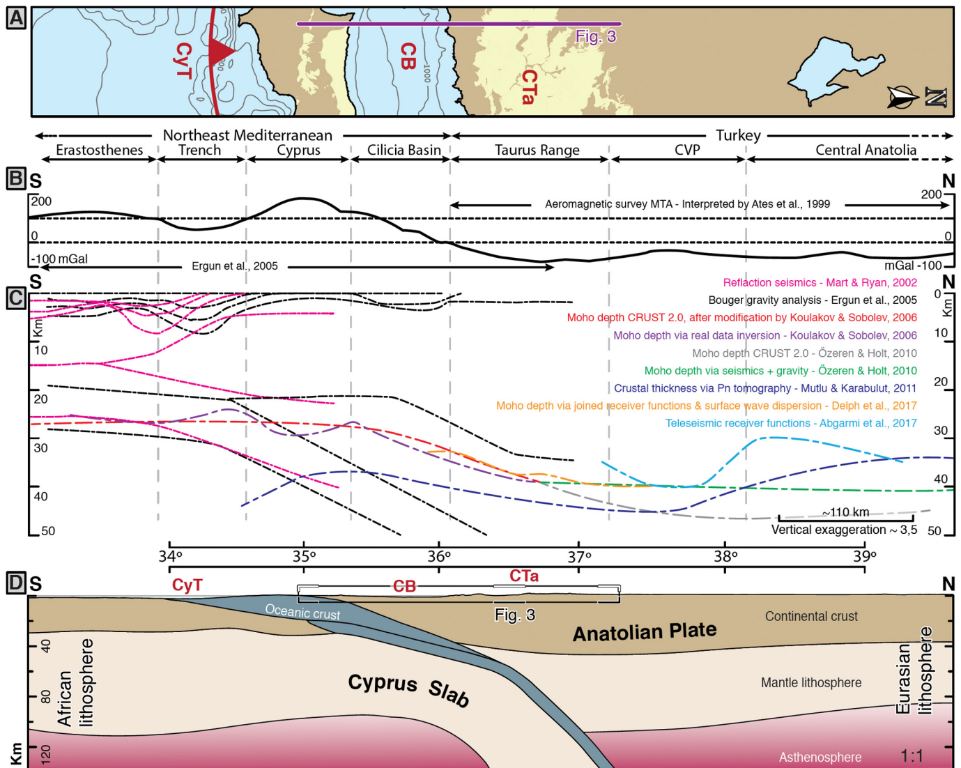
Fig. 2. Plate-scale transect along the Anatolian margin in Central Cyprus. (A) Map view of a 2°-longitude wide (32°30' E to 34°30' E) swath running ~650 km along latitude, as a reference for data along transects in panels (B) and (C). (B) Values along the section of interest derived from the two major gravimetric studies in the area (Ates et al., 1999; Ergün et al., 2005). (C) Published geophysical data, including the interpretation of the offshore section C in Ergün et al. (2005), and that of the seismic study performed by Mart and Ryan (2002). The cross-section also includes values of depth of the Moho obtained from Moho maps derived by geophysical approaches, including Pn tomography and receiver functions (Abgarni et al., 2017; Delph et al., 2017; Koulakov and Sobolev, 2006; Mutlu and Karabulut, 2011; Özeren and Holt, 2010). (D) Lithospheric-scale transect along the Central Cyprus subduction margin (for ~650 km at 33°30' E) from the interpretation of the data shown in (B) and (C).
