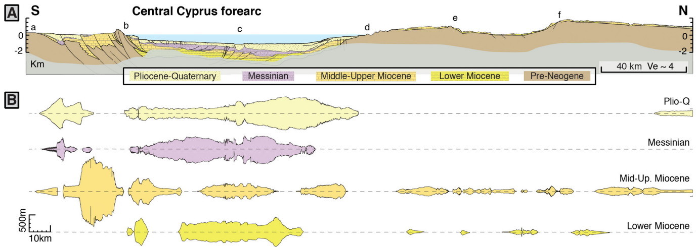
Fig. 3. Uppermost-crust transect along the Central Cyprus forearc. (A) Geologic transect along the Central Cyprus forearc (for \sim 300 km at 33^{\circ}30' E, exaggerated \sim 4 times in the vertical. Letters “a” to “f” show the approximate location of structural highs bounding basinal sectors with similar cross-sectional lengths. See main text for data used and interpretation. (B) Thicknesses of main stratigraphical units derived from the transect and their age.
