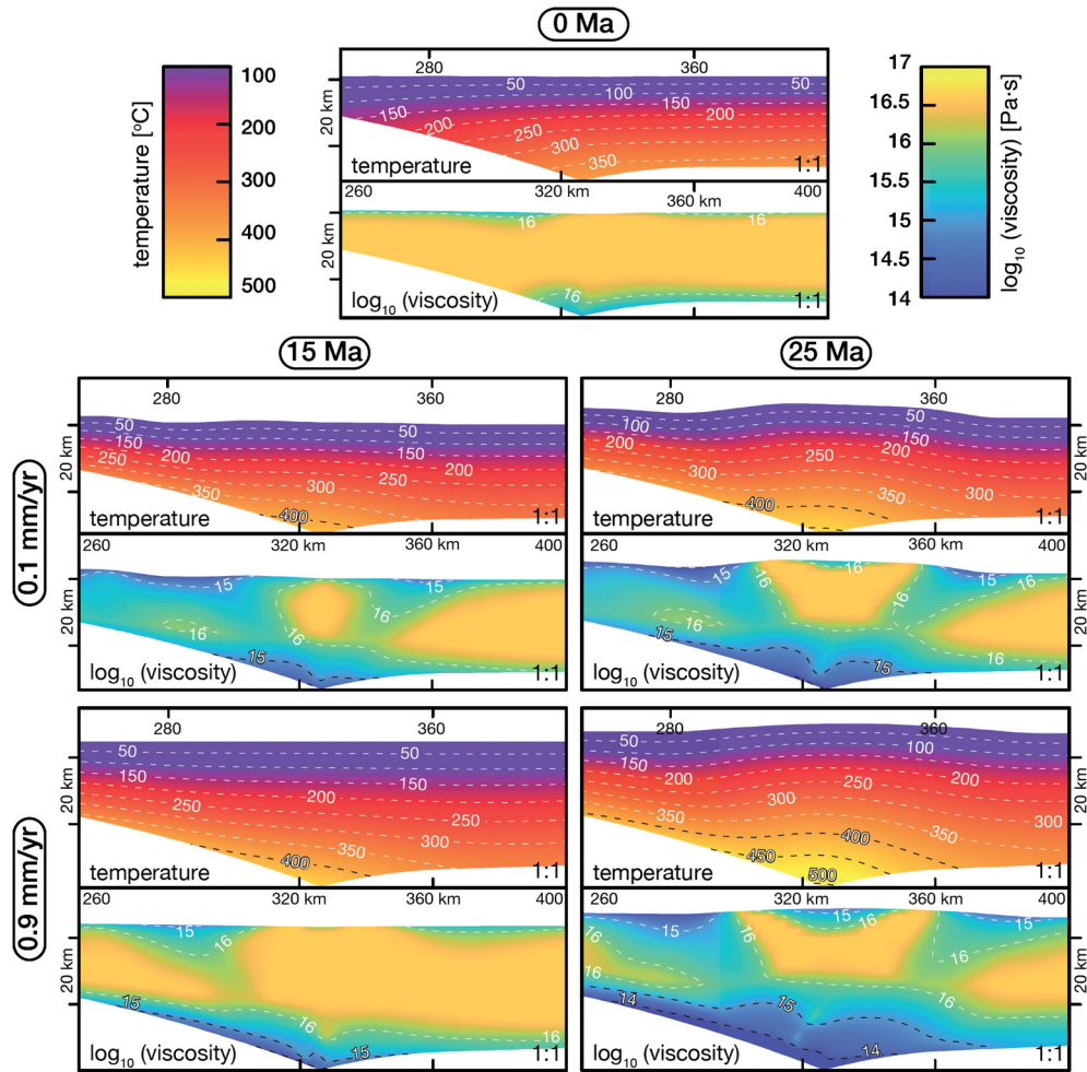
Fig. 7. Variations with sedimentation rate in the evolution of the temperature and the viscosity (in \log_{10} form) fields. Pairs of plots of temperature field (top) and viscosity field in \log_{10} form (bottom) for model onset (at the top centre), 15 Ma (left) and 25 Ma (right). For models at 15 Ma and 25 Ma, maximum sedimentation rates are 0.1 mm/yr in the upper row and 0.9 mm/yr in the bottom row. Plots represent a 140 km wide box of the model mechanical domain centred in the S point. Highlighted in black are specific contours showing the enlarged region of high temperature and low viscosity with increasing sedimentation fill level.
