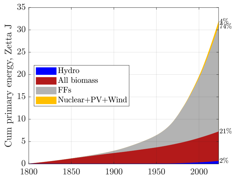
Figure 4.10: Global cumulative primary energy production by source. Please notice that in 2023, biomass and fossil fuels delivered 95% of the primary energy that drove our civilization for the last two centuries. The contribution of each energy source was rounded to an integer, and the results do not add to 100%. Sources: EIA, OWID, Clark and Jacks (2007) , Patzek, accessed 01/12/2025.
