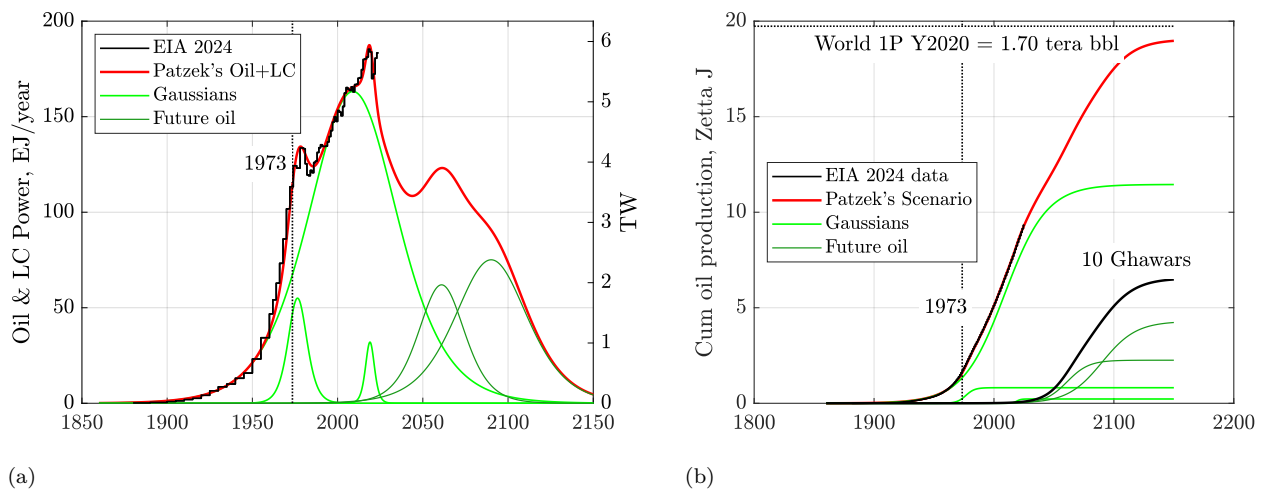
Figure 6.3: (a) The global crude oil and lease condensate power, with two very large Gaussians representing future production. (b) Cumulatively the world will produce the 2020 1P reserves or \sim 19 ZJ; 6.4 ZJ or 10 Ghawars at 100 billion bbl each will be produced in the future. Data sources: EIA, BP, OWID, and World Bank, accessed 9/15/2024; analysis by Patzek.
