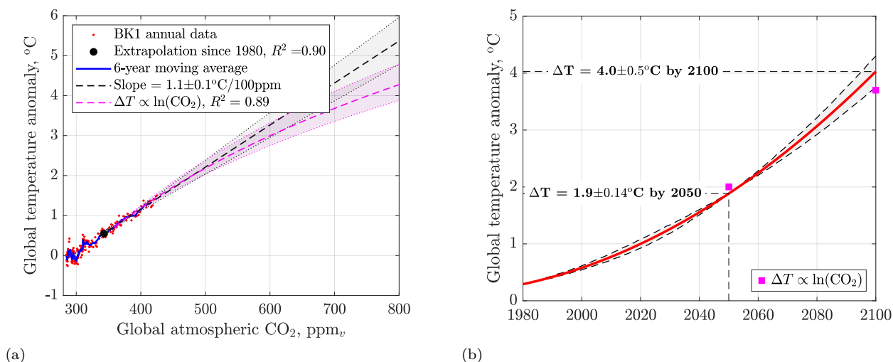
Figure 11.6: Patzek's 720 ppm v scenario. (a) Global temperature anomaly vs. \text{CO}_2 emissions, given \Delta T vs. time in Figure 10.10(b) and cumulative \text{CO}_2 emissions vs. time in Figure 5.5(b), the black parabola. (b) Global temperature anomaly vs. time, given \Delta T vs. \text{CO}_2 emissions in Figure 10.10(a) and cumulative \text{CO}_2 emissions vs. time in Figure 5.5(b). The 95% ( 2\sigma ) confidence intervals that the polynomial fits explain the data are shaded.
