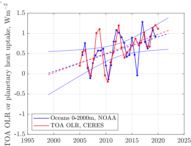
Figure 12.2: Outgoing Longwave Radiation (OLR) forcing by heated ocean water. In the last two decades, the Earth stored \Delta RF = +1 \text{ Wm}^{-2} , or half of incremental \text{CO}_2 forcing since 1750, see Figure 9.1(b). The global climate is controlled by the amount of sunlight absorbed by Earth and the amount of infrared energy emitted to space. These quantities – together with their difference – define Earth’s radiation budget (ERB). TOA OLR CERES = the Top-Of-the-Atmosphere Outgoing Longwave Radiation from the US Clouds and the Earth’s Radiant Energy System (CERES), a project that provides satellite-based observations of ERB and clouds. It uses measurements from CERES instruments flying on several satellites along with data from many other instruments to produce a comprehensive set of ERB data products for climate, weather and applied science research. The CERES instruments provide direct measurements of reflected solar radiation and emission of thermal infrared radiation to space across all wavelengths between the ultraviolet and far-infrared. Data sources: NOAA1 , NOAA2 , and NASA CERES Loeb et al. (2021) , calculations by Patzek.
