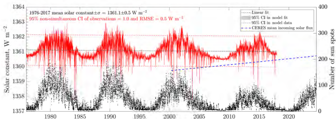
Figure 7.3: The best available reconstruction of the solar constant is based on multiple independent data sets. Over the past 42 years, the solar constant has remained remarkably stable, with a mean value of 1361.1 \pm 0.5 \text{ W m}^{-2} (1 standard deviation), varying by up to \pm 1 \text{ W m}^{-2} ( \pm 0.07\% ) in phase with the solar sunspot cycle. At top of atmosphere (TOA), Earth receives a time-averaged solar irradiance of F_{\odot}/4 = 1361.1 divided by four = 340.275 \text{ W m}^{-2} . The reduction factor of 1/4 arises from averaging the solar light incidence angles between the equator to the poles ( 1/2 ), and accounting for the Earth rotation (day-night cycle, 1/2 ). The solar constant values are derived from the supplementary data in Gueymard (2018) . CERES radiative fluxes are based on the dataset CERES_EBAF-TOA_Ed4.2_Subset_200003-202407.nc, accessed on February 1, 2025. Monthly sunspot numbers were obtained from the SILSO database at https://www.sidc.be/SILSO/datafiles . Calculations by Patzek.
