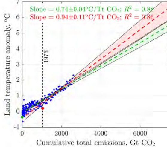
Figure 11.3: Global land temperature anomaly vs CO 2 emissions, given \Delta T vs. time in Figure 10.10(a) and cumulative CO 2 emissions vs time in Figure 5.5(b) (red curve). The 95% ( 2\sigma ) confidence intervals that the fitted curves explain the data are shaded. All data since 1850 were used in the green fit, and in the red one, only the post-1976 bifurcation data were used. Since the bifurcation was caused by land heating up over two times faster than the oceans, the slope difference is large.
