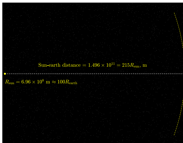
Figure 7.2: The Sun-Earth system drawn to scale. The arc on the right depicts the Earth's orbit around the Sun. At this scale the Earth is an invisible spec lost in the vast Universe. Because of its size and distance from the Sun, the Earth intercepts only one-half of one billionth of all radiation emitted by the Sun.
