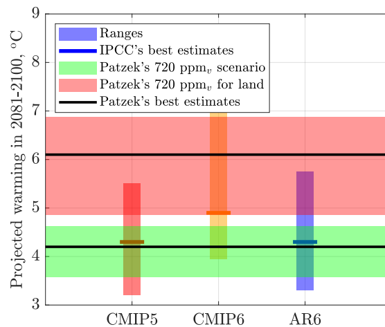
Figure 11.5: Comparison of Patzek's 720 ppm v scenario with IPCC's Sixth Assessment Report (AR6), and CMIP5 and 6. Agreement of Patzek's most probable global \Delta T with those from CMIP5 and AR6 is remarkable. The Climate Model Intercomparison Project, Phase 6 (CMIP6) consists of some 100 distinct climate models produced by 49 different modelling groups. The earlier CMIP5 protocol consisted of thirty five climate model experiments designed to (i) assess the mechanisms responsible for model differences in poorly understood feedbacks associated with the carbon cycle and with clouds, (ii) examine climate "predictability", and (iii) determine why similarly forced models produce different responses. Data source: AR6-Chapter 7 Figures, accessed 09/23/2023.
