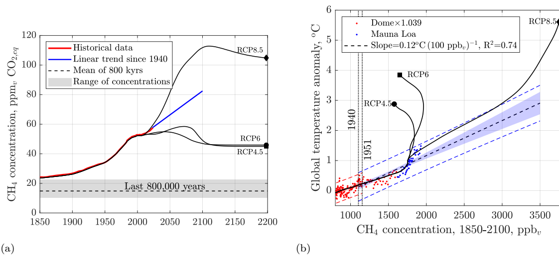
Figure 6.7: (a) Methane concentrations are converted to CO 2,eq by multiplying them by 29.8 (Arias et al. , 2021). Historic CH 4 concentrations are obtained from EPICA Dome C core data multiplied by 1.039 to align the overlapping data points with the Mauna Loa data. Very uncertain future concentrations are predicted by an extrapolation of the linear fit of historic data between 1940 and 2024. Three RCP scenarios are shown for calibration. (b) Global mean annual temperature anomaly vs CH 4 concentration. The plotted RCP scenarios (Meinshausen et al. , 2011) were converted to the corresponding temperature anomalies by multiplying their respective CTE by the average slope of 0.62 °C (Tt CO 2 ) -1 in Figure 5.7(c). This calculation is well within the range of global warming probability distributions for RCP4.5, 6 and 8.5 (Sherwood et al. , 2020, Fig. 23). Notice that the RCP8.5 trajectory tracks historical data best, but I am quite unsure how predictive its future outcomes are. Data sources: Supplementary materials to MacFarling Meure et al. (2006), PAGES (2016), Mauna Loa (Lan et al. , 2025b). Calculations by Patzek.
