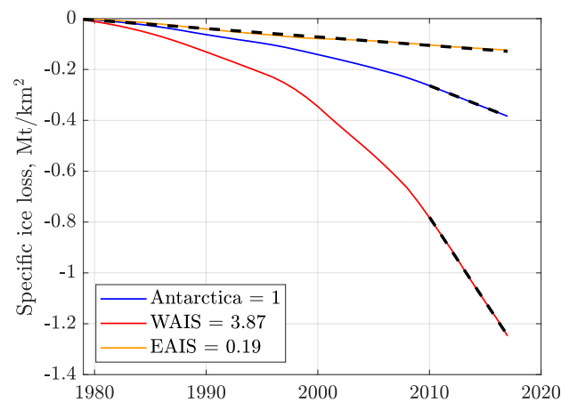
Figure 12.5: The slopes of the dashed lines are the specific rates of ice loss in \text{Mt} (\text{yr km}^2)^{-1} between 2010 and 2017. The West Antarctic Ice Sheet (WAIS) lost ice at the rate four times higher than Antarctica, while the East Antarctic Ice Sheet (EAIS) lost ice at the rate five times lower. Data source: Supplementary data set pnas.1812883116.sd01.xlsx to Rignot et al. (2019) , accessed on 01/06/2024, calculations by Patzek.
