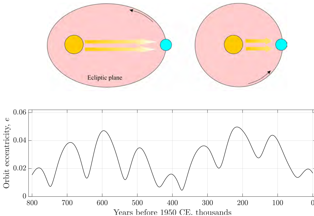
Figure 9.2: The MILANKOVITCH eccentricity cycle has three periods of roughly 405,000 yrs, 95,000 years and 124,000 years, with a beat period of 400,000 years. They loosely combine into a 100,000-year cycle. The present eccentricity is 0.0167 and decreasing. The Earth's orbit plane ( ecliptic ) also precesses (wobbles) with a period of 112 ky due to interactions with Jupiter and Saturn. We call this wobbling apsidal precession. Eccentricity refers to the shape of Earth's orbit around the Sun, varying from near circular ( e = 0.0034 ) to slightly elliptical ( e = 0.058 ). When Earth's orbit is at its most elliptic, about 23% more incoming solar radiation reaches Earth at perihelion than at aphelion. Currently, Earth's orbit eccentricity is very slowly decreasing.
