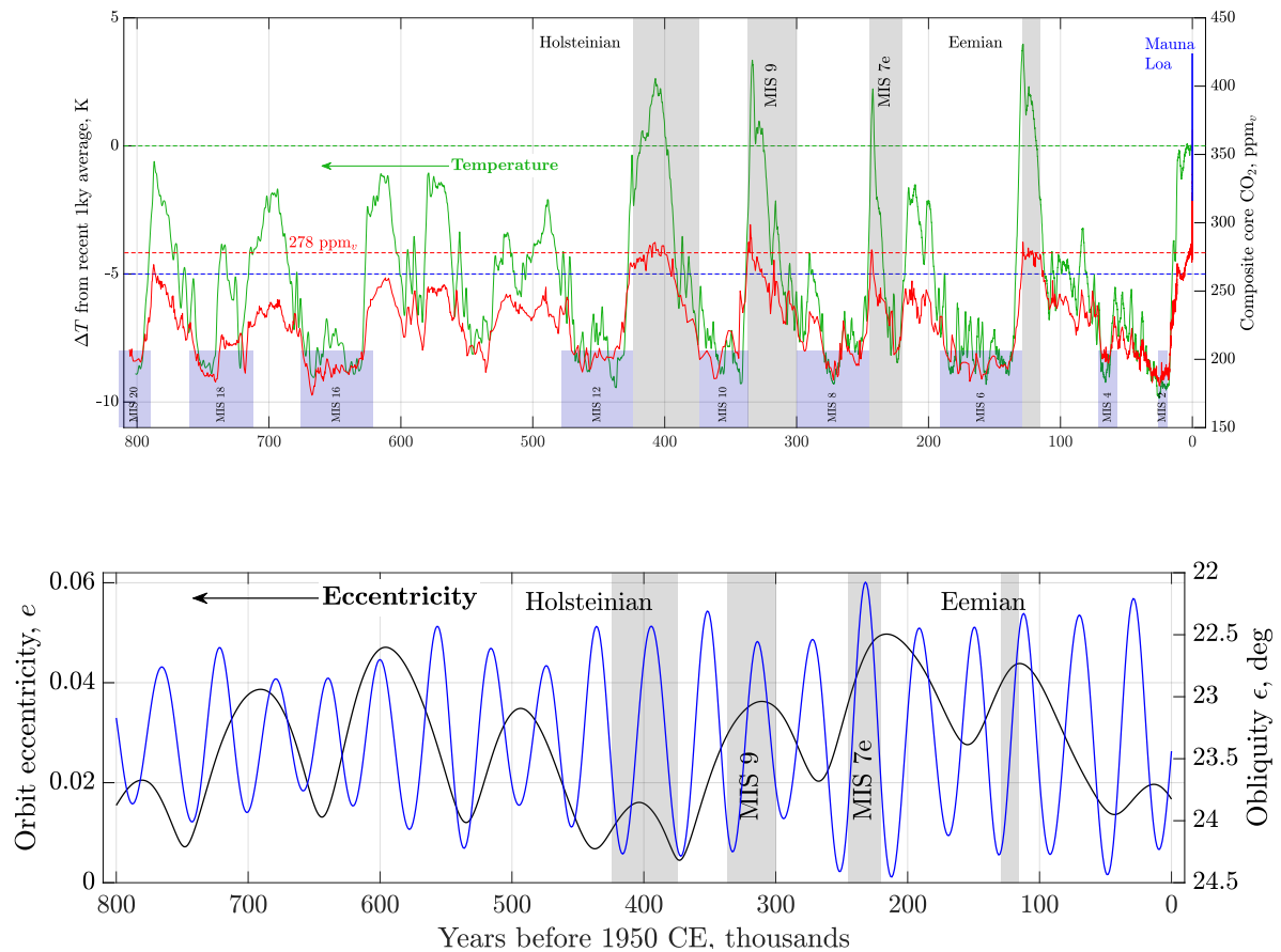
Figure 9.5: Sensitivity of paleoclimate over the last 800,000 years to pCO 2 ( top ) and the Milankovitch cycle forcing ( bottom ). It seems that the interglacial periods were driven usually by high orbit ellipticity (eccentricity), but not the Holsteinian, and low axis tilt (obliquity). When Earth's orbit is at its most elliptic, about 23 percent more incoming solar radiation reaches Earth each year at perihelion than does at its aphelion. The glaciation cycles were driven by low eccentricity. When eccentricity is low the glaciations become less extreme and more stable. Notice that the orbit eccentricity has a period of ~100 kyrs and the beat period (waveform repeats) of 400 kyrs. Data source: Supplementary materials to MacFarling Meure et al. (2006) , PAGES (2016) , NOAA Bereiter et al. (2015b) , Lan et al. (2025a) , calculations by Patzek, 12/30/2023.
