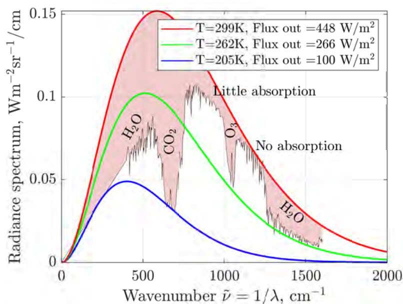
Figure 7.8: The energy-density spectrum of outgoing thermal radiation from the Earth at wave numbers ranging from 400 to 1600 cm -1 (black jagged curve). Equivalent wavelengths of 6.3-25 microns are in the mid- and far-infrared bands (see Definition 12 ). The pink area is due to net absorption of the outgoing energy flux by greenhouse gases that block parts of the Planck blackbody radiation of ground surface at the temperature of 299 K. These spectral radiance data were measured on May 5, 1970, 12:00:07 with NASA's IRIS instrument on the Nimbus 4 satellite. Here you can see one of the earliest satellite measurements of Earth's outgoing longwave radiation that have since become critical to monitoring our planet's energy balance. Data source: NASA. Calculations by Patzek.
