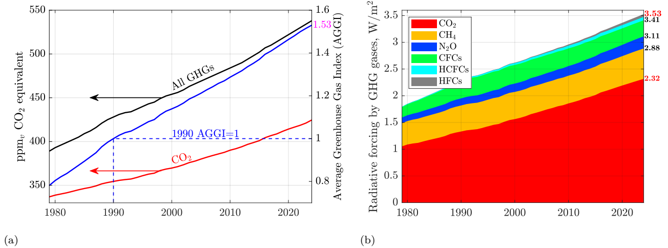
Figure 7.9: (a) Accumulation of CO 2 and all GHG gases in the atmosphere (left y -axis) and the NOAA Annual Greenhouse Gas Index (AGGI), normalized to the year 1990 (right y -axis). (b) Radiative forcing, relative to 1750, of virtually all long-lived greenhouse gases. Data sources: ( Dlugokencky et al. , 2025), see the caption of NOAA’s Figure 3 for the list of key GHGs. Calculations by Patzek.
