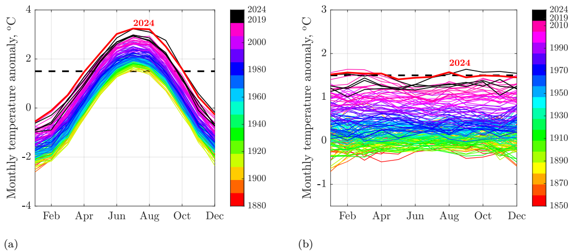
Figure 10.11: Stacked global temperatures colored by decade. The years 2020-2023 are shown in black and the record-breaking 2024 is a thick red curve. The thick horizontal dashed line is the +1.5°C temperature anomaly. (a) Seasonal temperatures of both hemispheres. (b) The stacked monthly global temperatures eerily resemble increasing water level in a tub filling with water that is warming most of the time. The almost horizontal water surface in this analogy has been controlled by clouds that make the Earth's albedo uniform. Data sources: NASA GISTEMP ( NASA, 2015 ) and Berkeley Earth, accessed 2/10/2025. Calculations by Patzek.
