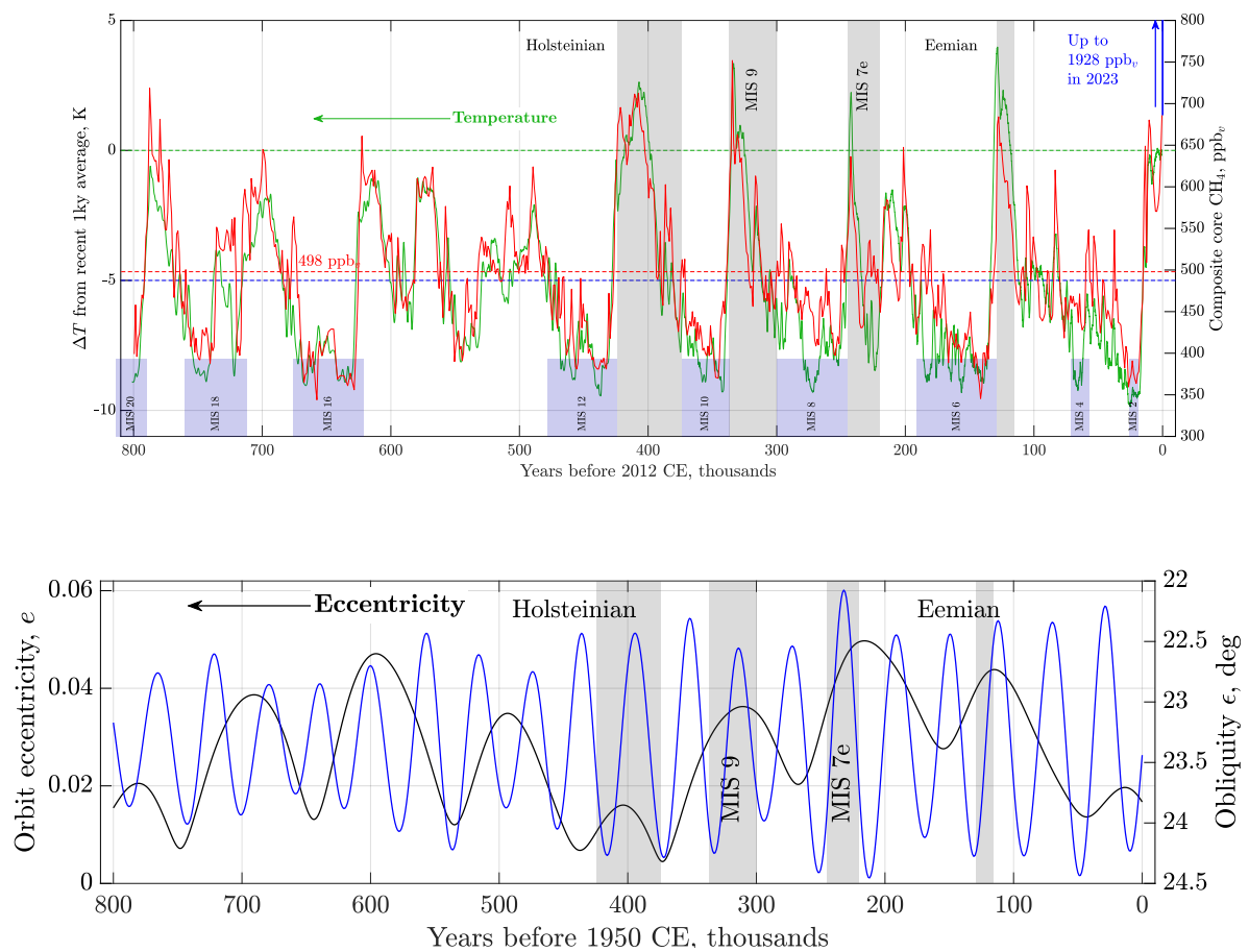
Figure 9.6: Sensitivity of paleoclimate over the last 800,000 years to ppb v of \text{CH}_4 ( top ) and the Milankovitch cycle forcing ( bottom ). Notice that current \text{CH}_4 concentration is so high that it exceeds the scale of the plot 2.5 times (if plotted, [\text{CH}_4] would extend beyond the top of this page). Data source: NOAA Bereiter et al. (2015b) , calculations by Patzek, 12/30/2023.
