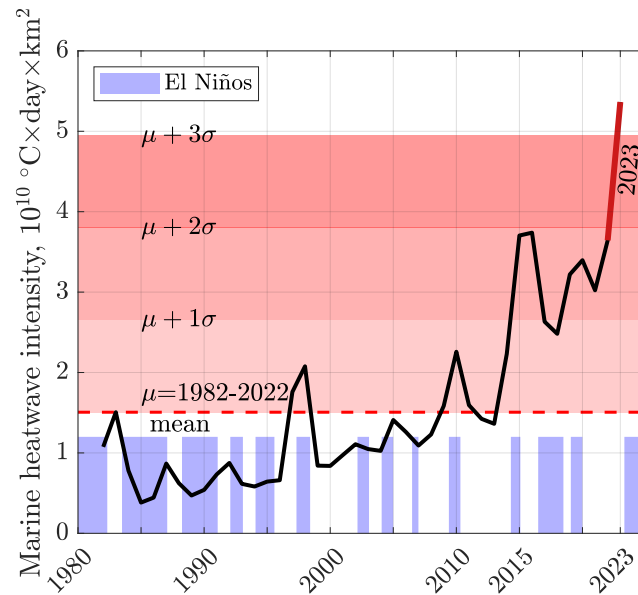
Figure 10.2: Extreme marine heatwave since 1981. Their intensity was quantified as the product of area-weighted average seawater surface temperature in ^{\circ}\text{C} from satellite images \times heatwave duration in days \times the heated area above a threshold temperature in \text{km}^2 . Note a mild positive correlation with El Niños. Plotted by Patzek, using the data to Fig1a from the Supporting Online information to Dong et al. (2025) , accessed 07/30/2025.
