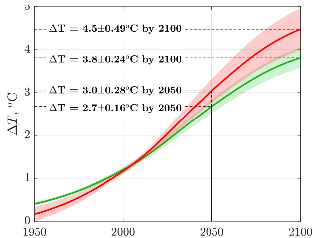
Figure 11.4: Global land temperature anomaly vs. time, given \Delta T vs. CO 2 emissions in Figure 11.3 and cumulative CO 2 emissions vs time in Figure 5.5. The 95% ( 2\sigma ) confidence intervals that the fitted curves explain the data are shaded. The land temperature data have a higher variance than global temperatures, and their 2\sigma intervals are wider.
