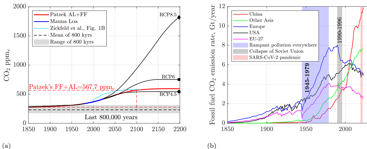
Figure 6.6: (a) Comparison of atmospheric pCO 2 until 2200, resulting from Patzek's FF+AL scenario and RCP 4.5, 6.0 and 8.5 scenarios ( Meinshausen et al., 2011 ). The Zickfeld et al. simulation curve is also displayed for comparison, showing that equal cumulative CO 2 emissions lead to equal pCO 2 s. (b) CO 2 FF emission rates by region or country. Europe includes the former Soviet Union and Warsaw Pact countries. Sources: EIA, NOAA, OWID, Clark and Jacks (2007) , Patzek, accessed 02/11/2025. Calculations by Patzek.
