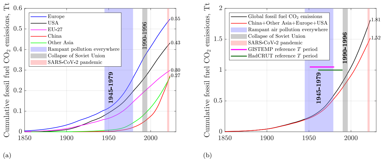
Figure 8.1: Cumulative fossil fuel CO 2 emissions by (a) country and region, and for the world and high-emitters (b). Sources: EIA, OWID, Clark and Jacks (2007) , Patzek, accessed 01/11/2024.
