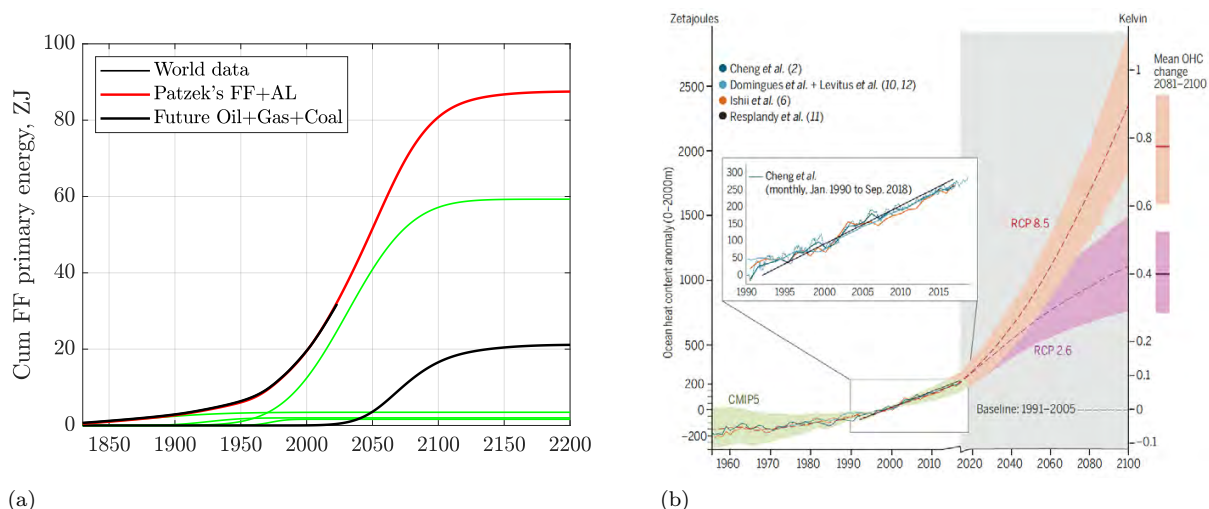
Figure 6.5: (a) Cumulative heat generated by FF fuels until 2200. Roughly 30% of these 88 ZJ of heat is converted to work and the remaining 62 ZJ is heat generated at the Earth's surface. (b) Cumulative heat from incremental radiation forcing by GHGs. Ocean water heat content 0–2000 m depth is likely to reach 1500 ZJ by 2100. Image source: Cheng et al. (2017) . Data sources: EIA, BP, OWID, and World Bank, accessed 9/15/2024; analysis by Patzek.
