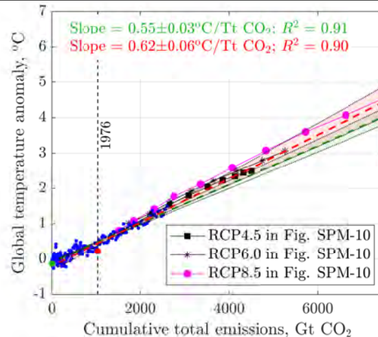
Figure 11.1: Global temperature anomaly vs \text{CO}_2 emissions, given \Delta T vs. time in Figure 10.10(b) and cumulative \text{CO}_2 emissions vs time in Figure 5.5(b) (red curve). The 95% ( 2\sigma ) confidence intervals that the fitted lines explain the data are shaded. The red color and dot signify the post-bifurcation fit, 1976-2023, and the green color signifies the 1850-2023 fit.
