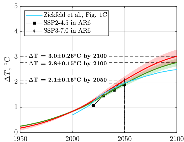
Figure 11.2: Global temperature anomaly vs time, given \Delta T vs. \text{CO}_2 emissions in Figure 11.1 and cumulative \text{CO}_2 emissions vs time in Figure 5.5(b) (red curve). The 95% ( 2\sigma ) confidence intervals that fitted curves explain the data are shaded. The Zickfeld et al.'s data fall below our prediction because their CTE was \sim 2 Tt of \text{CO}_2 less than that in the 528 \text{ppm}_v scenario, cf. Figure 5.5(b).
