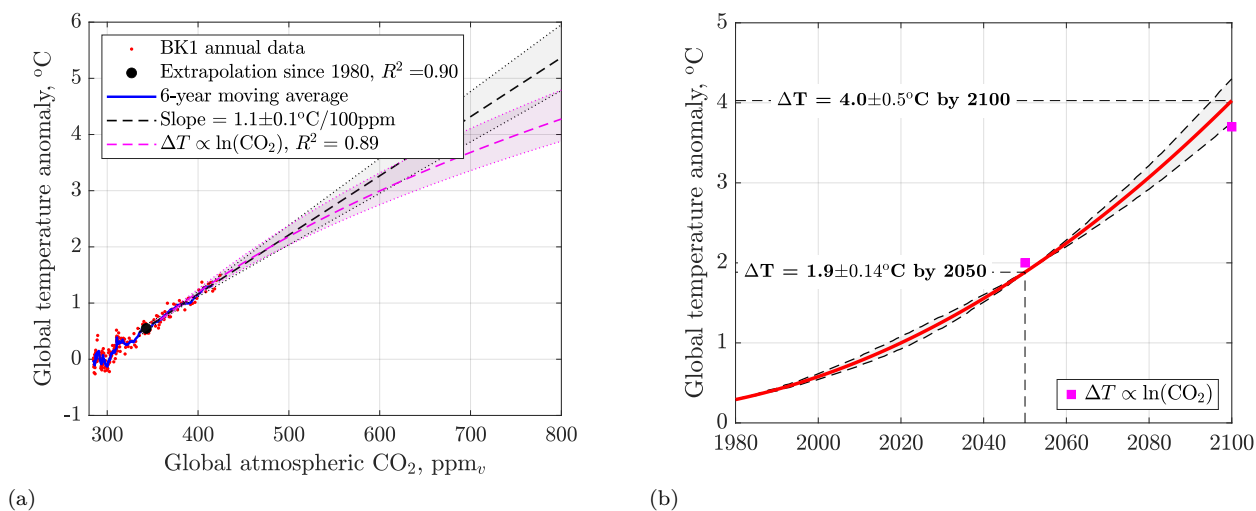
Figure 11.6: Patzek's 720 \text{ppm}_v scenario. (a) Global temperature anomaly vs. \text{CO}_2 emissions, given \Delta T vs. time in Figure 10.10(b) and cumulative \text{CO}_2 emissions vs. time in Figure 5.5(b), the black parabola. (b) Global temperature anomaly vs. time, given \Delta T vs. \text{CO}_2 emissions in Figure 10.10(a) and cumulative \text{CO}_2 emissions vs. time in Figure 5.5(b). The 95% ( 2\sigma ) confidence intervals that the polynomial fits explain the data are shaded.
