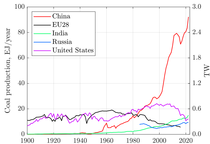
Figure 7.4: Coal production by country expressed in common energy units, because different coals have different heating values per unit mass and densities. Notice that China produces over five times more coal than any of the countries and entities in the plot. In fact, China has exceeded our own prediction of their peak coal production in \sim 2011 ( Patzek and Croft, 2010 ), remembering that truthfulness of Chinese coal production data reporting was questionable at times. Sometimes, the overburden rock would pass as coal. In 2022, China permitted more coal power plants than any other time in the last seven years, according to a new report released this week. “It’s the equivalent of about two new coal power plants per week . The report by energy data organizations, Global Energy Monitor and the Centre for Research on Energy and Clean Air, finds the country quadrupled the amount of new coal power approvals in 2022 compared to 2021.” Data sources: Energy Institute Statistical Review of World Energy ( Anonymous, 2023b ), ( Anonymous, 2023a ), and NPR .
