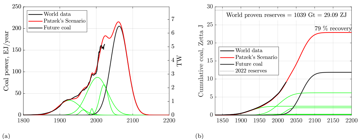
Figure 8.2: (a) Patzek's scenario of future coal production rate. The Gaussian representing future coal production is the largest ever. (b) Patzek's scenario of cumulative coal production predicts that 79% of global coal reserves will be produced. Data sources: EIA, BP, OWID, accessed 08/30/2024; analysis by Patzek.
