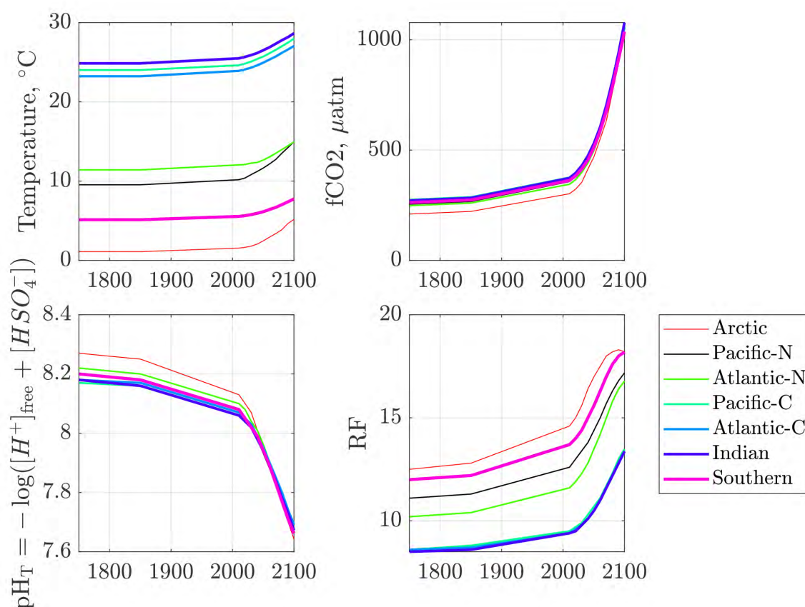
Figure 5.9: The key parameters characterizing the chemistry of surface seawater are shown. Note the abrupt changes in all of them after 2010. These trends reflect the accelerating global ocean warming and acidification driven by the rising atmospheric \text{CO}_2 concentration. Data source: NOAA, https://www.ncei.noaa.gov/data/oceans/ncei/ocads/data/0259391/ .
