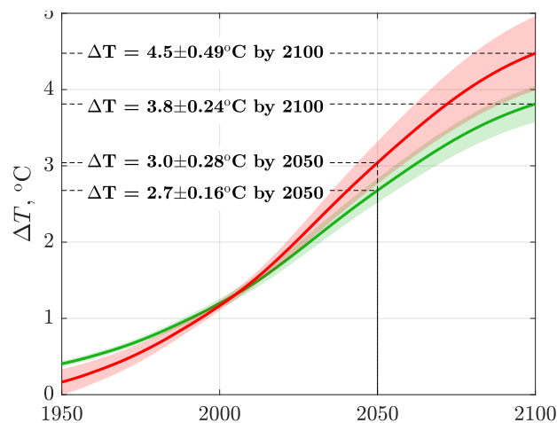
Figure 13.4: Global land temperature anomaly vs. time, given \Delta T vs. \text{CO}_2 emissions in Figure 13.3 and cumulative \text{CO}_2 emissions vs time in Figure 7.5. The 95% ( 2\sigma ) confidence intervals that the fitted curves explain the data are shaded. The land temperature data have a higher variance than global temperatures, and their 2\sigma intervals are wider.
