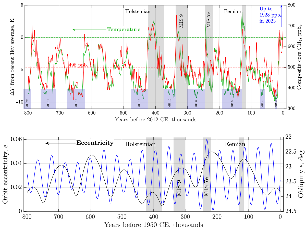
Figure 11.6: Sensitivity of paleoclimate over the last 800,000 years to ppb v of \text{CH}_4 ( top ) and the Milankovitch cycle forcing ( bottom ). Notice that current \text{CH}_4 concentration is so high that it exceeds the scale of the plot 2.5 times (if plotted, [\text{CH}_4] would extend to the middle of the previous page). Data source: NOAA Bereiter et al. (2015b) , calculations by Patzek, 12/30/2023.
