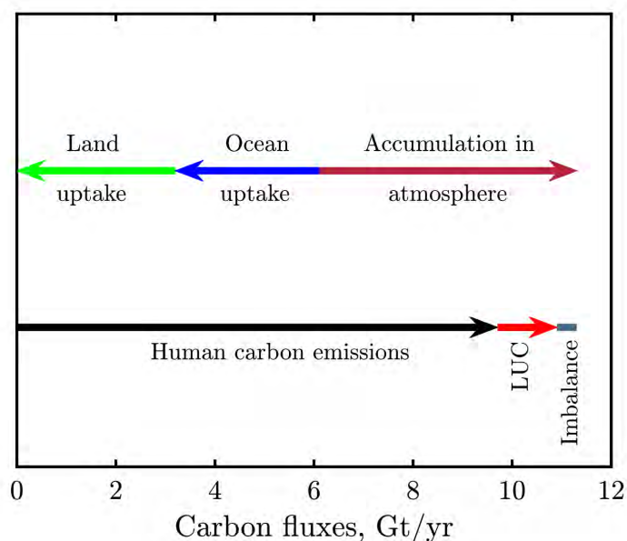
Figure 5.7: These fast-changing fluxes in the global carbon cycle matter most for climate change on an annual basis. LUC = Land Use Change. Other parts of the cycle are likely to adjust over decades, centuries and millennia. The annual accumulation in the atmosphere is roughly 5 Gt of C or 18 Gt CO 2 . To absorb this accumulation, we would need 550,000 giant direct air capture machines like the one depicted in Figure 16.5 . Data source ( Friedlingstein et al., 2025 ).
