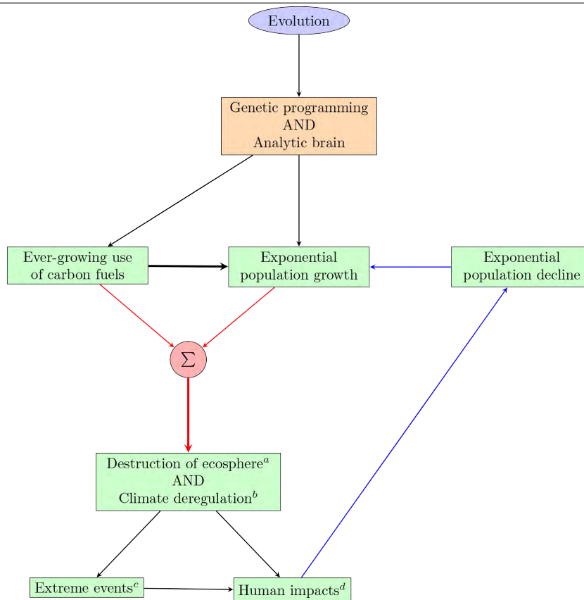
Figure 1.2: The story of human evolution and impacts on Earth is sketched by this flowchart and unfolds throughout this book. a Destruction of the ecosphere refers to ecological overshoot by humans, including ocean acidification, loss of biodiversity, wetland degradation, soil depletion, resource exhaustion, and the pervasive pollution of air, water, and land. b Climate breakdown denotes the intensifying thermal imbalance caused by greenhouse gas emissions – including the bifurcation of land and ocean warming, destabilization of the atmosphere, disruption of the water cycle, and weakening of major oceanic currents. c Extreme events encompass heatwaves, super-droughts, megafires, rain bombs and atmospheric rivers, hurricanes, tornadoes, and the collapse of ice sheets and glaciers. d Human impacts are – among others – air, soil, and water pollution; plastic saturation; freshwater scarcity; crop failures; forest collapse; rising epidemics and pandemics; increasing mortality and morbidity; hunger & starvation; mass migration (possibly 1-3 billion people); conflicts and wars; declining sperm counts; and the spread of invasive species.
