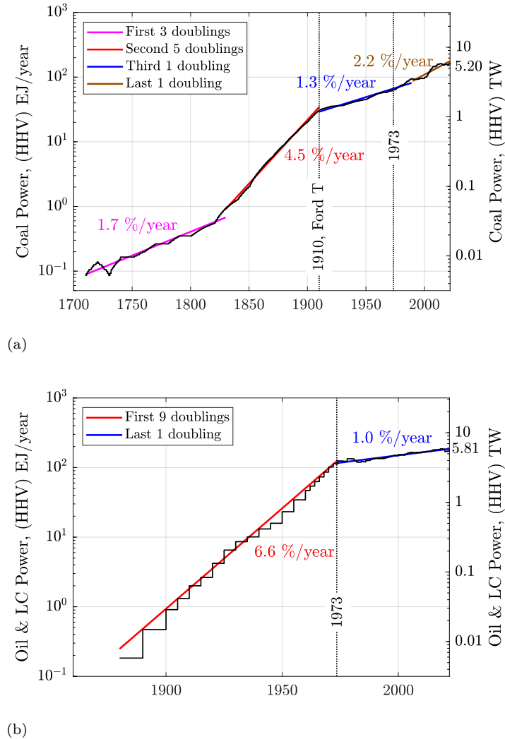
Figure 6.10: (a) The global rate of coal production underwent 10 doublings between 1710 and 2023, reaching 5.20 TW. The Ford Model T was introduced in 1908, but true mass production began with the adoption of the moving assembly line in 1913 and was fully established by 1914 (Ford, 1913), just before WWI. In 1919, a few months after the Armistice (11/11/1918 at 11 am), Citroën became the first European carmaker to implement Ford-style mass production (Citroën, 1921). During WWI, trucks, tanks and planes became common, and the rate of expansion of coal production decreased. (b) The global rate of oil and lease condensate production also underwent 10 doublings between 1880 and 2023, reaching 5.81 TW. Note that following the peak in U.S. oil and gas production in 1971–1972, the large-scale deployment of peripheral waterfloods in Middle Eastern fields over subsequent years, and the Arab oil embargo of 1973, the exponential growth rate of global oil production declined permanently by roughly a factor of six. This rate was close to zero in 2025. Sources: EIA, OWID, Clark and Jacks (2007), Patzek, accessed 11/11/2024.
