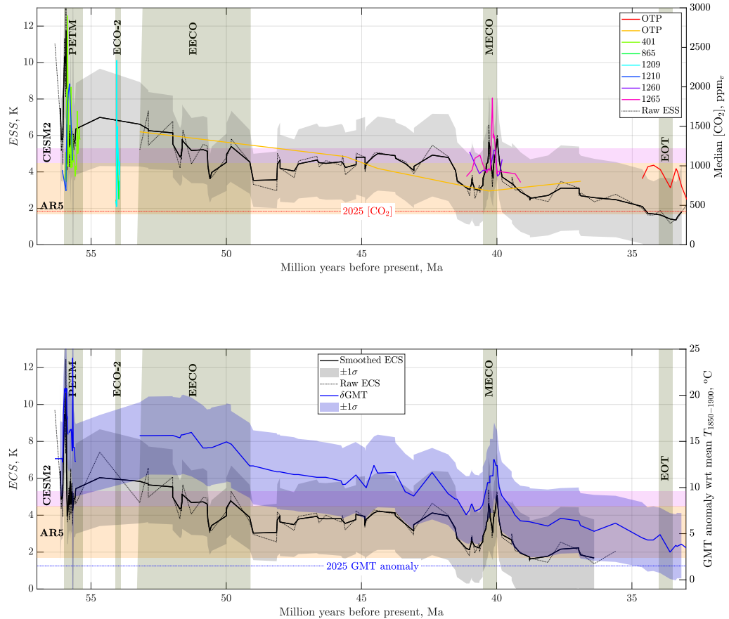
Figure 11.8: The shaded geologic periods from left to right are: PETM = Paleocene-Eocene Thermal Maximum, ECO-2 = Eocene Climatic Optimum 2, EECO = Early-Eocene Climatic Optimum, MECO = Middle-Eocene Climatic Optimum, EOT = Eocene-Oligocene Transition, during which the permanent Antarctic ice-sheets appeared. (top) ESS (see Table 9.3 for definitions), 4-point running average and raw data (left y -axis black) and median CO 2 concentrations in the atmosphere (color curves, with sources explained in the legend, right y -axis). (bottom) ECS, 4-point running average and raw data (in black, the left y -axis) and Global Mean Temperature (GMT) anomaly relative to the 1850-1900 GMT = 13.7°C IPCC, Full Report (2022) (the right y -axis). The orange rectangle denotes approximate range of ESS and ECS from Stocker et al. (2013) . The magenta rectangle reflects the high-sensitivity CESM-2 simulations Gettelman et al. (2019) . Data source: Supporting data to Anagnostou et al. (2020) , calculations by Patzek, 02/22/2025.
