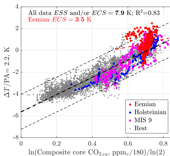
Figure 11.7: This regression shows clearly that most of the time climate during the last 800 kyrs was more sensitive to GHG forcing than today. The earth system or equilibrium climate sensitivities ( ESS or ECS ) defined in Section 9.11, see Table 9.4, to a very slow doubling of [\text{CO}_2] + 29.8[\text{CH}_4] = [\text{CO}_{2,eq}] for all data and the Eemian (MIS5e) data are plotted above. The warm Eemian climate response ( ESS = 3.5 K) is comparable to today's climate, but the slope of all ice core data from the last 800 kyrs yields ESS = 7.9 K, much higher than today and comparable to the incongruent climates during LGM (cf. Section 11.4.1) and Eocene, see Figures 11.8 to 11.9. All temperature data from the cores were divided by the Polar Amplification (PA) factor of 2.2 (Jouzel et al. , 2007a).
