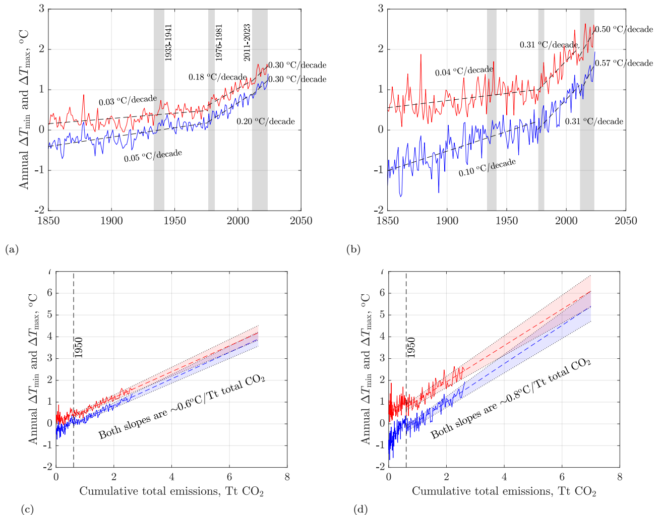
Figure 12.13: The annual maximum (red) and minimum (blue) temperatures between the years 1850 and 2024. Notice that both linear trends have been increasing slowly, with a significant break in the slope around 1976, after which the hottest temperatures have increased at 2.6^{\circ}\text{C}/\text{century} and the coldest ones have increased at 2.9^{\circ}\text{C}/\text{century} for the Earth (a), and at 3.1^{\circ}\text{C}/\text{century} for the land (b). The slopes of the warmest temperatures may have increased again in 2011 to 3.2^{\circ}\text{C}/\text{century} (!) for the global land and 5.3^{\circ}\text{C}/\text{century} (!) for the land. The slopes of the coldest temperatures jumped in 2011 to 2.4^{\circ}\text{C}/\text{century} for the Earth and 4.5^{\circ}\text{C}/\text{century} for the land. This means that winters and nights have been heating up faster during winters and nights, denying people rest and regeneration in most parts of the world. For example, soon majority of people will not be able to survive without AC year-long in most parts of the Middle East. In sub-Saharan Africa, India, Pakistan and Bangladesh, \sim 1 billion people will have no access to AC and will be increasingly dying from severe heat exposure and strokes. (c) and (d) same as (a) and (b) but plotted vs. cumulative CO 2 emissions.
