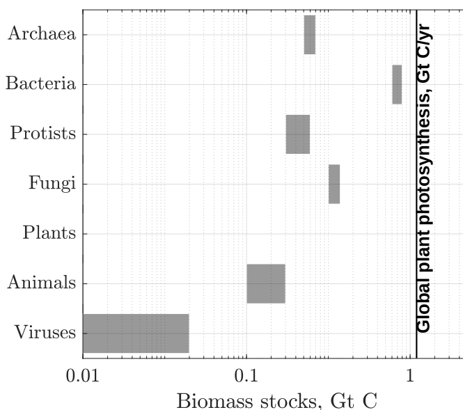
Figure 3.6: Biomass distribution by major domains and kingdoms, based on the data in Table 3.2 . Note that plants dominate so much, that the plot scale must be semi-logarithmic to visualize the other stocks of biomass. In general, biogeochemical visibility and impact are decoupled from mass.
