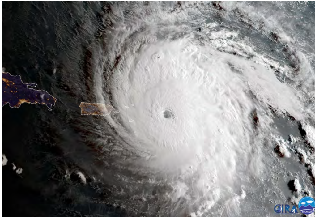
Figure 5.2: One of the strongest hurricanes ever recorded, Irma (6 September 2017), spanned an area comparable to that of France (effective radius of tropical-storm force winds = \sim 240 km)—the strongest on record remains Patricia (2015). Irma formed on August 30 and dissipated on September 13, 2017, making it a very long-lasting hurricane. At peak intensity and because of her large size, Irma ’s instantaneous power output was estimated to be nearly four times greater than the total primary power consumption of the global human economy at that time. Irma swept east-west damaging Cape Verde, the Leeward Islands (Barbuda, Saint Barthélemy, Anguilla, Saint Martin and the Virgin Islands), Greater Antilles (Cuba and Puerto Rico (intercepting the hurricane in the picture), Turks and Caicos Islands, Jamaica, The Bahamas, and Eastern United States (mostly Florida). Image source: NASA.
