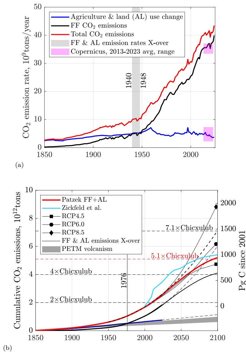
Figure 7.5: (a) CO 2 emissions rate from agriculture and land use change (AL) and fossil fuels (FF) since 1850. Notice that the substantial AL emissions rate is almost constant and provides the background CO 2 level in the atmosphere. (b) Cumulative CO 2 emissions from agriculture and land use change and fossil fuels since 1850. The Paleocene-Eocene Thermal Maximum (PETM) emissions range from 0.625 to 1 Tt C (kyr) -1 . The extrapolation of FF emissions is either quadratic (the black dashed line “720 ppm v scenario”), or it follows from our FF production model (the red “Patzek’s 562 ppm v scenario” both explained in Chapter 8). Notice that up to the year 2050, the red curve’s trajectory is very close to the representative Concentration Pathway RCP4.5 (Meinshausen et al., 2011) (black square), while RCP6.0 shoots up after 2060 (black circle). The most aggressive emissions scenario in Fig. 1 in Zickfeld et al. (2009) (blue curve) is far ahead of Patzek’s scenario, despite similar cumulative total emissions of ~1000 Pg C since 2001. Data sources: (Anonymous, 2023a) and Copernicus (Friedlingstein et al., 2023). Calculations by Patzek.
