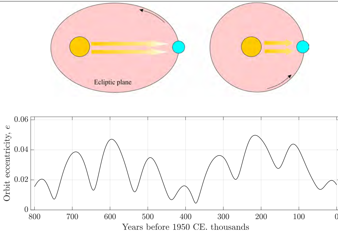
Figure 11.2: The MILANKOVITCH eccentricity cycle has three periods of roughly 405,000 yrs, 95,000 years and 124,000 years, with a beat period (repeat of wave shape) of 400,000 years. They loosely combine into a 100,000-year cycle. The present eccentricity is 0.0167 and decreasing. The Earth's orbit plane ( ecliptic ) also precesses (wobbles) with a period of 112 ky due to interactions with Jupiter and Saturn. We call this wobbling apsidal precession. Eccentricity refers to the shape of Earth's orbit around the Sun, varying from near circular ( e = 0.0034 ) to slightly elliptical ( e = 0.058 ). When Earth's orbit is at its most elliptical, about 23% more incoming solar radiation reaches Earth at perihelion than at aphelion. Currently, Earth's orbit eccentricity is very slowly decreasing.
