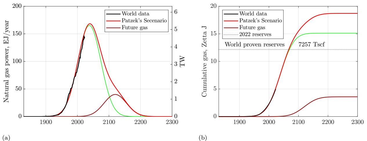
Figure 8.4: (a) The historic rate of global gas production is represented with one green Gaussian, whose unknown height is set to exceed the proven 2022 gas reserves by 35%. The future production is also represented with a single Gaussian. (b) Cumulatively the world might produce 19 ZJ as the HHV of natural gas, including 3.6 ZJ from the future projects. Data sources: EIA, BP, OWID, and World Bank, accessed 9/15/2024; analysis by Patzek.
