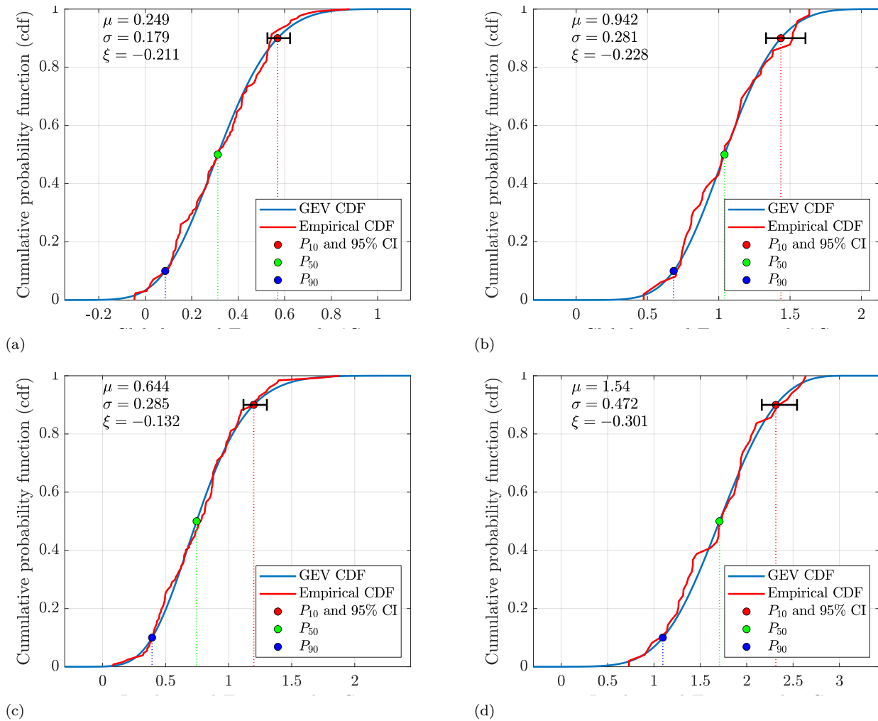
Figure 12.14: Theoretical and empirical (data-driven) GEV cumulative probability distribution functions (CDF) with the highlighted median value ( P_{50} ), and P_{90} (90% of the CDF values \geq P_{90} ) and P_{10} (10% of CDF values \geq P_{10} ). The bar around each P_{10} is the 95% confidence interval (CI). Notice that this interval is obtained from two minimizations of the function R_{10} subject to nonlinear constraints. The first minimization finds the maximum lower bound on CI, and the second one minimizes -R_{10} to find the minimum upper bound. Therefore this 95% CI can be asymmetrical with respect to the CDF. (a) CDF of 12-month data block maxima ( T_{\max} ) of global temperature anomaly, 1850-1976. T_{50} = 0.31^\circ\text{C} , T_{90} = 0.09^\circ\text{C} , and T_{10} = 0.57 \pm 0.05^\circ\text{C} . (b) CDF of monthly-block T_{\max} of global temperature anomaly, 1976-2023. T_{50} = 1.03^\circ\text{C} , T_{90} = 0.68^\circ\text{C} , and T_{10} = 1.42 \in [1.32, 1.59]^\circ\text{C} . (c) CDF of monthly-block T_{\max} of global land anomaly, 1850-1976. T_{50} = 0.75^\circ\text{C} , T_{90} = 0.39^\circ\text{C} , and T_{10} = 1.20 \pm 0.09^\circ\text{C} . (d) CDF of monthly-block T_{\max} of global land anomaly, 1976-2023. T_{50} = 1.68^\circ\text{C} , T_{90} = 1.09^\circ\text{C} , and T_{10} = 2.30 \in [2.14, 2.54]^\circ\text{C} .
