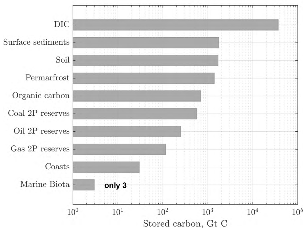
Figure 5.8: Most carbon reservoirs on Earth are enormous, and the largest near-surface store by far is the dissolved inorganic carbon (DIC) in the global ocean. By contrast, the proved plus probable (2P) fossil-fuel reserves – consistent with the IPCC AR6 definitions – constitute one of the smallest human-accessible carbon accumulations. If the possible category is added, the total fossil-fuel endowment expands to the industry’s 3P estimate, giving an ultimately technically recoverable fossil carbon resource of 3P \approx 5,000 Gt C. Data source ( Friedlingstein et al., 2025 ).
