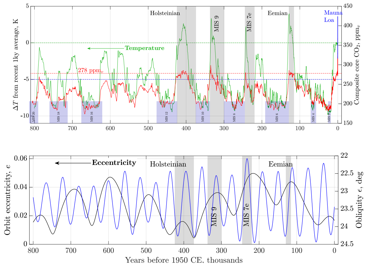
Figure 11.5: Sensitivity of paleoclimate over the last 800,000 years to pCO 2 ( top ) and the Milankovitch cycle forcing ( bottom ). It seems that the interglacial periods were driven usually by high orbit ellipticity (eccentricity), but not the Holsteinian, and low axis tilt (obliquity). When Earth's orbit is at its most elliptic, about 23 percent more incoming solar radiation reaches Earth each year at perihelion than does at its aphelion. The glaciation cycles were driven by low eccentricity. When eccentricity is low the glaciations become less extreme and more stable. Notice that the orbit eccentricity has a period of ~100 kyrs and the beat period (waveform repeats) of 400 kyrs. Data source: Supplementary materials to MacFarling Meure et al. (2006) , PAGES (2016) , NOAA Bereiter et al. (2015b) , Lan et al. (2025a) , calculations by Patzek, 12/30/2023.
