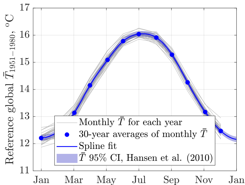
Figure 12.9: The 1951-1980 reference temperature for the Earth. For each grid cell in Figure 12.8, a cell-area analog of this global reference temperature must be used. Here, each monthly temperature anomaly anywhere on the Earth was averaged over 30 years and an average absolute global annual temperature of 14°C was added.
