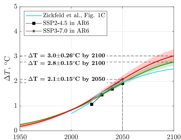
Figure 13.2: Global temperature anomaly vs time, given \Delta T vs. \text{CO}_2 emissions in Figure 13.1 and cumulative \text{CO}_2 emissions vs time in Figure 7.5(b) (the red curve for Patzek’s 568 \text{ppm}_v scenario). The 95% ( 2\sigma ) confidence intervals that fitted curves explain the data are shaded. The Zickfeld et al.’s data fall below our prediction because their CTE was \sim 2 Tt of \text{CO}_2 less than that in the 568 \text{ppm}_v scenario, cf. Figure 7.5(b) .
