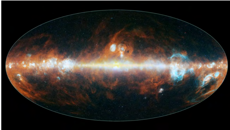
Figure 2.4: NASA’s SPHEREx has mapped the entire sky in 102 infrared colors, which are invisible to the human eye but can be used to reveal different features of the cosmos. This image features a selection of colors emitted primarily by stars (blue, green, and white), hot hydrogen gas (blue), and cosmic dust (red). Credit: NASA / JPL-Caltech.
