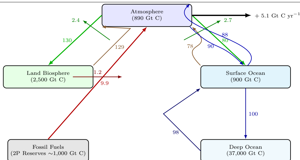
Figure 5.6: Major reservoirs and annual carbon fluxes in the contemporary (2024) global carbon cycle. Large gross biological fluxes (photosynthesis and respiration) are nearly balanced on annual timescales, while anthropogenic emissions and air–sea/air–land imbalances produce the observed atmospheric accumulation. Data source ( Friedlingstein et al., 2025 ).
