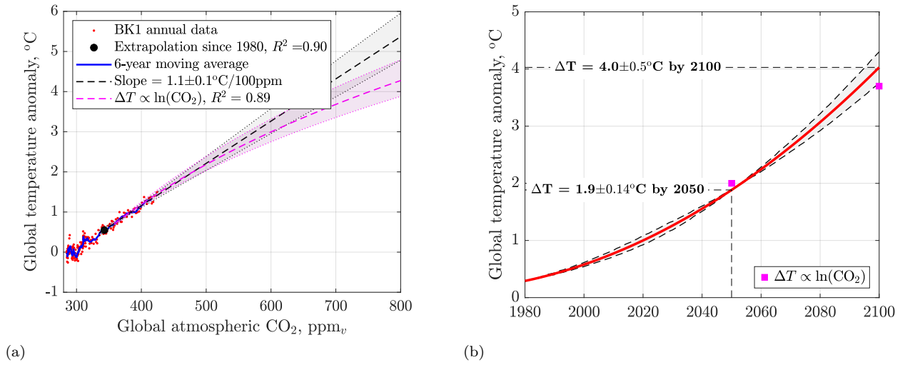
Figure 13.5: Patzek's 720 ppm v scenario. (a) Global temperature anomaly vs. CO 2 emissions, given \Delta T vs. time in Figure 12.10(b) and cumulative CO 2 emissions vs. time in Figure 7.5(b), the black parabola. (b) Global temperature anomaly vs. time, given \Delta T vs. CO 2 emissions in Figure 12.10(a) and cumulative CO 2 emissions vs. time in Figure 7.5(b). The 95% ( 2\sigma ) confidence intervals that the polynomial fits explain the data are shaded.
