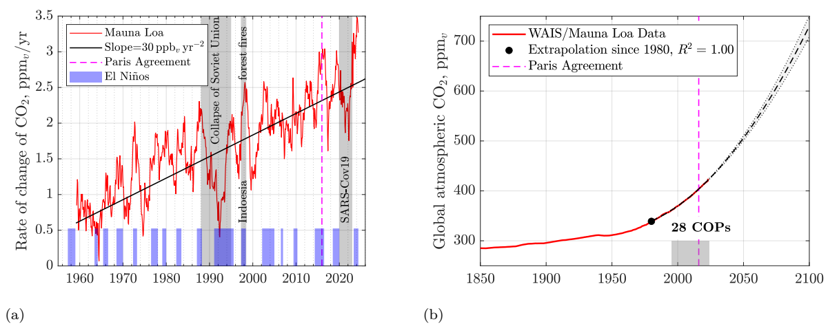
Figure 7.3: (a) Annual increases of atmospheric CO 2 concentration. Notice that the 28 COP meetings have had zero effect on the average annual acceleration of increase of atmospheric CO 2 at (30 ppb v (yr) -2 ). (b) Mixed atmosphere CO 2 concentration since 1850. The pre-1900 global CO 2 concentrations in the atmosphere were estimated from the West Antarctic Ice Sheet ice cores, see Ahn et al. (2012), Etheridge et al. (1996). The quadratic extrapolation curve fits the CO 2 data perfectly between 1980 and 2023 and reaches 720 ppm v by the year 2100, an increase of 300 ppm v relative to June 2023. Also shown is the 95% confidence interval for the curve fit. If nothing changes, we are 95% certain that the predicted CO 2 concentrations will be between 697 and 733 ppm v in the year 2100. But if a lot more coal is used to generate electricity, the likely CO 2 concentration might exceed 800 – 850 ppm v by 2100. Sources: Combined Scripps and NOAA CO 2 data, the Conference of the Parties (COP) dates from UN, calculations by Patzek.
