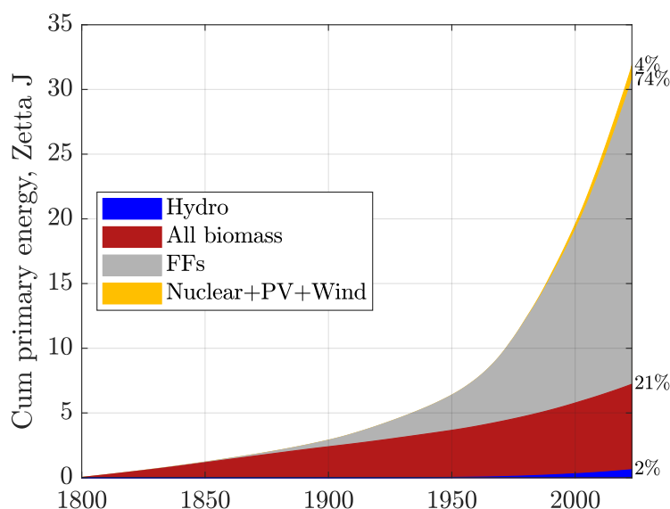
Figure 6.12: Global cumulative primary energy production by source. Please notice that in 2023, biomass and fossil fuels delivered 95% of the primary energy that drove our civilization for the last two centuries. The contribution of each energy source was rounded to an integer, and the results do not add to 100%. Sources: EIA, OWID, Clark and Jacks (2007), Patzek, accessed 01/12/2025.
