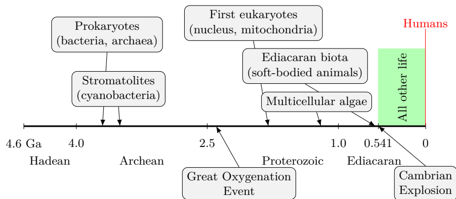
Figure 3.1: Timeline of the dominant life forms throughout the Precambrian, from the first microbial ecosystems to the Ediacaran soft-bodied fauna. All other life that started after the Cambrian Explosion 540 million years ago fits into the green rectangle. The entire human evolution is the thin red line on the far right.
