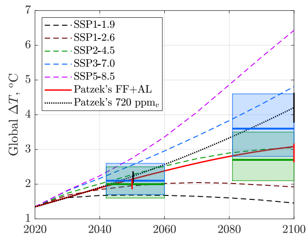
Figure 13.8: Comparison of our emission- and temperature-data-driven model predictions (red) with IPCC's Sixth Assessment Report (AR6). All temperature anomalies are referenced to +1.35^{\circ}\text{C} in 2020. The incremental \text{CO}_2 emissions since 2020 are converted into the corresponding \Delta T s by the multiplication by 0.61^{\circ}\text{C}(\text{Tt CO}_2)^{-1} . The color-coded horizontal lines and rectangles are the most likely temperature ranges over the \sim 18 -year intervals in AR6-Table SPM.1, accessed 01/24/2024. The vertical bars are the 95% confidence intervals from the more detailed calculations here.
