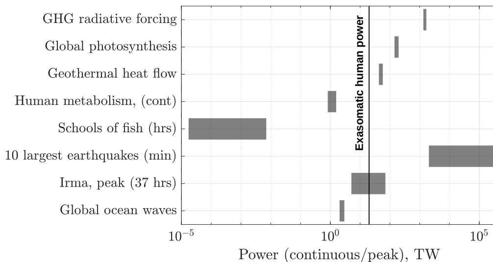
Figure 5.4: Power dissipation by major natural and anthropogenic Earth systems. Calculations by Patzek.
