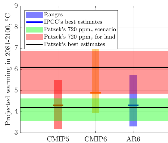
Figure 13.7: Comparison of Patzek's 720 ppm v scenario with IPCC's Sixth Assessment Report (AR6), and CMIP5 and 6. Agreement of Patzek's most probable global \Delta T with those from CMIP5 and AR6 is remarkable. The Climate Model Intercomparison Project, Phase 6 (CMIP6) consists of some 100 distinct climate models produced by 49 different modelling groups. The earlier CMIP5 protocol consisted of thirty five climate model experiments designed to (i) assess the mechanisms responsible for model differences in poorly understood feedbacks associated with the carbon cycle and with clouds, (ii) examine climate "predictability", and (iii) determine why similarly forced models produce different responses. Data source: AR6-Chapter 7 Figures, accessed 09/23/2023.
