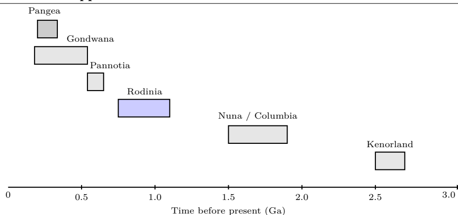
Figure 5.1: Approximate durations of major supercontinents over the last 3 billion years, plotted against time before present in billions of years (Ga). Ages are schematic and compiled from standard reconstructions of Kenorland, Nuna/Columbia, Rodinia, Pannotia, Gondwana, and Pangea. During and after the prolonged breakup of Rodinia, Earth plunged twice into a globally frozen, ice-covered state—the two “Snowball Earth” episodes—that together lasted for roughly 70 million years, about five million years longer than the time elapsed since the extinction of the dinosaurs to the present day.
