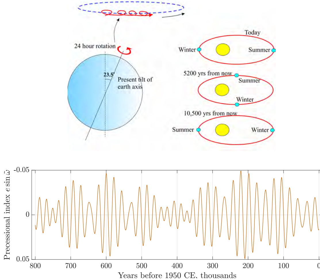
Figure 11.4: The MILANKOVITCH precession cycle refers to the wobble of the axis of Earth's rotation describing a circle in space with a period of 26,000 years. Modulated by orbital eccentricity, precession determines where on the orbit around the Sun (i.e., relative to aphelion or perihelion) seasons occur, thereby increasing the seasonal contrast in one hemisphere and decreasing it in the other. The effect is largest at the equator and decreases with increasing latitude. The periods of the precessional signal modulated by eccentricity are 23,000 and 19,000 years, the periods observed in geological records.
