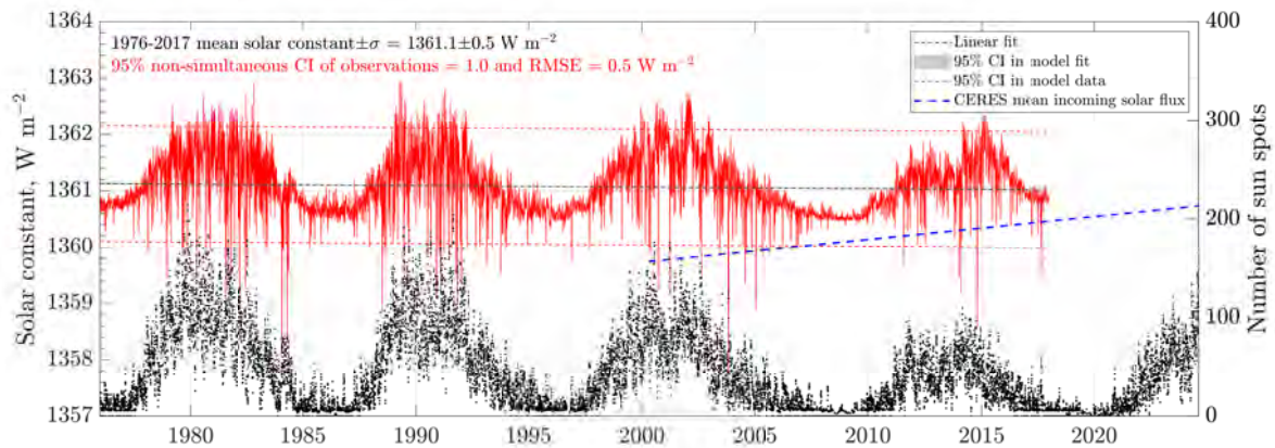
Figure 9.4: The best available reconstruction of the solar constant is based on multiple independent data sets. Over the past 42 years, the solar constant has remained remarkably stable, with a mean value of S_{\oplus} = 1361.1 \pm 0.5 \text{ W m}^{-2} (1 standard deviation), varying by up to \pm 1 \text{ W m}^{-2} ( \pm 0.07\% ) in phase with the solar sunspot cycle. At top of atmosphere (TOA), Earth receives a time-averaged solar irradiance of S_{\oplus}/4 = 1361.1 divided by four = 340.275 \text{ W m}^{-2} . The reduction factor of 1/4 arises from averaging the solar light incidence angles between the equator to the poles ( 1/2 ), and accounting for the Earth rotation (day-night cycle, 1/2 ). The solar constant values are derived from the supplementary data in Gueymard (2018) . CERES radiative fluxes are based on the dataset CERES_EBAF-TOA_Ed4.2_Subset_200003-202407.nc, accessed on February 1, 2025. Monthly sunspot numbers were obtained from the SILSO database at https://www.sidc.be/SILSO/datafiles . Calculations by Patzek.
