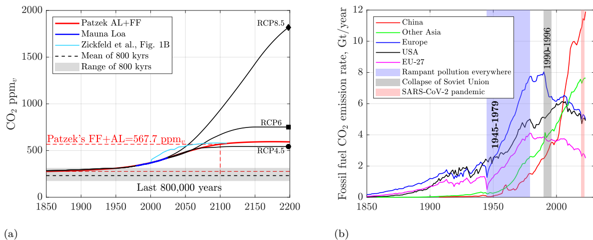
Figure 8.6: (a) Comparison of atmospheric \text{pCO}_2 until 2200, resulting from Patzek's FF+AL scenario and RCP 4.5, 6.0 and 8.5 scenarios ( Meinshausen et al., 2011 ). The Zickfeld et al. simulation curve is also displayed for comparison, showing that equal cumulative \text{CO}_2 emissions lead to equal \text{pCO}_2 s. (b) \text{CO}_2 FF emission rates by region or country. Europe includes the former Soviet Union and Warsaw Pact countries. Sources: EIA, NOAA, OWID, Clark and Jacks (2007) , Patzek, accessed 02/11/2025. Calculations by Patzek.
