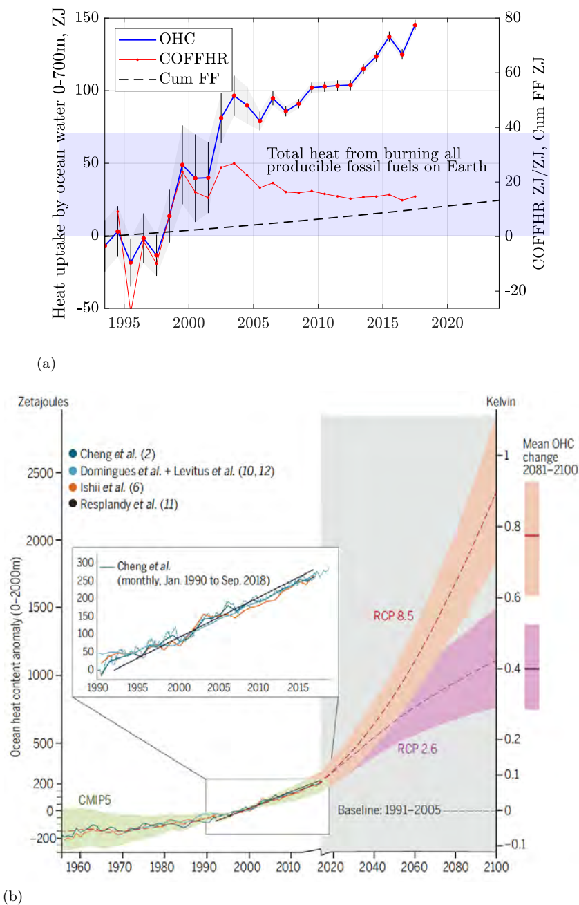
Figure 14.1: (a) Left axis: Cumulative ocean heat content (OHC) in the upper 0 – 700 m reached approximately 150 ZJ by 2018. According to Cheng et al. (2017) , the 0–2000 m ocean layer has already absorbed incremental heat equal to approximately 4× the ~67 ZJ of energy ever generated by fossil fuels, as shown in Figure 8.5(a) . Right axis: Cumulative fossil fuel high heating value (HHV) from 1994 to 2024, and the ratio of cumulative ocean heat to fossil fuel heat. The data indicate that each 1 ZJ of fossil fuel HHV corresponds to 15 – 27 ZJ of heat retained in the upper 0 – 700 m of the ocean. Data sources: NOAA, EIA. (b) Ocean heat content (OHC) for the 0 – 2000 m depth layer. If current trends continue, the thermal burden on the ocean will intensify to levels incompatible with the survival of global industrial civilization. Image source: Cheng et al. (2017) .
