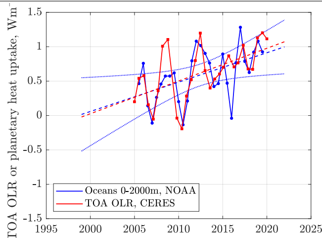
Figure 14.2: Outgoing Longwave Radiation (OLR) forcing by heated ocean water. In the last two decades, the Earth stored \Delta RF = +1 \text{ Wm}^{-2} , or half of incremental \text{CO}_2 forcing since 1750, see Figure 11.1(b). The global climate is controlled by the amount of sunlight absorbed by Earth and the amount of infrared energy emitted to space. These quantities – together with their difference – define Earth’s radiation budget (ERB). TOA OLR CERES = the Top-Of-the-Atmosphere Outgoing Longwave Radiation from the US Clouds and the Earth’s Radiant Energy System (CERES), a project that provides satellite-based observations of ERB and clouds. It uses measurements from CERES instruments flying on several satellites along with data from many other instruments to produce a comprehensive set of ERB data products for climate, weather and applied science research. The CERES instruments provide direct measurements of reflected solar radiation and emission of thermal infrared radiation to space across all wavelengths between the ultraviolet and far-infrared. Data sources: NOAA1 , NOAA2 , and NASA CERES Loeb et al. (2021) , calculations by Patzek.
