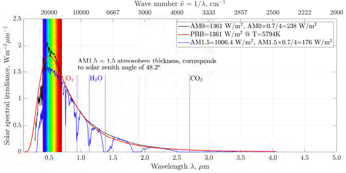
Figure 9.5: The measured and theoretical (Planck's blackbody PBB) solar radiation spectra. Sources: NREL , calculations by Patzek.
