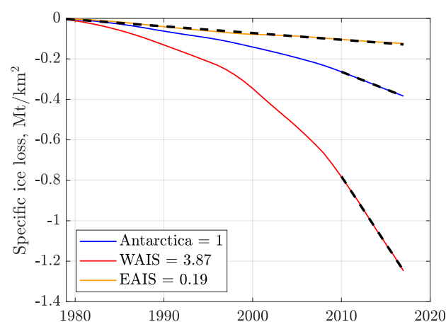
Figure 14.5: The slopes of the dashed lines are the specific rates of ice loss in \text{Mt (yr km}^2)^{-1} between 2010 and 2017. The West Antarctic Ice Sheet (WAIS) lost ice at the rate four times higher than Antarctica, while the East Antarctic Ice Sheet (EAIS) lost ice at the rate five times lower. Data source: Supplementary data set pnas.1812883116.sd01.xlsx to Rignot et al. (2019), accessed on 01/06/2024, calculations by Patzek.
