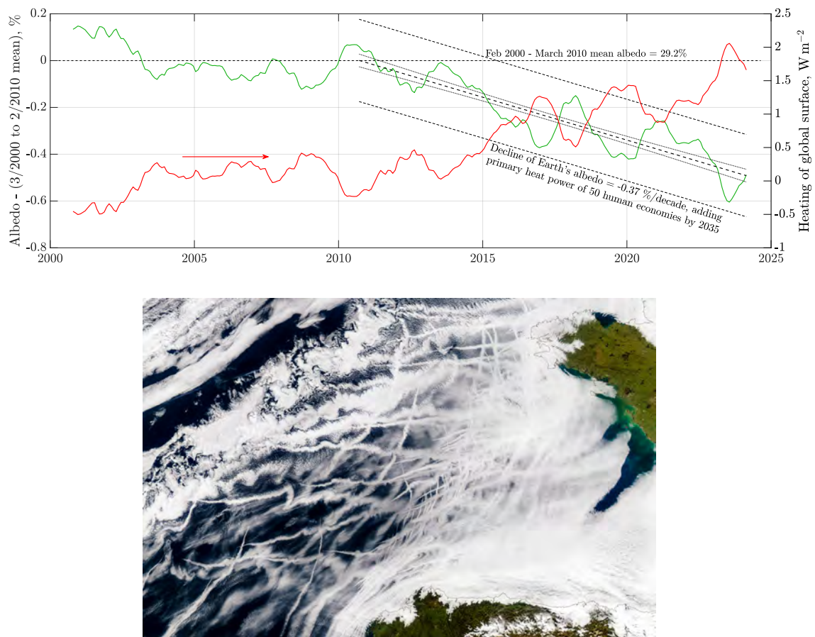
Figure 10.4: Top: The Earth albedo between 2/2000 and 12/2024. The albedo's deviation from the 2/2000-3/2010 mean (the green curve) is a 12-month moving average of the CERES measurements. This change of albedo is translated into more unequilibrated radiative forcing, approaching the total radiative forcing from CO 2 in Figure 9.10(b). Data source: File
