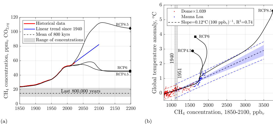
Figure 8.7: (a) Methane concentrations are converted to \text{CO}_{2,eq} by multiplying them by 29.8 ( Arias et al., 2021 ). Historic \text{CH}_4 concentrations are obtained from EPICA Dome C core data multiplied by 1.039 to align the overlapping data points with the Mauna Loa data. Very uncertain future concentrations are predicted by an extrapolation of the linear fit of historic data between 1940 and 2024. Three RCP scenarios are shown for calibration. (b) Global mean annual temperature anomaly vs \text{CH}_4 concentration. The plotted RCP scenarios ( Meinshausen et al., 2011 ) were converted to the corresponding temperature anomalies by multiplying their respective CTE by the average slope of 0.62^\circ\text{C} (\text{Tt CO}_2)^{-1} in Figure 7.7(c) . This calculation is well within the range of global warming probability distributions for RCP4.5, 6 and 8.5 ( Sherwood et al., 2020, Fig. 23 ). Notice that the RCP8.5 trajectory tracks historical data best, but I am quite unsure how predictive its future outcomes are. Data sources: Supplementary materials to MacFarling Meure et al. (2006) , PAGES (2016) , Mauna Loa ( Lan et al., 2025b ). Calculations by Patzek.
