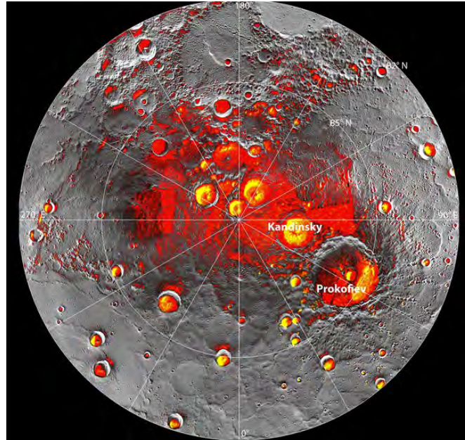
Figure 2.6: Shown in red are areas of Mercury’s north polar region that are in shadow in all images acquired by MESSENGER. Image coverage, and mapping of shadows, is incomplete near the pole. The polar deposits imaged by Earth-based radar are in yellow, and the background image is the mosaic of MESSENGER images. Credit NASA/Johns Hopkins University Applied Physics Laboratory/Carnegie Institution of Washington/National Astronomy and Ionosphere Center, Arecibo Observatory, Oct 22, 2013.
