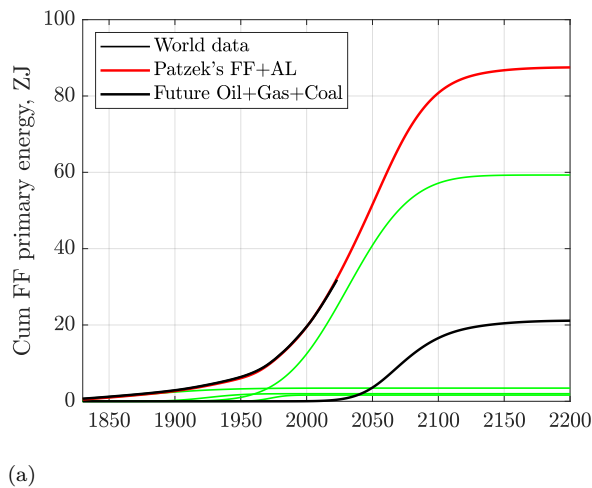
Figure 8.5: (a) Cumulative heat generated by FF fuels until 2200. Roughly 30% of these 88 ZJ of heat is converted to work and the remaining 62 ZJ is heat generated at the Earth's surface. (b) Cumulative heat from incremental radiation forcing by GHGs. Ocean water heat content 0–2000 m depth is likely to reach 1500 ZJ by 2100. Image source: Cheng et al. (2017) . Data sources: EIA, BP, OWID, and World Bank, accessed 9/15/2024; analysis by Patzek.
