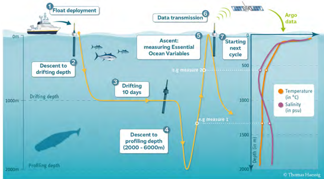
Figure 12.4: Argo float water column profiling cycles. Source: UCSD .
