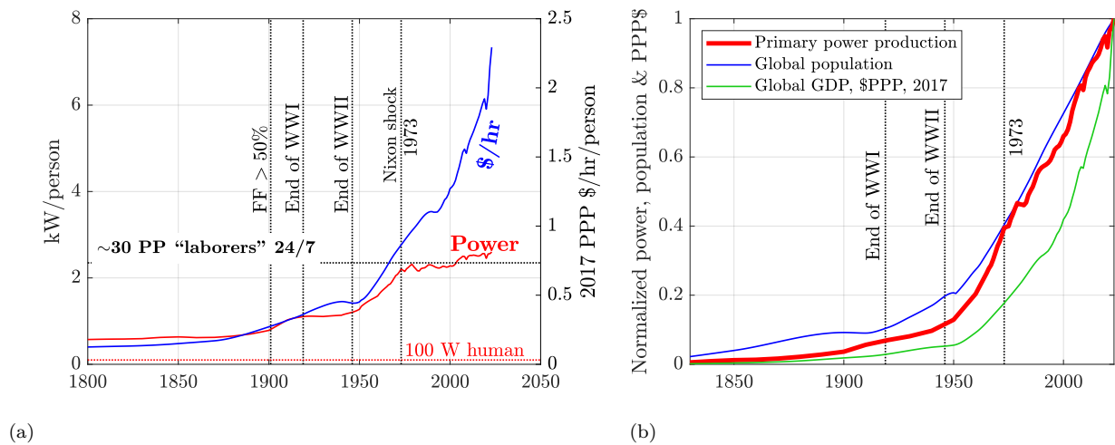
Figure 6.6: (a) Global per capita power consumption in kW, and gross domestic product (GDP) generation power in Purchasing Power Parity (PPP) constant 2017 US dollars per hour per person. Both quantities grew more less in unison until 1973, and diverged afterwards. Oil and gas production peaked in the US in 1971 and 1972, followed by production decline and reservoir repressuring with peripheral waterfloods in the Middle East, and the Arab embargo after the Yom Kippur war in 1973. The growth rates of production of oil and lease condensate and natural gas have been markedly lower post-1973. (b) The total primary energy/time (PP), population and GDP histories are normalized so that they are zero in 1830 and 1 in 2023. Human population and global GDP have been following consumption of primary power, with the population leading until 1973 and the GDP always lagging. Sources: EIA, BP, UN Dept. of Economic and Social Affairs, Population Division and World Bank, accessed 08/30/2023; analysis by Patzek.
