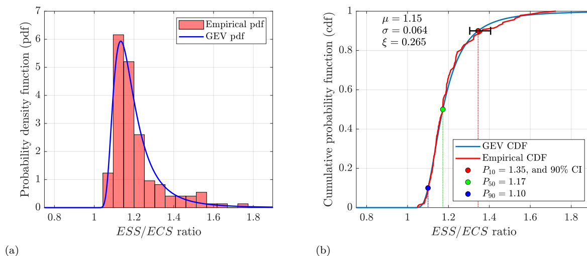
Figure 11.9: The distribution of ESS/ECS ratios for the Eocene climate data shown in Figure 11.8. The data are fit with a Generalized Extreme Value (GEV) distribution Gumbel (1958) , which reduces to a Fréchet distribution with \xi > 0 , left cut-off and right fat tail. (a) The experimental and GEV probability density functions (pdf). (b) The corresponding cumulative distribution functions (cdf) including a 90% confidence interval (CI) on P_{10} . Note that the median value of the ratio is 1.17, and only 10% of data exceed the P_{10} = 1.35 . Thus, most of the time, the ratio of ESS to ECS is between 1.1 and 1.35. Calculations by Patzek.
