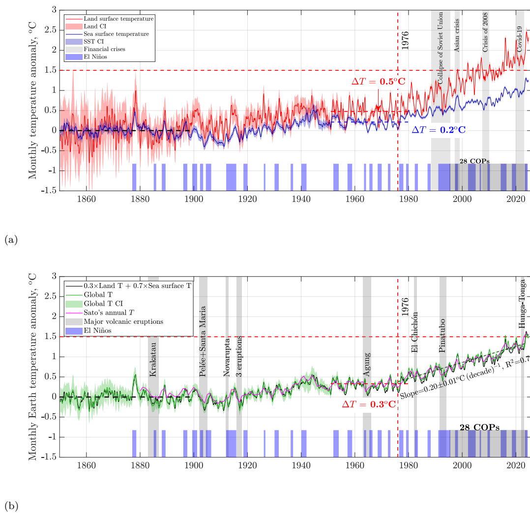
Figure 12.10: All temperature anomalies are relative to the 1850-1900 mean global surface temperature. The 1951-1980 temperature plateau anomalies are shown as the dashed horizontal lines offset by +0.5^{\circ}\text{C} for global land, +0.2^{\circ}\text{C} for SST, and +0.3^{\circ}\text{C} for the Earth. (a) Anomalies of the global land temperature (Land) and sea surface temperature (SST) vs. time. Notice that in 1976, the global land temperature started increasing faster than SST, and the global climate bifurcated. (b) Global monthly temperature anomaly (more precisely, global mean surface air temperature (GMSAT) anomaly) vs. time. As a cross-check, also plotted are the ocean and land areas-weighted average of SST and land temperature anomaly (black curve), and (Sato, 2025) annual temperature anomaly (magenta). All these global anomaly histories are self-consistent. Data sources: Berkeley Earth and HadSST.4.0.1.0, accessed 02/10/2025. Calculations by Patzek.
