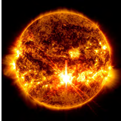
Figure 9.2: The Sun is a G-type main-sequence star, commonly referred to as a yellow dwarf. Its surface occasionally exhibits sunspots – temporary, cooler, and darker regions caused by intense magnetic activity that suppresses convective mixing. Sunspot temperatures range from 3,800 to 4,500 K, significantly cooler than the surrounding photosphere at approximately 5,800 K. In addition to sunspots, the Sun’s fast-changing magnetic field powers solar flares and coronal mass ejections (CMEs) – massive bursts of solar plasma and magnetic fields. A notable example is a solar flare captured by NASA’s Solar Dynamics Observatory on October 3, 2024.
