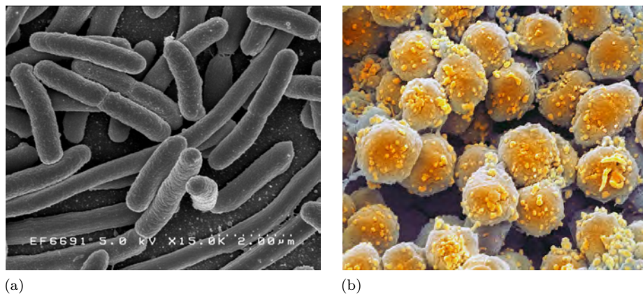
Figure 3.4: Single-celled organisms that lack cell nuclei are called prokaryotes. (a) Typically a few micrometres in length, bacteria were among the first life forms to appear on Earth, and are present in most of its habitats. Bacteria inhabit soil, water, acidic hot springs, radioactive waste, and the deep biosphere of the Earth's crust. Bacteria are vital in many stages of the nutrient cycle by recycling nutrients such as the fixation of nitrogen from the atmosphere. They can cause cholera, syphilis, anthrax, leprosy, and bubonic plague. The most common fatal bacterial diseases are respiratory infections. Image: SEM of Escherichia coli , grown in culture and adhered to a cover slip. Credit NIAID. (b) Despite their morphological similarity to bacteria, archaea possess genes and several metabolic pathways that are more closely related to those of eukaryotes, notably for the enzymes involved in transcription and translation. Other aspects of archaeal biochemistry are unique, such as their reliance on ether lipids in their cell membranes. Archaea are a major part of Earth's life. They are a part of the microbiota of all organisms. In the human microbiome, they are important in the gut, mouth, and on the skin. Credit Steve Gschmeissner / Science Photo Library.
