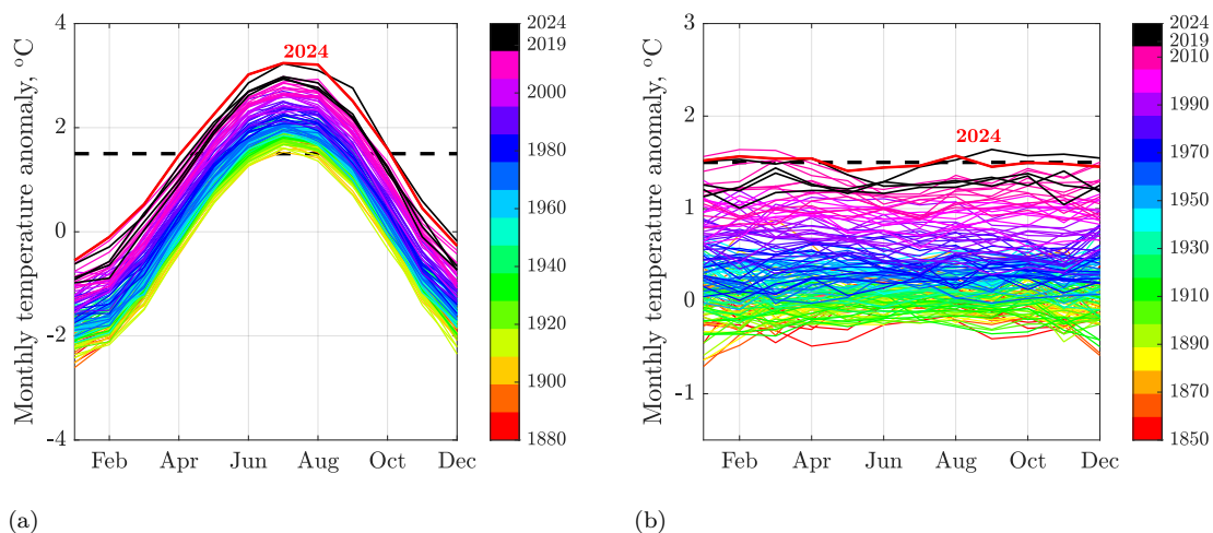
Figure 12.11: Stacked global temperatures colored by decade. The years 2020-2023 are shown in black and the record-breaking 2024 is a thick red curve. The thick horizontal dashed line is the +1.5^{\circ}\text{C} temperature anomaly. (a) Seasonal temperatures of both hemispheres. (b) The stacked monthly global temperatures eerily resemble increasing water level in a tub filling with water that is warming most of the time. The almost horizontal water surface in this analogy has been controlled by clouds that make the Earth's albedo uniform. Data sources: NASA GISTEMP ( NASA, 2015 ) and Berkeley Earth, accessed 2/10/2025. Calculations by Patzek.
