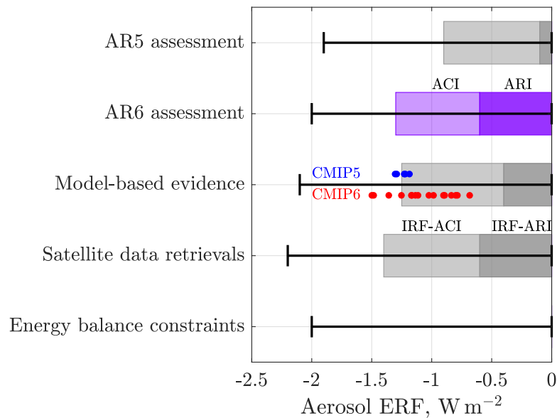
Figure 10.2: Aerosol net effective radiative forcing (ERF) from different lines of evidence. IRF ARI refers to the Instantaneous Radiative Forcing (IRF) from Aerosol-Radiation Interactions (ARI). Similarly ACI refers to Aerosol-Cloud Interactions. The headline AR6 assessment of -1.3 [ -2.0 to -0.6 ] ( \text{mean}[\text{min to max}] ) \text{W m}^{-2} is highlighted in purple for 1750-2014 and compared with the AR5 assessment of -0.9 [ -1.9 to -0.1 ] \text{W m}^{-2} for 1750-2011 (note a discrepancy between the AR5 bars in IPCC's Figure 7.5 and the supporting data). The evidence comprising the AR6 assessment consists of climate model-based evidence of -1.25 [ -2.1 to -0.4 ] \text{W m}^{-2} ; observational evidence from satellite retrievals of -1.4 [ -2.2 to -0.6 ] \text{W m}^{-2} ; and energy balance constraints [ -2 to 0 ] \text{W m}^{-2} with no best estimate. Based on the data to Figure 7.5 in Masson-Delmotte et al. (2021) . Calculations by Patzek.
