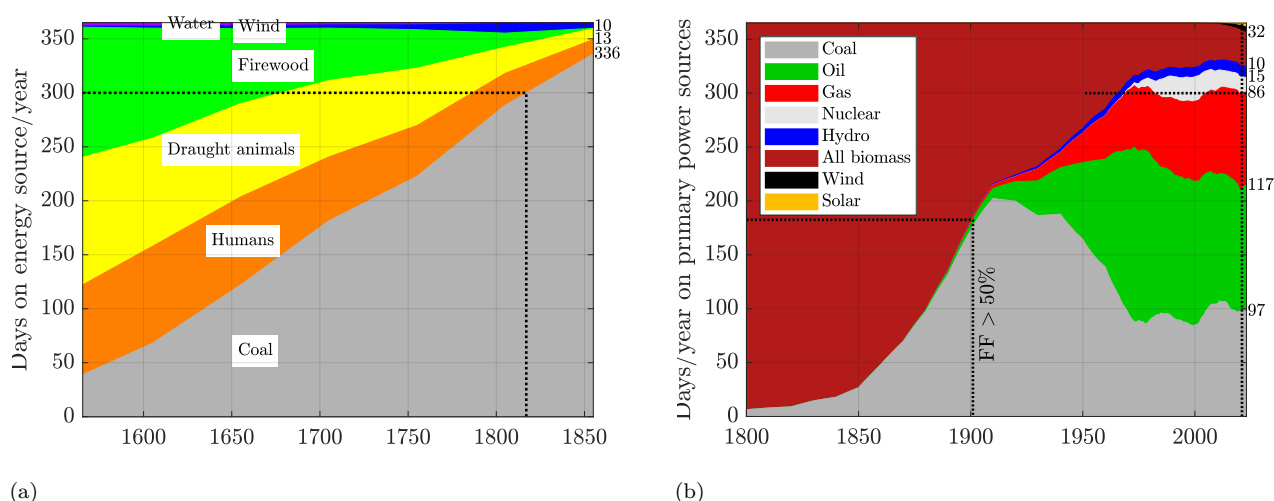
Figure 6.9: Days per year on each primary power source for Britain (a) and the world (b). The data from Wrigley (2016) were converted to days per year on a given primary energy source in Britain since 1565. The two horizontal lines at 300 days/year, denote Britain's dependence on coal by 1817 and world's dependence on fossil fuel since 1951. The vertical line on the right in the onset of the SARS-CoV-2 virus pandemic. Other sources: EIA, OWID, accessed 01/21/2025. Calculations by Patzek.
