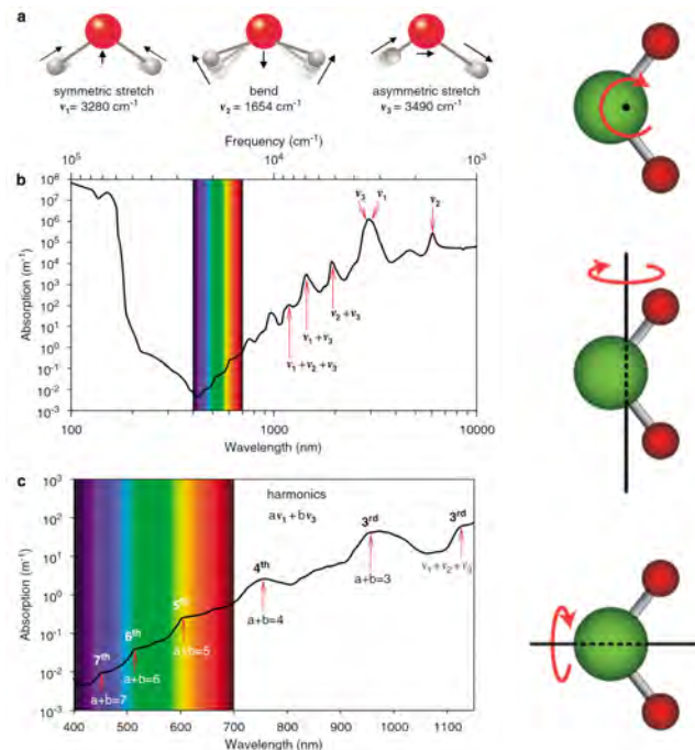
Figure 9.8: Sources: Figure 2 in Stomp et al. (2007) (left) and https://www.xaktly.com/Water.html (right). Radiation absorption by \text{H}_2\text{O} vapor (similar, but not identical for \text{CO}_2 ). (a) The three vibrational modes of the water molecule and their fundamental frequencies in liquid water: symmetric stretching ( \nu_1 ), bending ( \nu_2 ) and asymmetric stretching ( \nu_3 ). The atoms move in the directions indicated by arrows. (b) Absorption spectrum of pure water. Peaks in the absorption spectrum correspond to the fundamental frequencies and higher harmonics of the vibrations of the water molecules. (c) Absorption spectrum of pure water in the visible and infrared region. Shoulders in the absorption spectrum correspond to the third, fourth, fifth, sixth and seventh harmonics of the symmetric and asymmetric stretch vibrations, as indicated.
