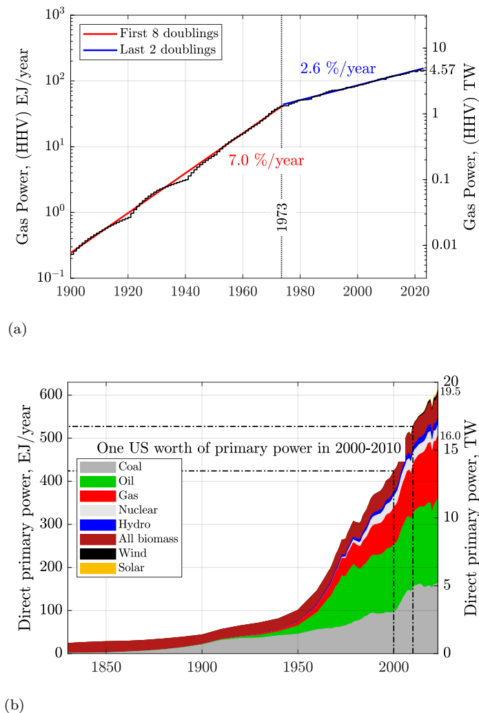
Figure 6.11: (a) The global rate of natural gas production underwent approximately 10 doublings between 1900 and 2023. After 1973, however, the exponential growth rate of natural gas production declined by nearly a factor of three – substantially less than the corresponding slowdown observed for oil production (see Figure 6.10). (b) Direct primary power developed by each source of primary energy since 1830. Today the human world is a giant \sim 20 TW machine. “Direct” means that no division by average fossil fuel power plant efficiency (0.40) to convert PV and wind electricity into a “fossil fuel equivalent” is performed, essentially multiplying their output by a factor of 1/0.40 = 2.5 . Primary power is primary power, and without these accounting gimmicks solar PV and wind are almost invisible. Sources: EIA, OWID, Clark and Jacks (2007), Patzek, accessed 11/11/2024.
