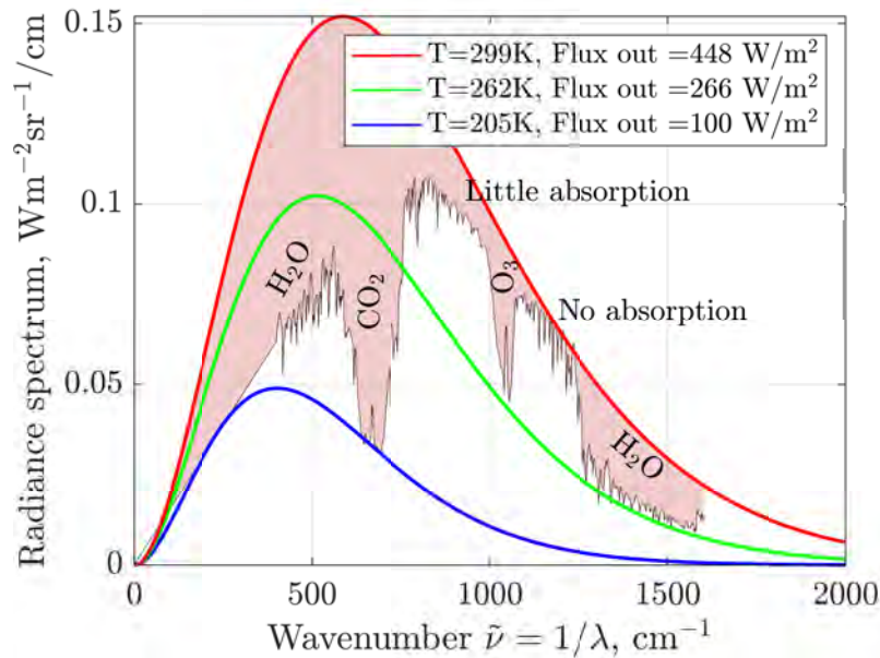
Figure 9.9: The energy-density spectrum of outgoing thermal radiation from the Earth at wave numbers ranging from 400 to 1600 \text{cm}^{-1} (black jagged curve). Equivalent wavelengths of 6.3-25 microns are in the mid- and far-infrared bands (see Definition 12). The pink area is due to net absorption of the outgoing energy flux by greenhouse gases that block parts of the Planck blackbody radiation of ground surface at the temperature of 299 K. These spectral radiance data were measured on May 5, 1970, 12:00:07 with NASA's IRIS instrument on the Nimbus 4 satellite. Here you can see one of the earliest satellite measurements of Earth's outgoing longwave radiation that have since become critical to monitoring our planet's energy balance. Data source: NASA. Calculations by Patzek.
