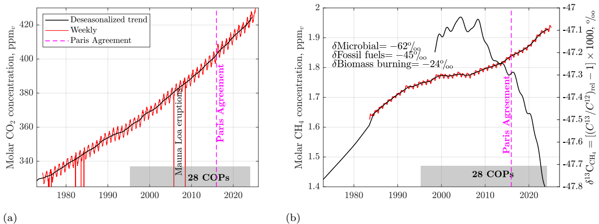
Figure 7.2: (a) The weekly average values of mixed-atmosphere molar concentration of CO 2 and their trend. (b) Weekly average values of molar concentration of methane and their trend. The carbon isotopic composition of atmospheric CH 4 ( \delta^{13}\text{C}_{\text{CH}_4} ) is a powerful tool because different CH 4 sources have distinctive \delta^{13}\text{C}_{\text{CH}_4} signatures ( Michel et al., 2024 ) (the right axis). Current unprecedented growth of methane concentration to almost 2 ppm v or 2 \times 29.8 \approx 60 ppm v of CO 2,eq seems to have a growing microbial component (up to 20% of the weighted average) caused by global climate change, and agriculture and land use change. The main component ( \sim 80\% ) are industrial methane emissions, especially from oil and gas fields, and processing facilities. Data source: Mauna Loa, ( Lan et al., 2025a,b ); El Niño Southern Oscillation (ENSO): Wikipedia .
