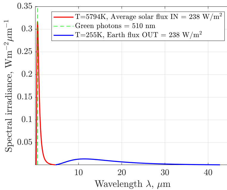
Figure 9.7: The solar radiation spectrum is scaled by the factor of (1 - \alpha)/4 so that both areas under the irradiance spectra are equal. The Planck blackbody radiation curves in Equation (B.26) are plotted at the absolute temperatures of 5794 and 255 K, respectively. Notice that the two spectra are disjoint. The solar spectrum ends at the infrared light wavelengths at which the Earth spectrum begins. Calculations by Patzek are based on Equation (B.26).
