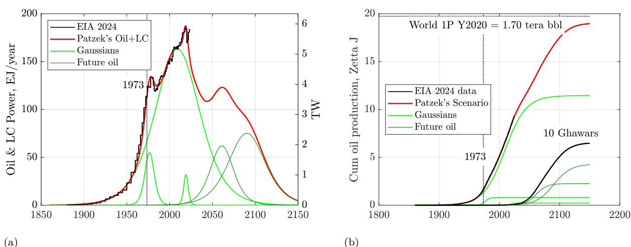
Figure 8.3: (a) The global crude oil and lease condensate power, with two very large Gaussians representing future production. (b) Cumulatively the world will produce the 2020 1P reserves or ~19 ZJ; 6.4 ZJ or 10 Ghawars at 100 billion bbl each will be produced in the future. Data sources: EIA, BP, OWID, and World Bank, accessed 9/15/2024; analysis by Patzek.
