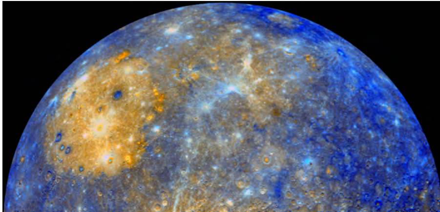
Figure 2.5: NASA’s MESSENGER mission: a false color mosaic of an eastern limb of Mercury. Credit: NASA/Johns Hopkins University Applied Physics Laboratory/Carnegie Institution of Washington, Oct 22, 2010.
