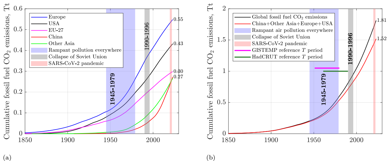
Figure 10.1: Cumulative fossil fuel CO 2 emissions by (a) country and region, and for the world and high-emitters (b). Sources: EIA, OWID, Clark and Jacks (2007) , Patzek, accessed 01/11/2024.
