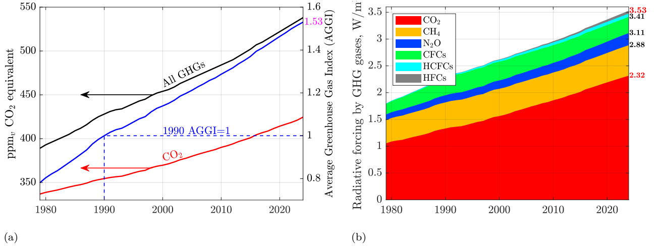
Figure 9.10: (a) Accumulation of CO 2 and all GHG gases in the atmosphere (left y -axis) and the NOAA Annual Greenhouse Gas Index (AGGI), normalized to the year 1990 (right y -axis). (b) Radiative forcing, relative to 1750, of virtually all long-lived greenhouse gases. Data sources: (Dlugokencky et al., 2025), see the caption of NOAA's Figure 3 for the list of key GHGs. Calculations by Patzek.
