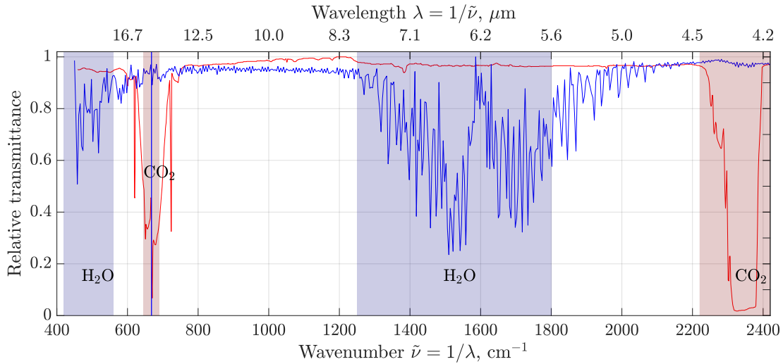
Figure 15.3: The infrared relative transmittance of pure gaseous CO 2 and pure water vapor. The displayed range of wave numbers covers that in Figure 9.9. The CO 2 spectrum was obtained at the CO 2 pressure of 200 mmHg diluted to a total pressure of 600 mmHg with N 2 . Calculations by Patzek. Source: The US National Institute of Standards and Technology (NIST) Chemistry WebBook.
