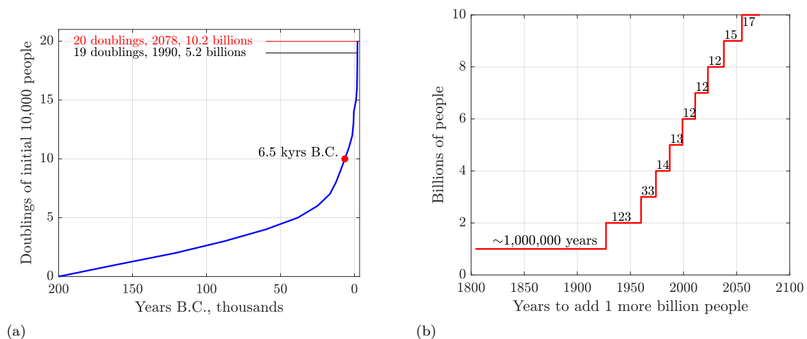
Figure 6.1: The power of exponential growth illustrated by successive doublings ( 2^0 , 2^1 , 2^2 , ...) of a human cohort initially numbering 10,000 individuals around 200,000 BCE. The timing of these doublings is aligned with widely accepted reconstructions of historical human population size. Notably, between 900,000 and 800,000 BCE, humans nearly went extinct, with only about 1,000 individuals surviving in Africa ( Hu et al., 2023 ). For the subsequent 600,000 years, the global human population remained small, averaging only \sim 27,000 individuals at any given time. Thus, a cohort of 10,000 people living 200,000 years ago could plausibly have represented nearly all anatomically modern humanity. If such a cohort were to double twenty times, it would reach approximately 10.2 billion people by the year 2078. There will not be a twenty-first doubling. (b) Years required to add each successive billion people. Sources: Early population data from Rex Weyler (2017, private communication) and UN Department of Economic and Social Affairs, Population Division (accessed 2023-08-30). Calculations by Patzek.
