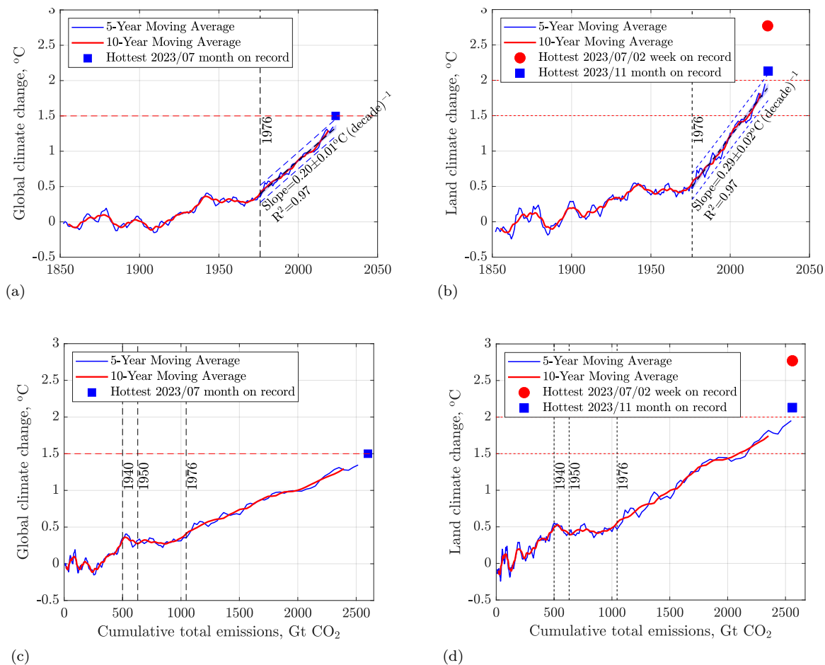
Figure 12.12: Global and land climate change, 1850-2024. The climate temperature anomalies relative to 1850-1900 are calculated as the moving 10-year averages of the annual anomaly data to smooth out the effects of weather. The five-year running averages are also shown for comparison. (a) Global climate temperature anomaly. (b) Land climate temperature anomaly. In 1951, the FF emissions rate exceeded that of AL and in 1976 cumulative FF emissions exceeded those of AL. Notice that the sharp kinks in global temperatures in 1976 (Figure 12.10) are smeared by the moving averages. The post-1976 temperature slopes are (a) , 0.2 \pm 0.01^\circ\text{C} (\text{decade})^{-1} , and (b) 0.3 \pm 0.02^\circ\text{C} (\text{decade})^{-1} . The 95% certainty ( \pm 2\sigma ) intervals for the models are shaded in blue and for the observations appear as dashed blue lines. (c) and (d) same as (a) and (b) but plotted vs. cumulative CO 2 emissions. The 1940-1976 hiatus reflects the uncontrolled global air pollution that dampened temporarily solar irradiation of much of the Earth's surface.
