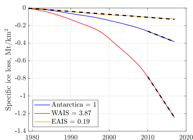
Figure 14.5: The slopes of the dashed lines are the specific rates of ice loss in \text{Mt (yr km}^2)^{-1} between 2010 and 2017. The West Antarctic Ice Sheet (WAIS) lost ice at the rate four times higher than Antarctica, while the East Antarctic Ice Sheet (EAIS) lost ice at the rate five times lower. Data source: Supplementary data set pnas.1812883116.sd01.xlsx to Rignot et al. (2019), accessed on 01/06/2024, calculations by Patzek.
