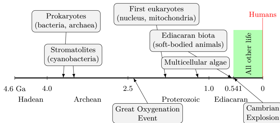
Figure 3.1: Timeline of the dominant life forms throughout the Precambrian, from the first microbial ecosystems to the Ediacaran soft-bodied fauna. All other life that started after the Cambrian Explosion 540 million years ago fits into the green rectangle. The entire human evolution is the thin red line on the far right.
