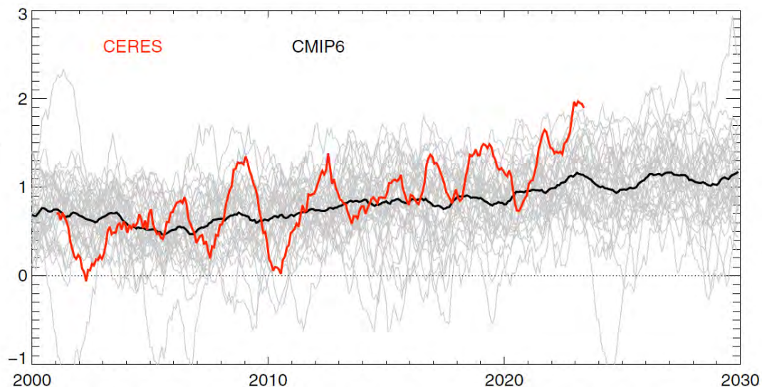
Figure 9.11: Trends in Earth energy imbalance (EEI) from CERES (in red) data and CMIP6 models (black and gray). The CERES data are shown from 2001 to 2023. The CMIP6 data are shown from 2000 to 2030. All EEI are given as 12-month running means. CMIP6 model mean is shown by a thick black line and individual models are shown in thin gray lines. Only one ensemble member for each of the models is shown. Notice that the ocean heat uptake in Figure 14.2 is referenced to zero in the year 2000, and is consistent with this figure. Source: Fig. 1 in ( Myhre et al., 2025 ), reproduced with permission.
