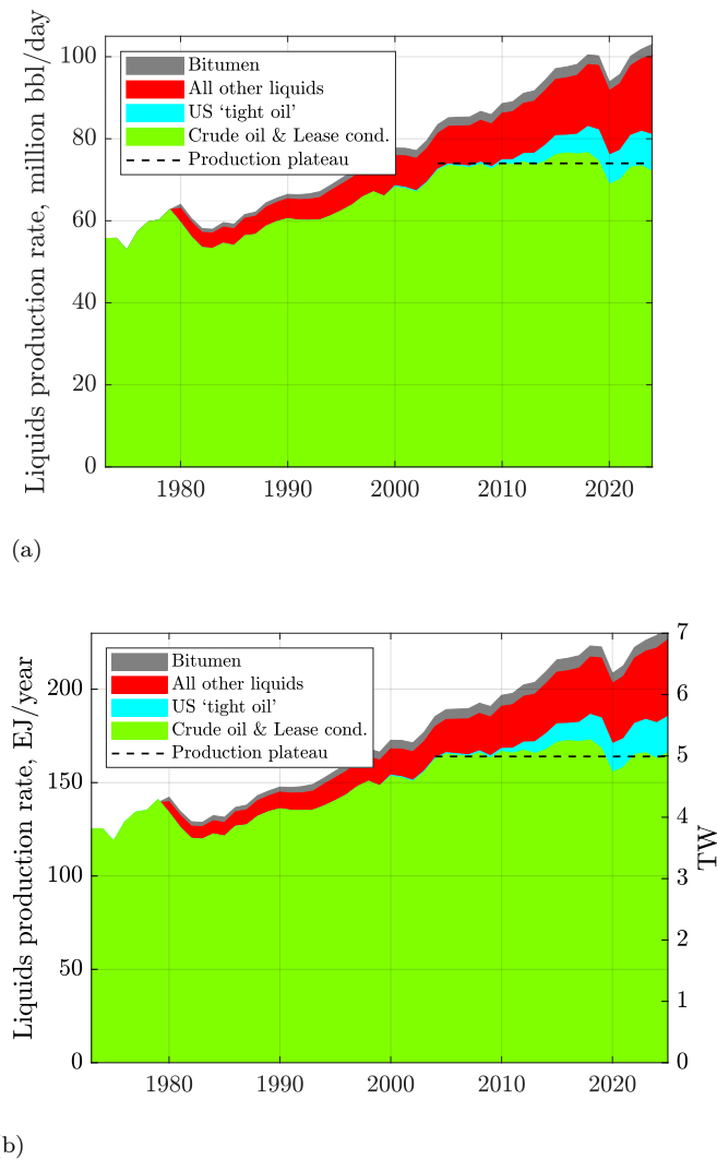
Figure 6.12: (a) Global liquid-fuel production rate. The green area represents the production of conventional crude oil and associated lease condensate. This production rate plateaued at approximately 73 million barrels per day in October 2004 and has since oscillated around that level without a sustained upward trend. The only substantial increase in global light-oil production has come from predominantly U.S. shale (“tight oil”) formations, shown in blue, with the majority of this growth originating in the Permian Basin of Texas and New Mexico. The expansion of other liquids (red area) accounts for most of the apparent increase in global liquid-fuel production from roughly 82 to 102 million barrels per day, with bitumen contributing approximately 2 million barrels per day. (b) Same as panel (a), but expressed in consistent energy and power units ( \text{EJ yr}^{-1} and TW). Sources: EIA, OWID, and Texas Railroad Commission; data accessed 11 January 2026.
