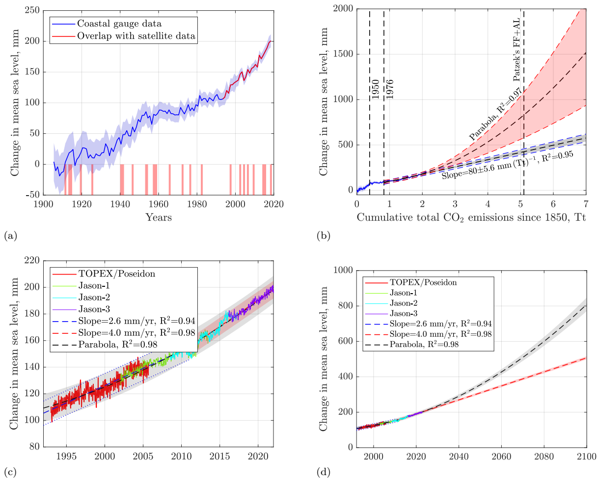
Figure 14.6: (a) Mean global sea level rise 1900-2022. The 1900-1910 mean sea level is zero. This reference makes it easier to understand that in 120 years AL+FF emissions already caused over 20 cm of average sea level rise with much more to come soon to a coast near you. There might be a correlation with some of the El Niños. (b) Same as (a), but now plotted against cumulative total CO 2 emissions. The new parametrization compresses the 1900-1950-time interval (lower emissions) and linearizes better the post-1976 level rise. Of the two extrapolations, the linear one is more conservative and stable, while the parabola captures better the residual curvature of the post 1976-data, i.e., the acceleration of sea level rise, and predicts 830 \pm 244 mm of sea level raise by the year 2100 or 5.1 Tt of CO 2 emissions in Patzek's FF+AL scenario. (c) Mean global sea level rise 1993-2023, shifted upwards by 106 mm to coincide the coastal gauge data zeroed in 1900. (d) same as (c) but now extrapolated to 2100. There are two linear fits of data (1993-2011 and 2011-2023) and one parabolic fit (1993-2023). The second linear fit and the parabolic fit are extrapolated to 2100. In 2100, the linear extrapolation falls within 15 mm of that in (b) at 7 Tt, but the quadratic one is 2\sigma lower than that in (b). The 95% confidence intervals ( \pm 2\sigma ) are shaded. Data sources: NASA (coastal gauges), NOAA (satellites), NOAA references and Wikipedia , calculations by Patzek.
