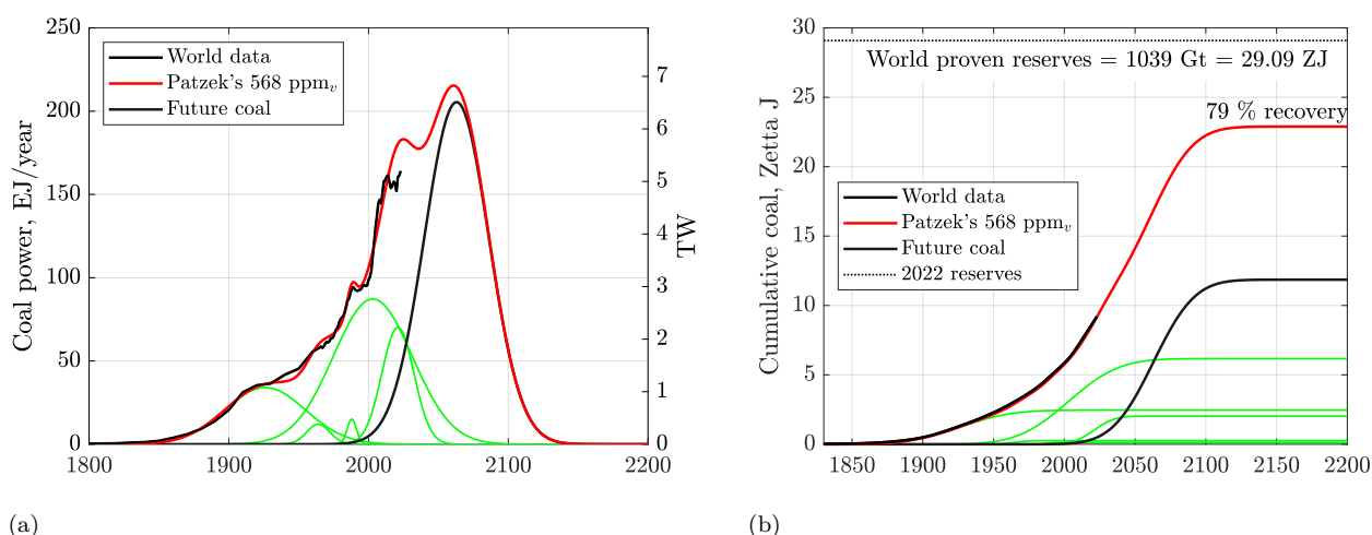
Figure 8.3: (a) Patzek's scenario of future coal production rate. The Gaussian representing future coal production is the largest ever. (b) Patzek's scenario of cumulative coal production predicts that 79% of global coal reserves will be produced. Data sources: EIA, BP, OWID, accessed 08/30/2024; analysis by Patzek.
