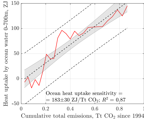
Figure 14.3: Heat absorption by the ocean water in Figure 14.1(a) replotted vs cumulative total CO 2 emissions.
