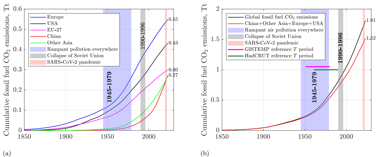
Figure 10.1: Cumulative fossil fuel CO 2 emissions by (a) country and region, and for the world and high-emitters (b). Sources: EIA, OWID, Clark and Jaks (2007) , Patzek, accessed 01/11/2024.
