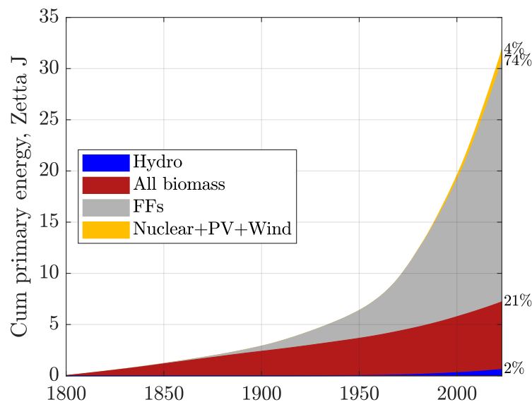
Figure 6.15: Global cumulative primary energy production by source. Please notice that in 2023, biomass and fossil fuels delivered 95% of the primary energy that drove our civilization for the last two centuries. The contribution of each energy source was rounded to an integer, and the results do not add to 100%. Sources: EIA, OWID, Clark and Jacks (2007) , Patzek, accessed 01/12/2025.
