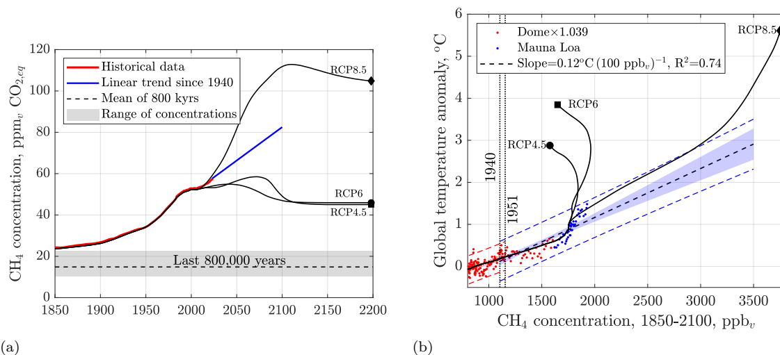
Figure 8.8: (a) Methane concentrations are converted to CO 2,eq by multiplying them by 29.8 (Arias et al. , 2021). Historic CH 4 concentrations are obtained from EPICA Dome C core data multiplied by 1.039 to align the overlapping data points with the Mauna Loa data. Very uncertain future concentrations are predicted by an extrapolation of the linear fit of historic data between 1940 and 2024. Three RCP scenarios are shown for calibration. (b) Global mean annual temperature anomaly vs CH 4 concentration. The plotted RCP scenarios (Meinshausen et al. , 2011) were converted to the corresponding temperature anomalies by multiplying their respective CTE by the average slope of 0.62 °C (Tt CO 2 ) -1 in Figure 7.7(c). This calculation is well within the range of global warming probability distributions for RCP4.5, 6 and 8.5 (Sherwood et al. , 2020, Fig. 23). Notice that the RCP8.5 trajectory tracks historical data best, but I am quite unsure how predictive its future outcomes are. Data sources: Supplementary materials to MacFarling Meure et al. (2006), PAGES (2016), Mauna Loa (Lan et al. , 2025b). Calculations by Patzek.
