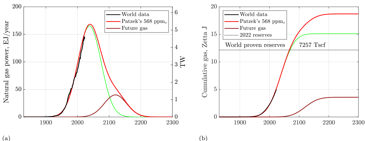
Figure 8.5: (a) The historic rate of global gas production is represented with one green Gaussian, whose unknown height is set to exceed the proven 2022 gas reserves by 35%. The future production is also represented with a single Gaussian. (b) Cumulatively the world might produce 19 ZJ as the HHV of natural gas, including 3.6 ZJ from the future projects. Data sources: EIA, BP, OWID, and World Bank, accessed 9/15/2024; analysis by Patzek.
