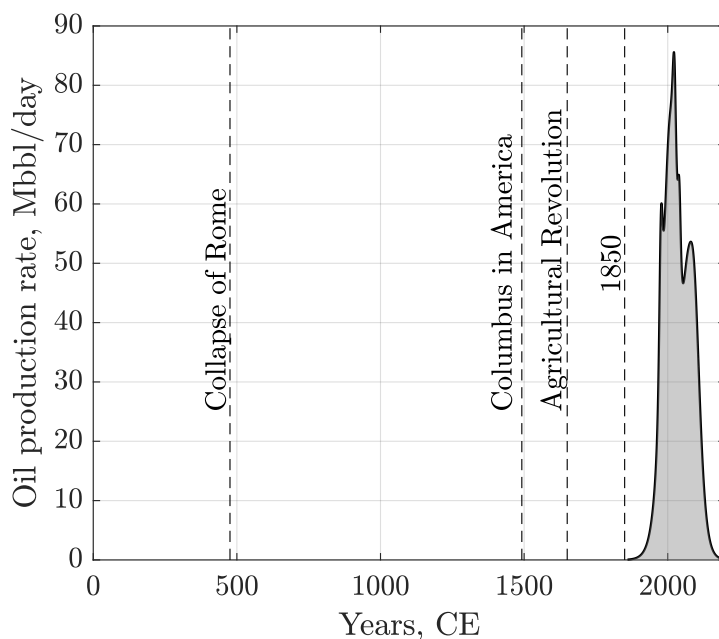
Figure 8.1: Patzek's crude oil and lease condensate production scenario referenced to year 0 of the Common Era (CE). The lifetimes of everyone we have ever known personally fall inside of the gray Washington-Monument-like spike.
