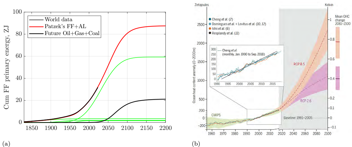
Figure 8.6: (a) Cumulative heat generated by FF fuels until 2200. Roughly 30% of these 88 ZJ of heat is converted to work and the remaining 62 ZJ is heat generated at the Earth's surface. (b) Cumulative heat from incremental radiation forcing by GHGs. Ocean water heat content 0–2000 m depth is likely to reach 1500 ZJ by 2100. Image source: Cheng et al. (2017) . Data sources: EIA, BP, OWID, and World Bank, accessed 9/15/2024; analysis by Patzek.
