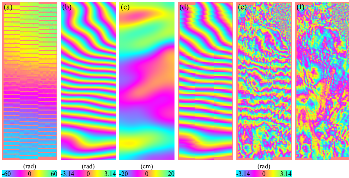
Fig. 5. InSAR ionospheric correction for Sentinel-1 TOPS mode. (a) Ionospheric phase at the ionosphere layer. (b) Filtered ionospheric phase at the ionosphere layer. (c) Azimuth shift caused by ionosphere. (d) Phase for correction. (e) Original interferogram with ESD applied. (f) Corrected interferogram. Note that the values in (a)-(d) are wrapped. The data partly cover northern Chile with a size of 250km×690km (range×azimuth) and were acquired on October 29, 2017 and November 10, 2017 on ascending track 149.
