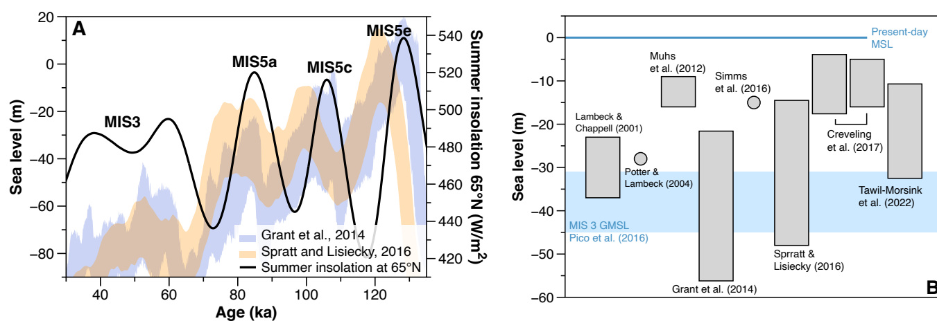
Supplementary Figure 8: A. Summer insolation at 65°N between 35 and 135 ka (Laskar et al., 2004), with indication of the insolation peaks of MIS 5e, MIS 5c, MIS 5a and MIS 3. Sea-Level reconstructions from \delta^{18}\text{O} in benthic foraminifera (Spratt & Lisiecki, 2016) and planctonic \delta^{18}\text{O} in the Red Sea (Grant et al., 2014). 95% confidence intervals are shown for both records. B. GIA and uplift-corrected estimates of MIS 5a GMSL from Huon Peninsula (Papua New Guinea) (Lambeck & Chappell, 2001), the North Atlantic (Potter & Lambeck, 2004), Pacific coasts of North America (Muhs et al., 2012; Simms et al., 2016), Barbados (Tawil-Morsink et al., 2022) and the results of the global inversion by Creveling et al. (2017) (the two values correspond to GMSL calculated using the entire database or only a subset with more reliable constraints). MIS 5a GMSL is also shown for the reconstructions of Grant et al. (2014) and Spratt and Lisiecki (2016) shown in panel A. MIS 3 GMSL reconstructed by Pico et al. (2016) is shown for reference.
