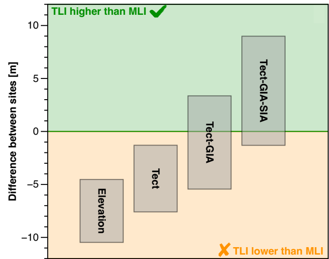
Figure 3: Difference between the marine limiting index point (MLI) in Nueva Palmira and the terrestrial limiting point (TLI) in Chuy Creek (AC-01) after applying different corrections. From left to right: elevation only, Tectonics only, GIA+Tectonics, GIA+SIA+Tectonics.
