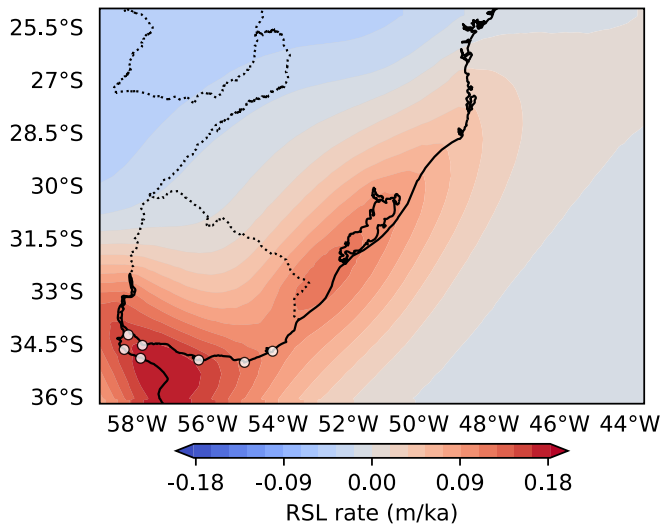
Figure 5: Rate of RSL change (positive = land subsidence) caused by SIA (50% loading scenario) in the study area. The dots on the map mark the locations where data from tide gauges records in the Río de la Plata region are available.
