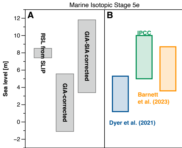
Figure 2: A. MIS 5e relative sea level (RSL) in Osorio as indicated by (from left to right) uncorrected sea level index point (SLIP), GIA-corrected and GIA+SIA corrected SLIP. B. GMSL in MIS 5e as estimated by Barnett et al. (2023) and Dyer et al. (2021) and the IPCC AR6 (Gulev et al., 2021).
