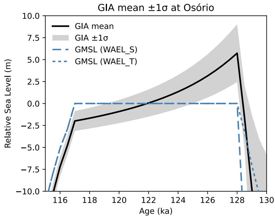
Supplementary Figure 1: Mean and standard deviation of relative sea-level histories reconstructed at Osório using the GIA models of Dyer et al. (2021). The blue lines represents GMSL according to two different MIS 6 configurations (see the Methods section for details), with "WAEL_S" corresponding to a MIS 6 maximum at 135.5 ka, and "WAEL_T" at 142 ka.
