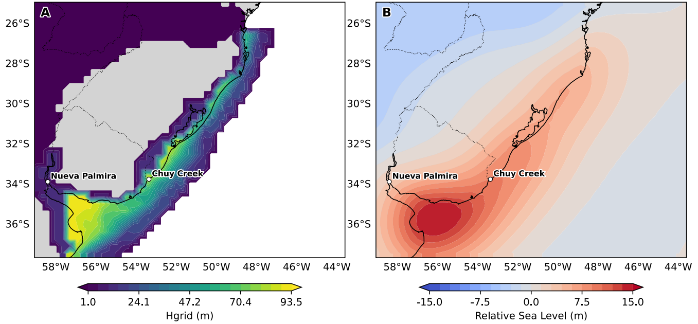
Figure 4: A. Sediment loading (100% loading scenario) on the the Río de la Plata continental shelf between MIS 5a and present-day (100% loading scenario). B. Relative sea-level change (for the 100% loading scenario) since 80 ka caused by sediment isostatic adjustment (SIA). Positive values represent subsidence, negative represent uplift caused by SIA (see standard deviation in Supplementary Figure 6 ).
