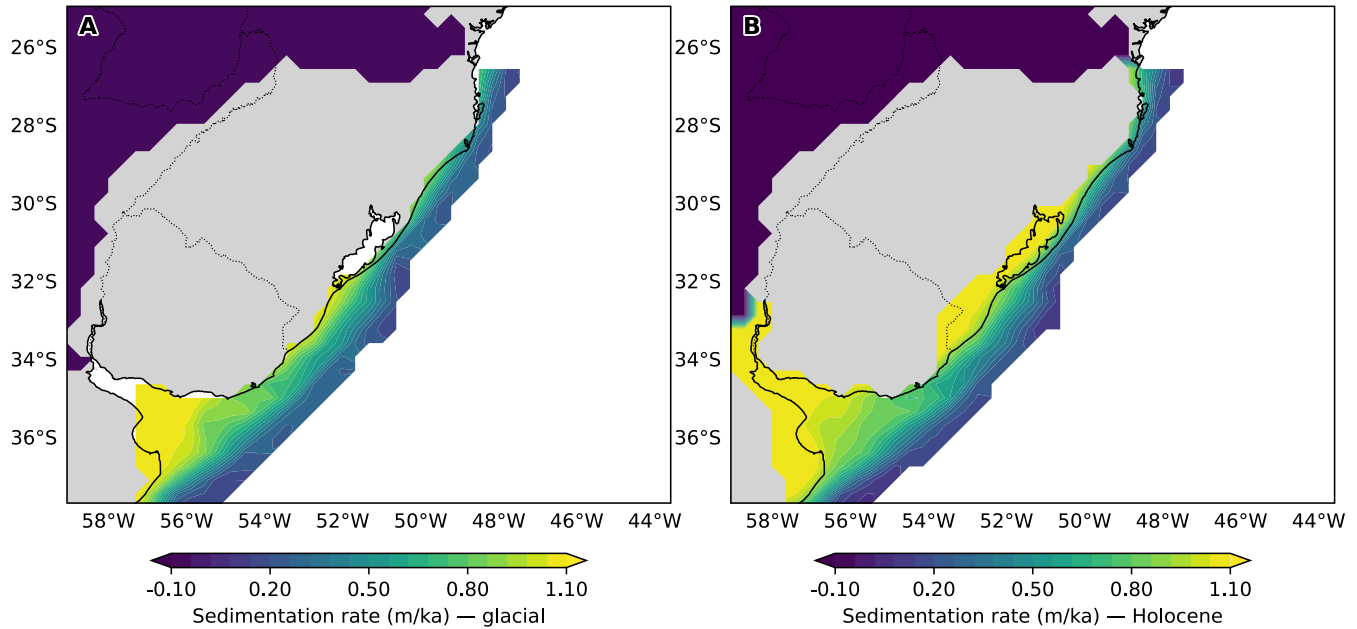
Figure 7: A. Sedimentation rate applied between 122 ka to 10.5 ka. B. Sedimentation rate applied from 10.5 ka to modern.
