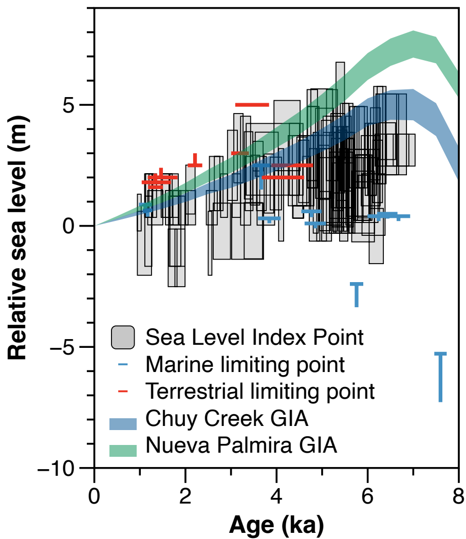
Supplementary Figure 11: Sea level index points and limiting data as compiled by Rubio Sandoval et al. (2025) the Río de la Plata region, together with RSL as predicted by the GIA model ensemble of Dyer et al. (2021) at Nueva Palmira and Chuy Creek.
