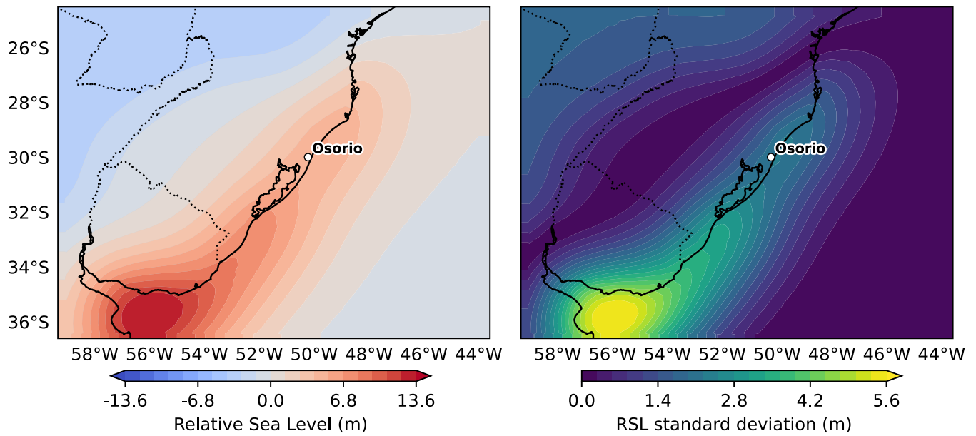
Supplementary Figure 3: A) and B) maps of mean and standard deviation across the four loading scenarios of the subsidence since 122 ka caused by sediment isostatic adjustment (SIA). In panel A positive values represent subsidence, negative represent uplift caused by SIA. The Osorio site where MIS 5e deposits outcrop is shown on the map.
