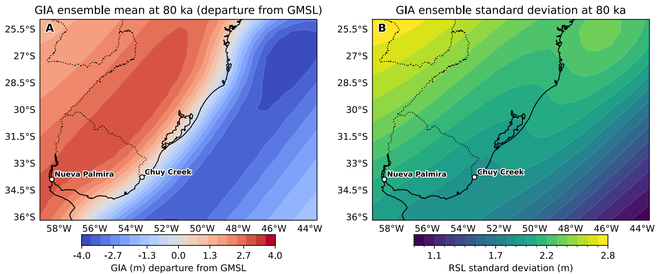
Supplementary Figure 4: A) and B) maps of mean and standard deviation of the departure from GMSL at MIS 5a using the GIA models of Dyer et al. (2021). The two sites where MIS 5a deposits outcrop are shown on the map. Timeseries for these two sites are shown in Supplementary Figure 5 .
