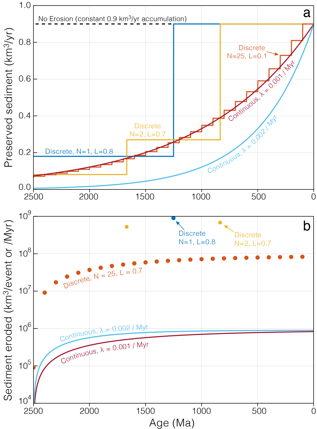
Supplementary Figure 4: Effects of continuous and discontinuous erosion in a model with constant 0.9 km 3 y sediment input prior to erosion. Following Gregor [10], erosion is assumed to consume preexisting crust in proportion to its abundance. (a) : Preserved sediment volume per unit time for several imposed continuous and discontinuous erosion scenarios. (b) : Mass of sediment eroded per event or per unit time, for the same scenarios as in (a) . In the discontinuous erosion scenarios, erosion occurs during one or more discrete erosional events, producing step functions in preserved sediment volume. The strength of a given discrete erosional event is specified in terms of a loss factor: L = 0.8 specifies an erosional event in which 80% of all accumulated sediment present at the time of the event is eroded. The erosion rate in continuous erosion models, meanwhile, is determined by the decay constant \lambda , with units of 1/Myr. Discontinuous models with N equally-spaced events of identical L converge towards the exponential form of continuous erosion as N becomes large. Note, for instance, the correspondence in preserved volume between the discrete model where 10% of the crust is lost every 100 Myr, and the continuous model with a \lambda = 0.001/\text{Myr} (i.e., 10%/100 Myr).
