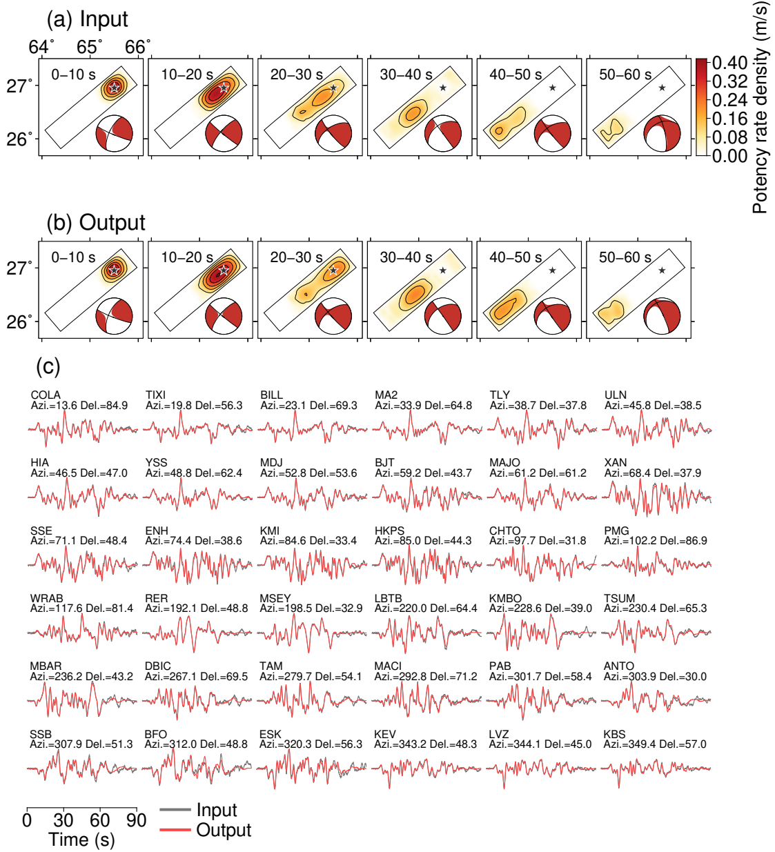
Figure S2. Snapshots of (a) input source model and (b) output source model, and (c) waveform fitting at all stations between input and output synthetic waveforms in the case 1. (a, b) Colour shows the potency-rate density. Contour interval is 0.08 m/s. The black line outlines the model fault. The star denotes the epicentre. The large red beach ball represents the centroid potency-density tensor at each time window. (c) The waveforms are plotted with a sampling interval of 0.05 s. Station code, azimuth, and epicentral distance are shown above the traces.
