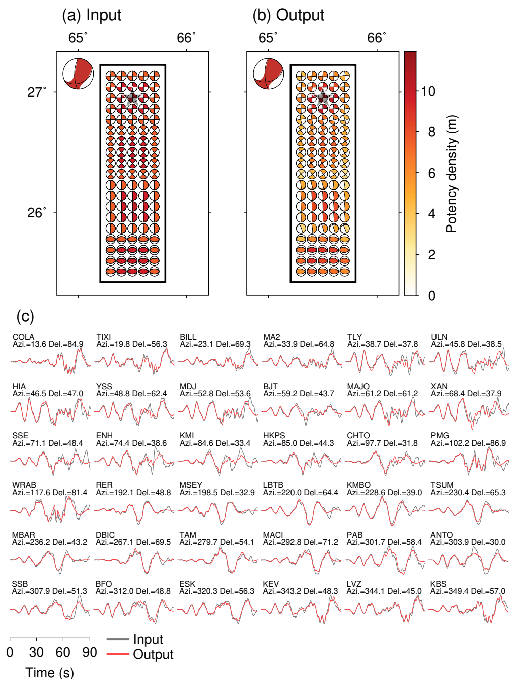
Figure S5. (a) Input source model, (b) Output source model, and (c) waveform fitting at all stations between input and output synthetic waveforms in the case 3. (a, b) The beach ball colour shows the potency density. The dashed line outlines the model fault, and the bold black line shows the top of the model fault, respectively. The star denotes the epicentre. The large red beach ball represents the total moment tensor obtained by taking a spatial integration of the potency-density tensors. (c) The waveforms are plotted with a sampling interval of 0.05 s. Station code, azimuth, and epicentral distance are shown above the traces.
