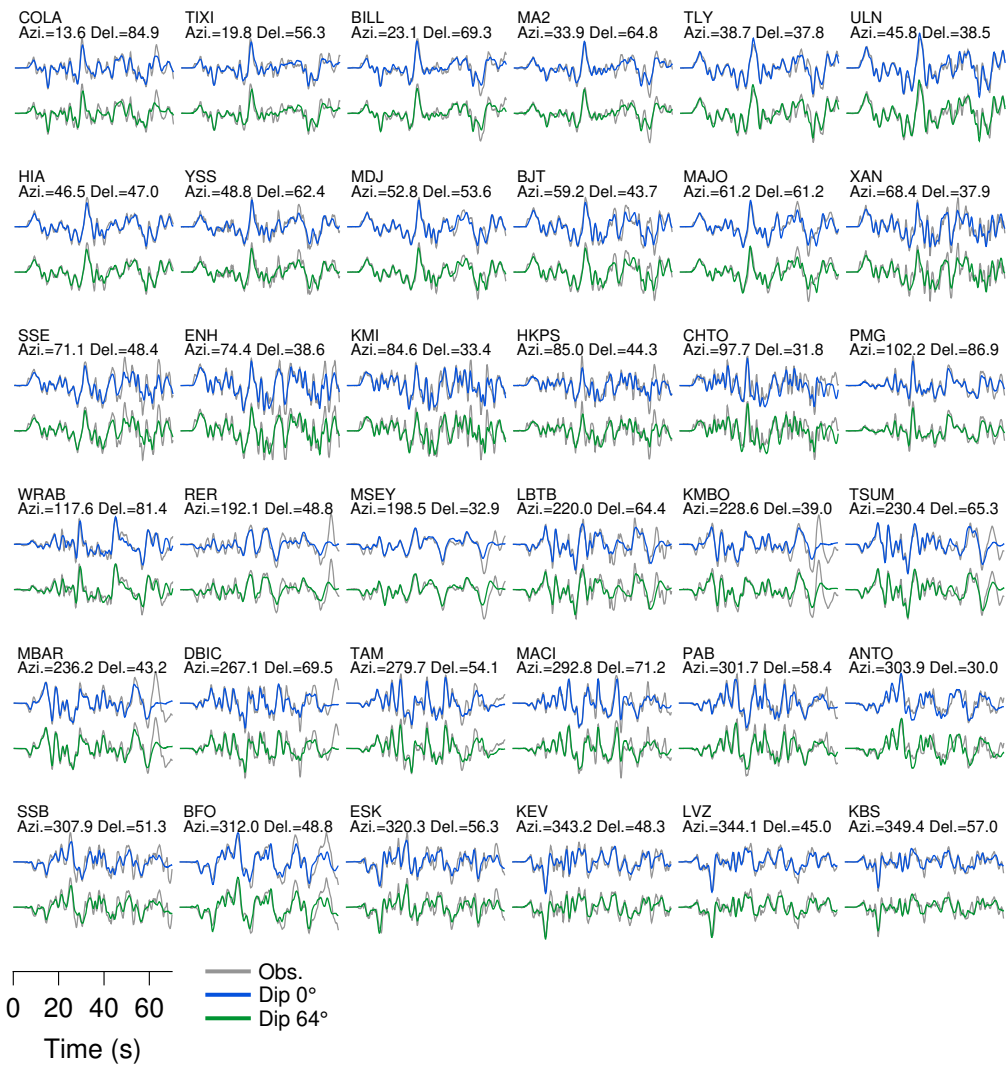
Figure S10. Waveform fitting at all stations between observed (grey line) and synthetic waveforms for the model planes dipping 0° (top blue line) and dipping 64° (bottom green line). The waveforms are plotted with a sampling interval of 0.05 s. Station code, azimuth, and epicentral distance are shown above the traces.
