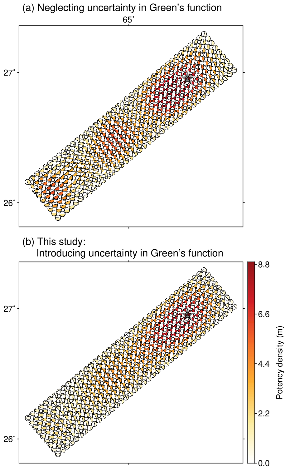
Figure S12. Spatial distribution of the potency-density tensors obtained by using (a) the formulation that neglects uncertainty of Green's function and (b) the one developed in this study introducing uncertainty of Green's function into the data covariance matrix. The small beach ball shows the focal mechanism at each source knot, plotted using a lower-hemisphere stereographic projection. The star denotes the epicentre. The beach ball colour shows the potency density.
