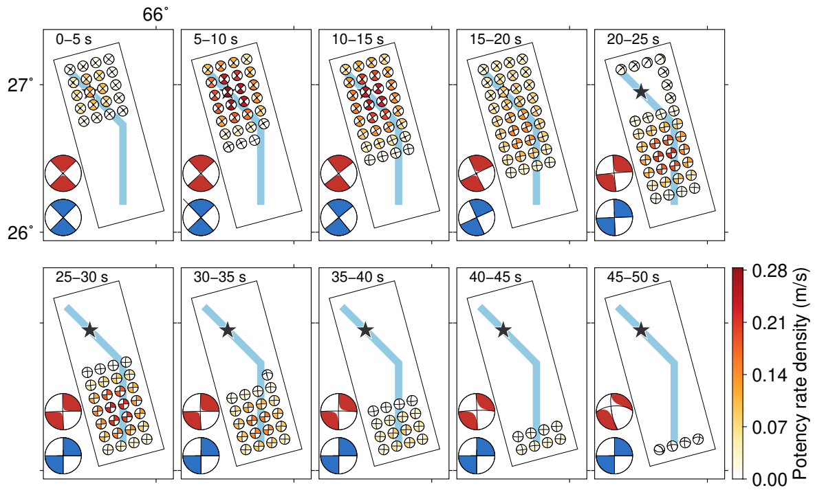
Figure S8. Snapshots of output source model. Colour shows the potency-rate density in the case 4. The star denotes the epicentre. The black line outlines the model fault. The blue line represents the top of a fault plane of the input source model. The small beach ball shows the focal mechanism at each source knot, plotted using a lower-hemisphere stereographic projection. The large blue and red beach ball are the centroid potency-density tensor at each time window of the input and output source models, respectively.
