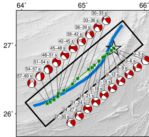
Figure S13. The evolution of the centroid of the potency-rate-density tensors. The centroid locations (green squares) of the potency-rate density and its potency-density tensor is shown at each time window, along with the distance between the neighbouring centroid locations and the corresponding time window for estimation of the centroid location. The blue line represents the surface-rupture trace measured by Zinke et al. (2014). The rectangle outlines the model plane. The star denotes the epicentre.
