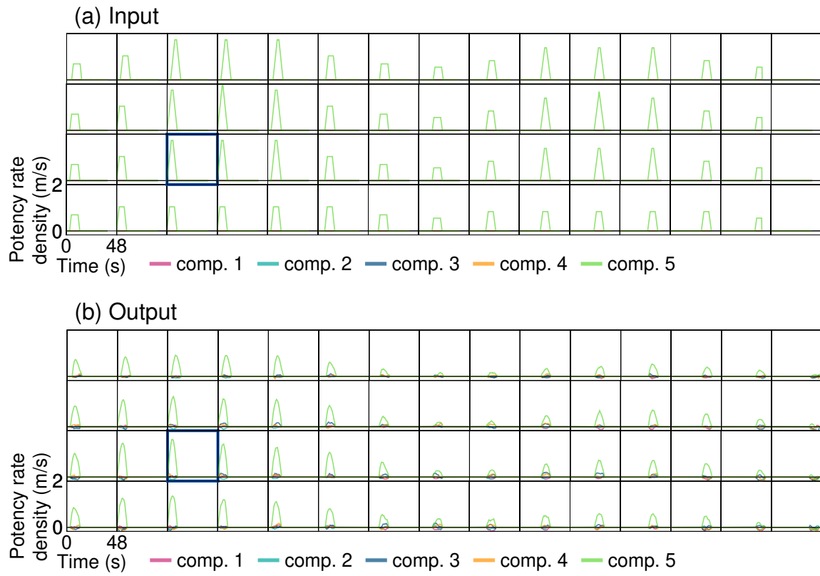
Figure S4. (a) Input and (b) output potency-rate-density functions on an assumed model fault in the case 2. The sub-fault outlined by blue line shows the initial rupture point. Potency-rate-density functions for all basis double-couple components are represented as different colour traces.
