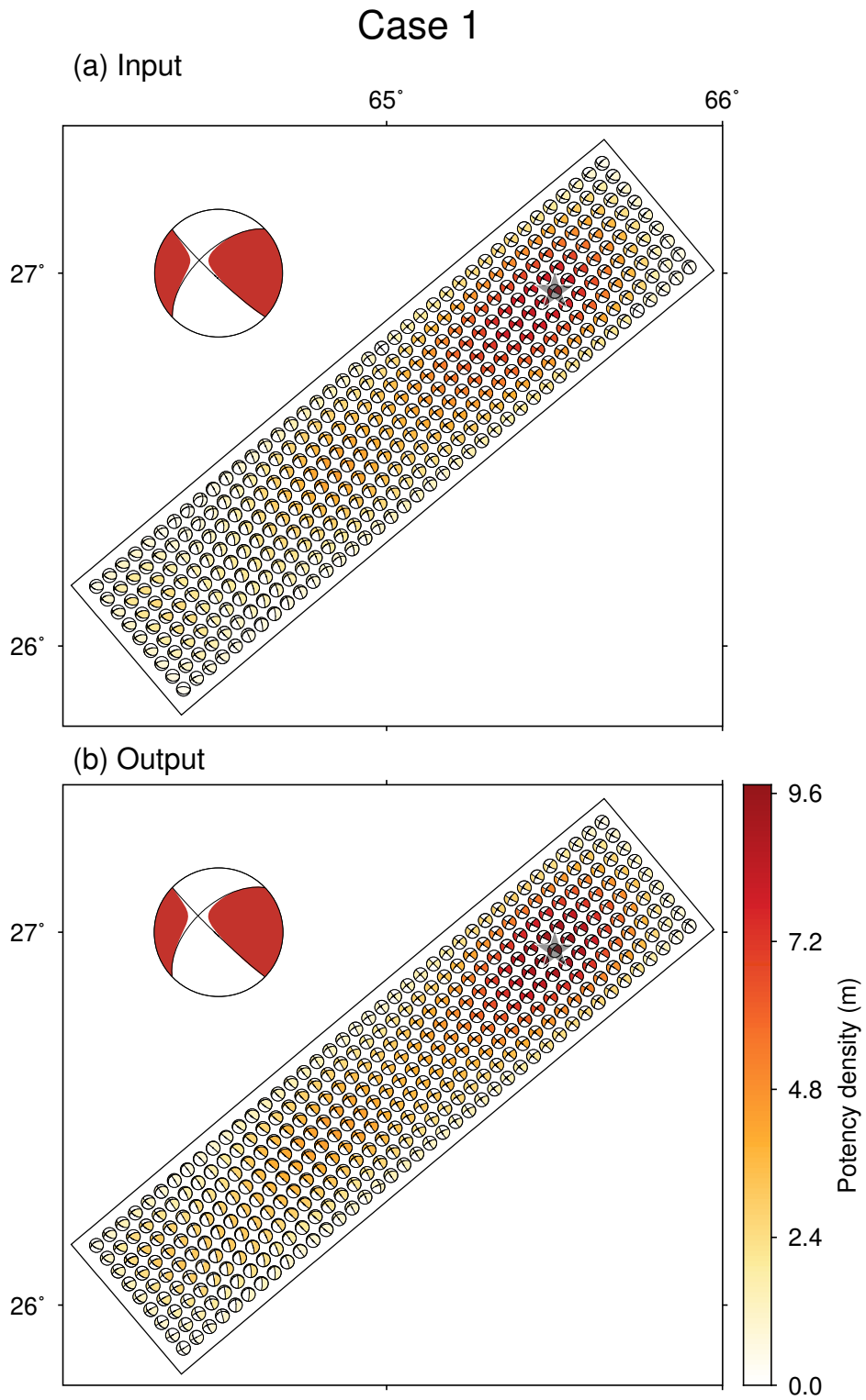
Figure S1. (a) Input source model and (b) Output source model in the case 1. The small beach ball colour shows the potency density. The black line outlines the model fault. The star denotes the epicentre. The large red beach ball represents the total moment tensor obtained by taking a spatial integration of the potency-density tensors.
