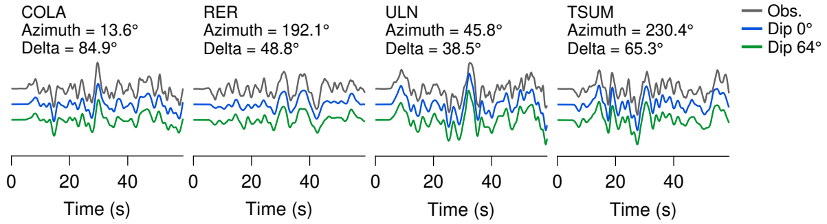
Figure 7. Fitting of waveforms between observed (top grey line) and synthetic waveforms for the model planes dipping 0° (middle blue line) and dipping 64° (bottom green line). The waveforms are plotted with a sampling interval of 0.05 s. The stations were selected to highlight the difference in the results of the fittings. Station code, azimuth, and epicentral distance are shown above the traces.
