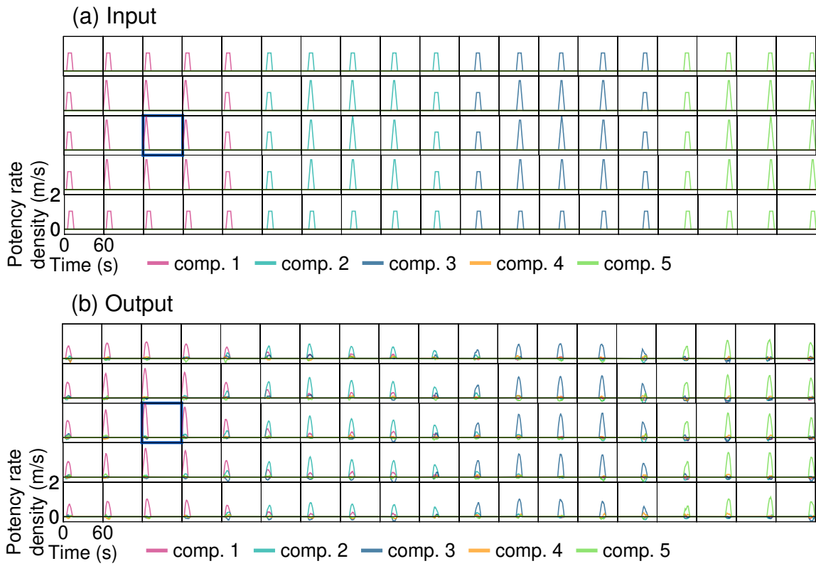
Figure S6. (a) Input and (b) output potency-rate-density functions on an assumed model fault in the case 3. The sub-fault outlined by blue line shows the initial rupture point. Potency-rate-density functions for all basis double-couple components are represented as different colour traces.
