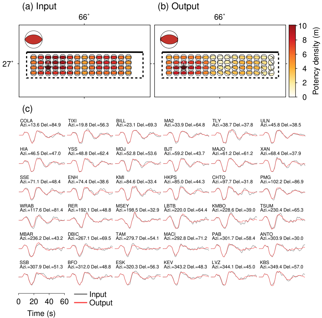
Figure S3. (a) Input source model, (b) Output source model, and (c) waveform fitting at all stations between input and output synthetic waveforms in the case 2. (a, b) The beach ball colour shows the potency density. The dashed line outlines the model fault, and the bold black line shows the top of the model fault, respectively. The star denotes the epicentre. The large red beach ball represents the total moment tensor obtained by taking a spatial integration of the potency-density tensors. (c) The waveforms are plotted with a sampling interval of 0.05 s. Station code, azimuth, and epicentral distance are shown above the traces.
