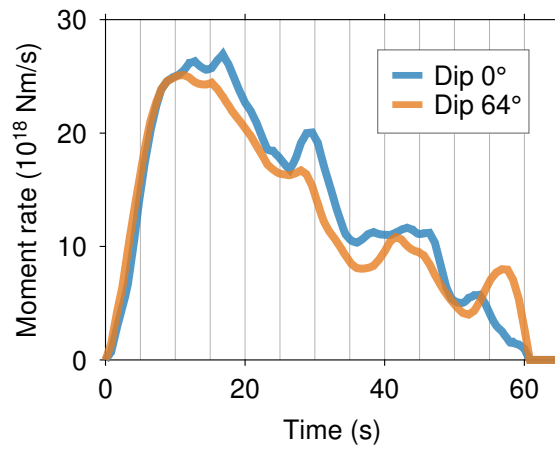
Figure S14. Moment-rate functions for the model planes dipping 0° (blue line) and 64° (orange line).
