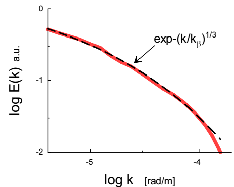
FIG. 9: Perturbation kinetic energy spectrum (ensemble- and meridional-averaged for the 25 Dec 2010 snowstorm) at 36 hours of the lead time.
