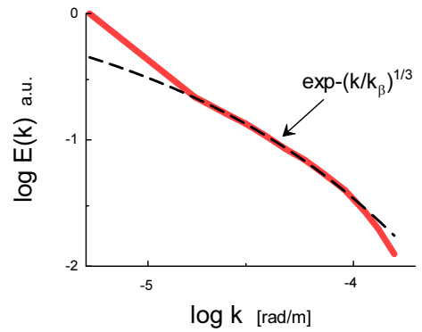
FIG. 8: Background kinetic energy spectrum (ensemble- and meridional-averaged) for the 25 Dec 2010 snowstorm.
