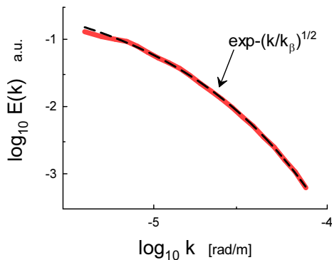
FIG. 11: Spectrum of the kinetic energy of the perturbations about the ensemble mean at the 36 hours of the lead time for the 17 Dec 2008 snowstorm.
