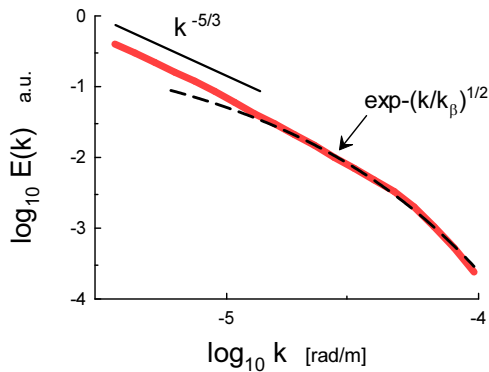
FIG. 10: Average of the horizontal kinetic energy spectra at 700-hPa at 1200 UTC 17 Dec 2008.
