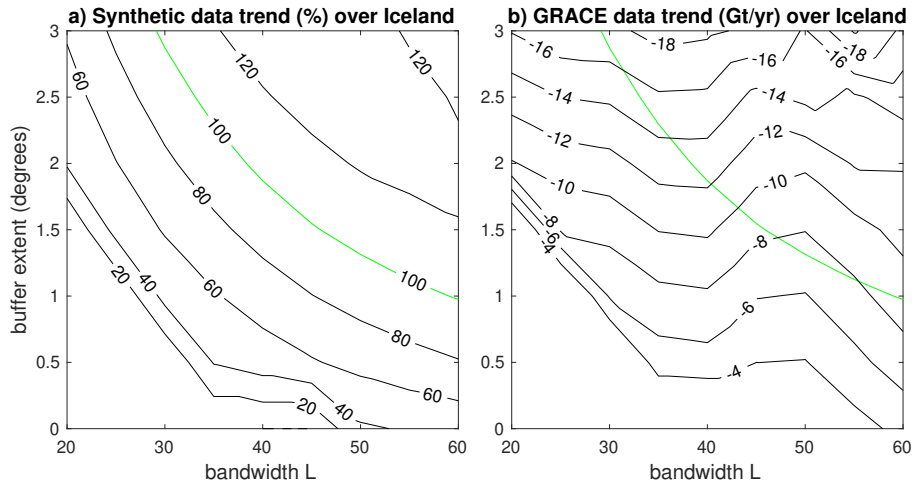
Figure 2. a) Synthetic trend recovery over Iceland. The contours represent the percent signal recovered from the synthetic data for each choice of buffer and bandwidth. b) Real trend recovery over Iceland. The contours represent the actual trend estimates calculated from GRACE data for each choice of buffer and bandwidth. The 100% recovery contour from a) is shown in green. For the bandwidth of the data ( L = 60 ), the 100% recovery contour closely aligns with the choice of a 1.0^\circ buffer around Iceland.
