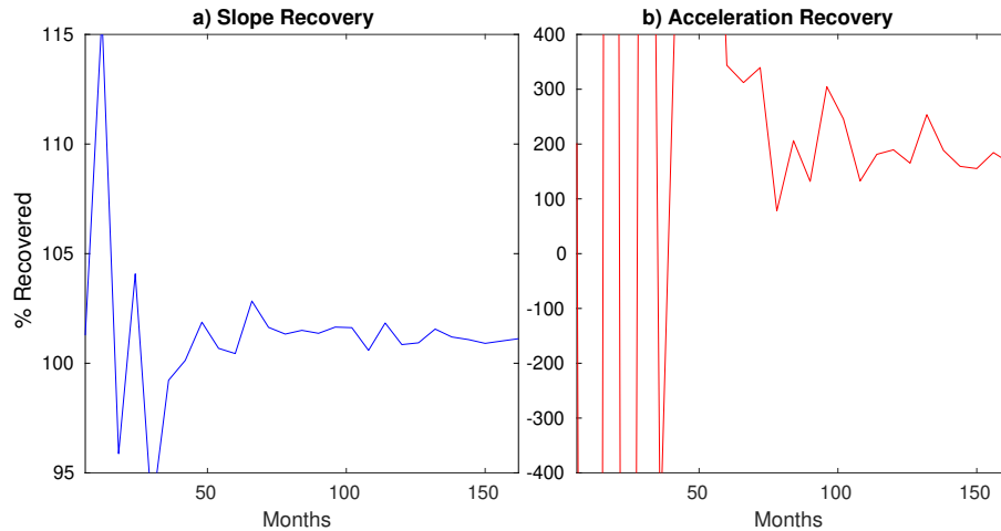
Figure 6. Results of our synthetic experiment for Iceland to test recovery of a) slope and b) acceleration parameters. For varying amounts of months of consistent synthetic data over Iceland we use our Slepian method to measure the slope and acceleration of the mass loss trend. The x -axis denotes the number of cumulative months of synthetic data processed, and the y -axis denotes the 100 * \frac{R}{A} , where R is the recovered slope or acceleration and A is the applied synthetic slope or acceleration.
