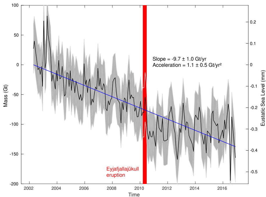
Figure 3. GRACE-derived mass loss trend over Iceland. The black line indicates the total integrated monthly mass change since 2002 (gigatons left axis and equivalent eustatic sea level change, right axis), and the gray shaded region is its \pm 2\sigma uncertainty interval. The blue line is the best-fit linear equation over the entire timespan. The red strip highlights the time period of the Eyjafjallajökull volcanic eruption.
