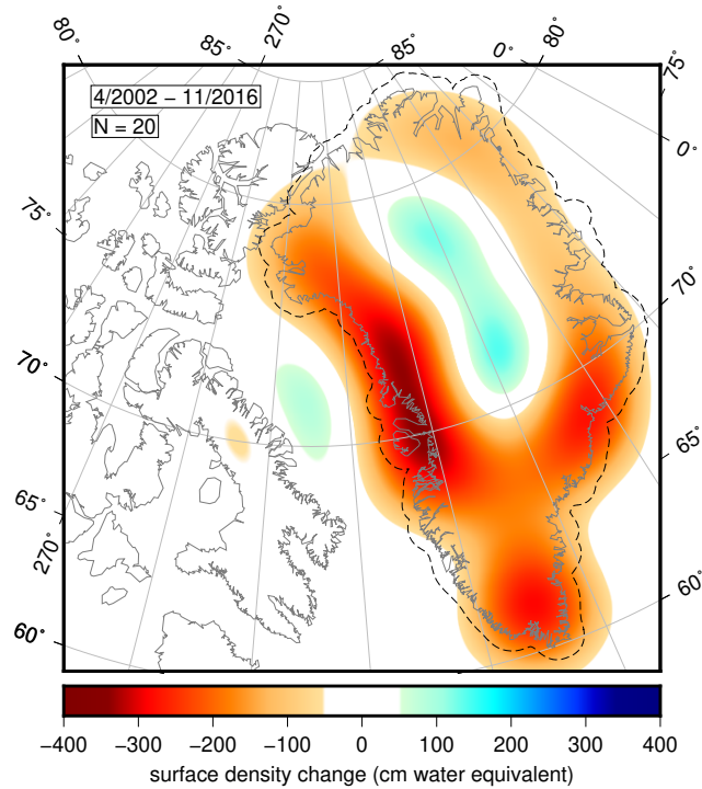
Figure 4. Geographic pattern of mass change over Greenland, shown in centimeters water equivalent. The dashed line around Greenland is its 0.5^\circ buffer. The figure represents the total mass change over the date range specified in the top left. Below the date range is the Shannon number N = 20 for the buffered region and bandwidth of 60, indicating that the figure represents the sum of 20 optimal Slepian functions.
