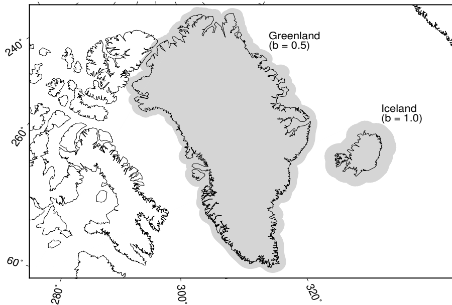
Figure 1. A map of the localization regions used for Greenland and Iceland. The gray areas represent the region of Greenland buffered by 0.5^\circ and the region of Iceland buffered by 1.0^\circ , respectively. We use an oblique mercator projection centered in Greenland.
