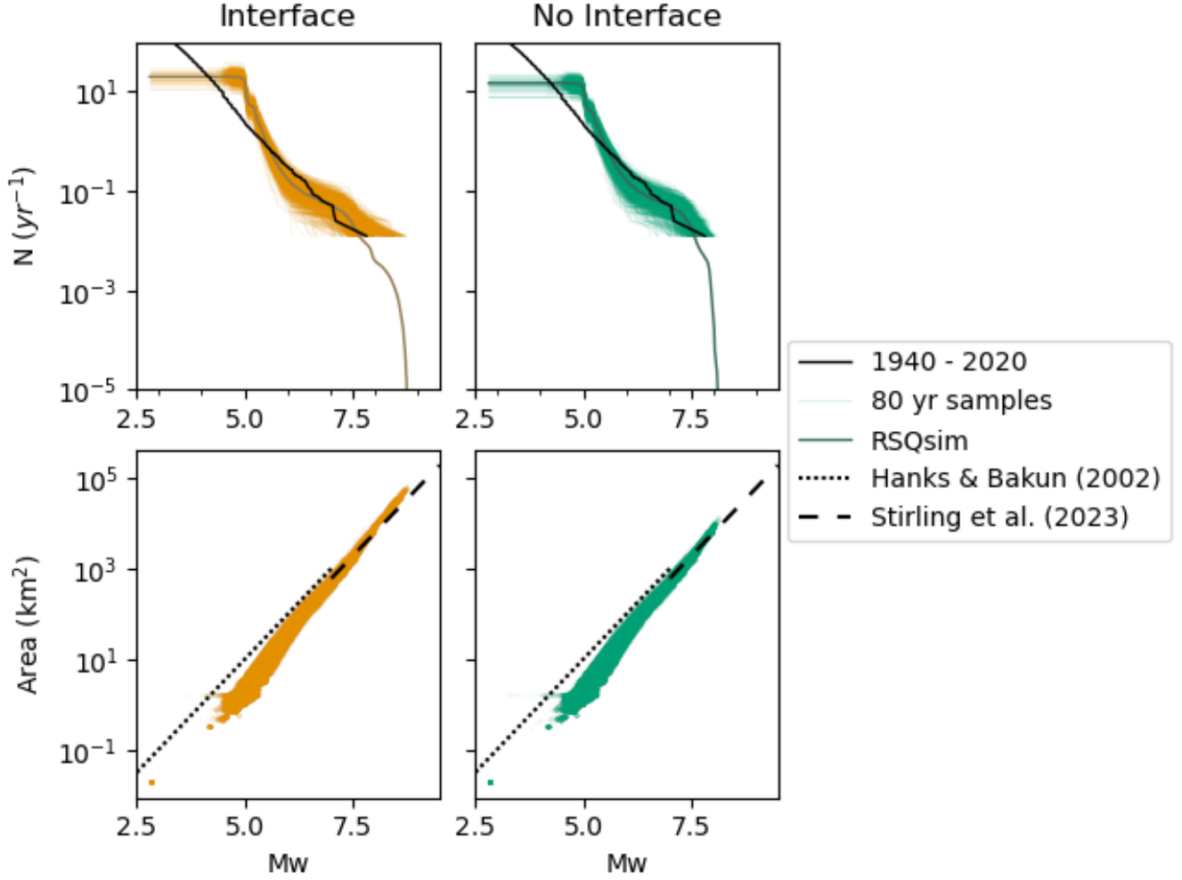
Figure 4: Scaling relationships for RSQsim catalogues (left - with the subduction interface, right - without the subduction interface). Top panels show magnitude-frequency distributions for 80 year samples from these catalogues (bright colours) and the whole catalogue (darker colours). The instrumental record, from Rollins et al. (2024), is plotted in black. Bottom panels show the magnitude - area scaling for events in each catalogue. Dotted black line is the scaling relationship proposed by Hanks (2002), and dashed black line is that proposed by Stirling et al. (2023), for M_w > 8 and used in the New Zealand National Seismic Hazard Model 2022 (Gerstenberger et al., 2024a).
