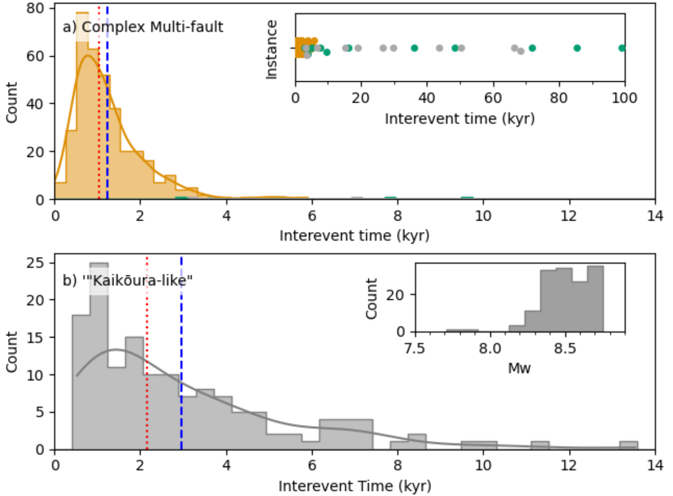
Figure 6: Interevent times for a) complex multi-fault synthetic earthquakes ( M_w > 7.5 , involving \geq 4 faults within 1.5 magnitude units of the highest moment release fault, section 3.4, defined to capture key features of the Kaikōura earthquake). Counts are dominated by earthquakes which involve the subduction interface ( n=357 , orange histogram and kernel density estimate plot) which have a mean interevent time of 1.2 kyr and a coefficient of variation of 0.66. Complex multi-fault events which involve only crustal faults are shown in green ('Interface' catalogue) and grey ('No Interface' catalogue). Inset panel shows the time between events of each type for longer interevent times (up to 100 kyr), which are typically for events not involving the subduction interface, whereas the maximum interevent time for a complex multi-fault earthquake involving the subduction interface is \sim 6 kyr. Note that because these plots are for a class of earthquakes, not events on a particular fault, the interevent times are not directly comparable to paleoseismic interevent times on a single fault. b) shows the interevent time distribution for the subset of complex multi-fault event which have moment release equivalent to at least M_w 7 on the Jordan-Kekerengu-Needles (JKN) fault, which we term 'Kaikōura-like'. The inset shows the distribution of magnitudes for such 'Kaikōura-like' earthquakes. Blue and red lines in a) and b) show the mean and median interevent times respectively.
