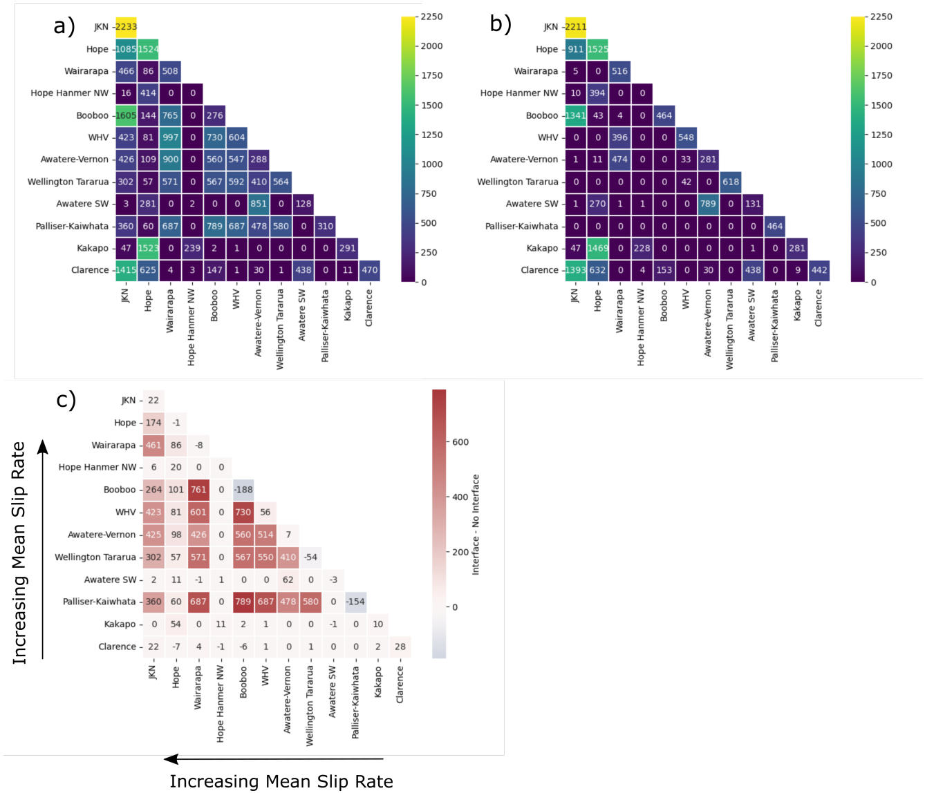
Figure 7: Occurrences of co-ruptures on high slip rate faults. a) and b) show the number of co-ruptures of faults in the ‘Interface’ and ‘No Interface’ models, respectively. Diagonal squares show the number of single fault earthquakes on each fault. Catalogues are filtered to synthetic earthquakes with M_w > 6.5 . Note that because some earthquakes involve more than two faults, the sum of the numbers across the whole heat map is greater than the total number of synthetic earthquakes with M_w > 6.5 in each catalogue. c) shows the difference in the number of co-ruptures between these two models (‘Interface’ - ‘No Interface’, i.e. a)-b)). The diagonal squares show the change in the number of single-fault earthquakes on that fault between the two models.
