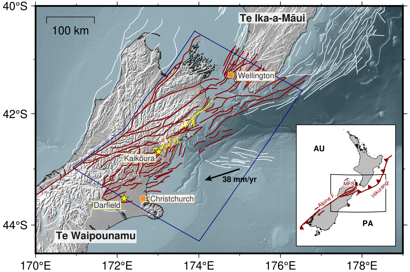
Figure 1: Map of the study area, which spans the northern South Island | Te Waipounamu and southern North Island | Te Ika-a-Māui of A-NZ. Fault traces from the New Zealand Community Fault Model (Seebeck et al., 2022, 2023) are shown in white, whilst those used in our modelling are shown in red. The faults used are those within, or which intersect, the blue box. We exclude faults with reported slip rates of 0 \text{ mm yr}^{-1} , except those which are thought to have ruptured in the Kaikōura earthquake (e.g. the Offshore Splay Thrust Fault, Mouslopoulou et al., 2019; Nicol et al., 2023). Surfaces ruptures from this earthquake (downloaded from https://data.gns.cri.nz/af/ , last accessed 4/12/25) are shown in yellow, which extend from The Humps fault (the epicentre of the earthquake, shown by the yellow star labelled Kaikōura) to the Needles fault in the north east. The plate motion vector is taken from DeMets et al. (2010). HF is the Hope Fault. Yellow star on the edge of the blue box shows the epicentre of the 2010 Darfield earthquake. Inset shows the overall tectonics of A-NZ, on the boundary between the Pacific (PA) and Australian (AU) plates, transitioning from the Hikurangi subduction zone in the north-east, through the Marlborough fault zone (MFS) to the Alpine Fault and the Puysegur subduction zone in the south-west. Black box shows the location of the main figure.
