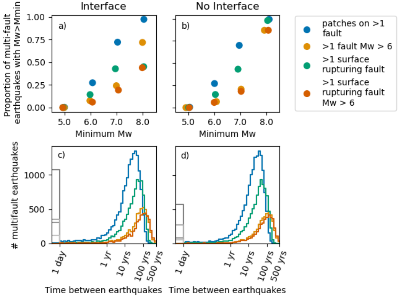
Figure 5: Effects of choosing different definitions of ‘multi-fault’ on the proportion of multi-fault earthquakes in catalogues with (left panels) and without (right) the subduction interface. Top panels show the proportion of multi-fault earthquakes with M_w > M_w^{min} using different definitions. Bottom panels show histograms of the times between multi-fault events with M_w > 7 using these different definitions.
