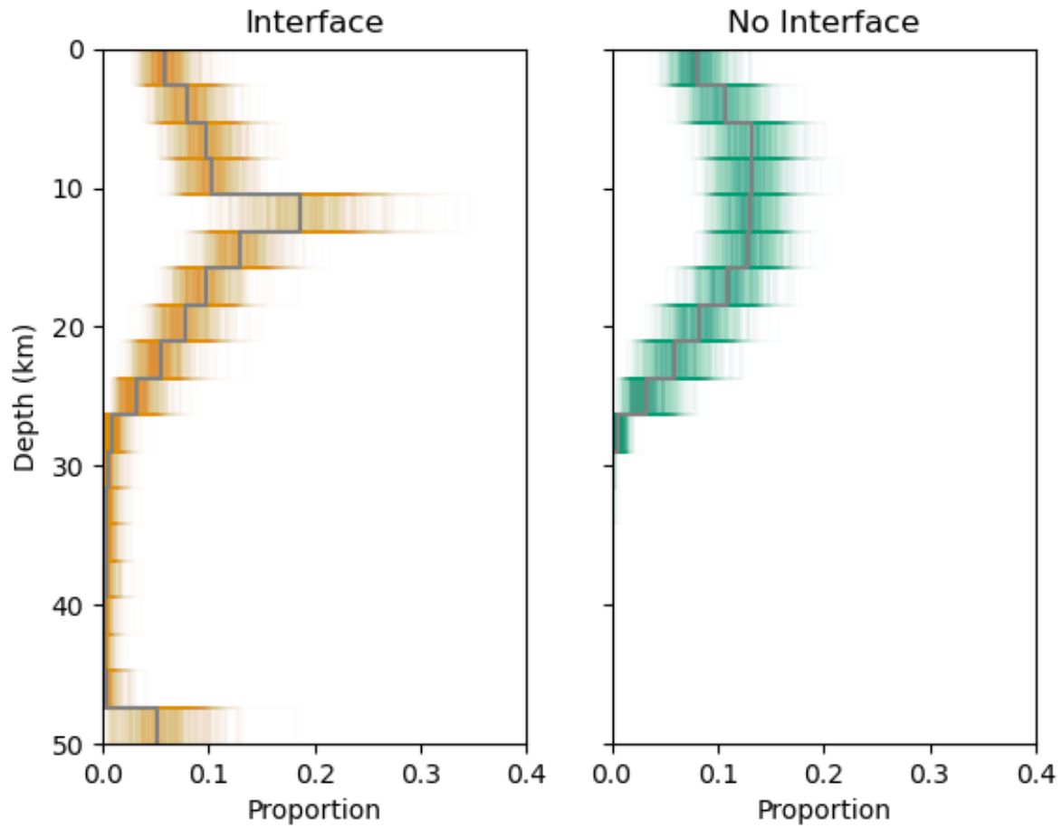
Figure 3: Depth histograms for RSQsim catalogues (left - with the subduction interface, right - without the subduction interface). Coloured lines show depths from 1000 80 year time windows in each catalogue, grey lines show the whole catalogue.
