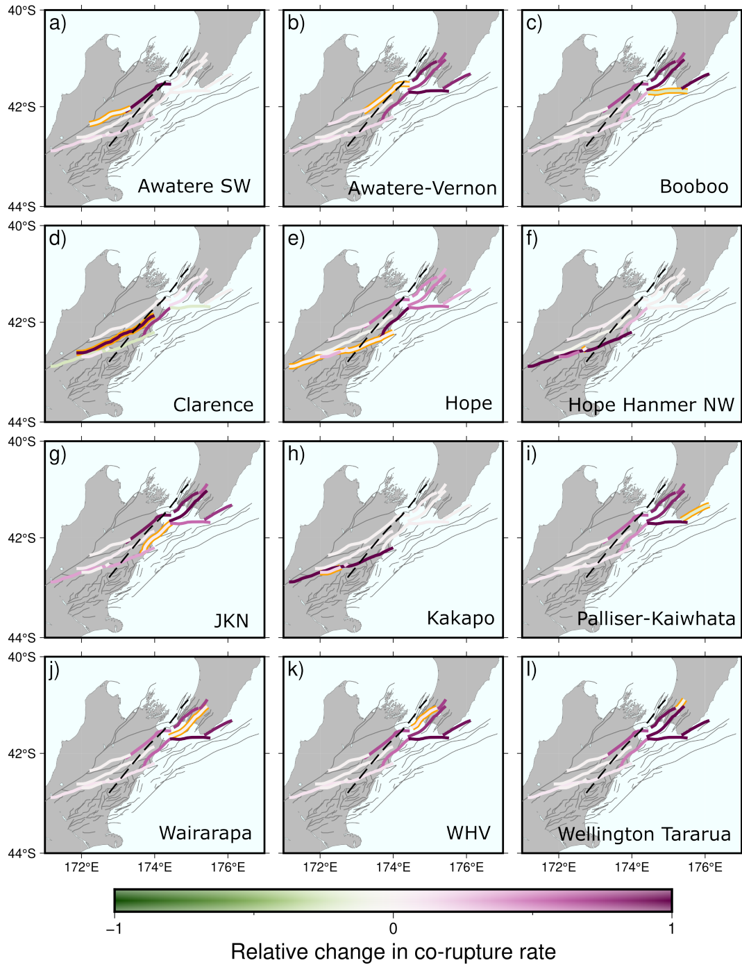
Figure 8: Relative occurrence of co-ruptures on high slip rate faults between our two simulations. This figure is a geographical representation of the information in figure 7. The rate is the normalised difference ( \text{'Interface'} - \text{'No Interface'} / \text{maximum difference for that primary fault} ) in the number of synthetic earthquakes involving both the primary fault (highlighted in orange) and each other fault. Purple colours imply more events rupture both that fault and the primary fault in the 'Interface' than the 'No Interface' model. The colour of the primary fault reflects the change in single fault ruptures on that fault. Dashed line shows the 30km contour from the interface model of Williams et al. (2013) – we expect this contour to form an approximate dividing line with crustal faults up-dip (South-East) of this line interacting with the interface, whilst those to the North-West do not. Primary faults: a) Awatere South West, b) Awatere-Vernon, c) Boo Boo, d) Clarence, e) Hope, f) Hope Hanmer North West, g) Jordan-Kekerengu-Needles, h) Kakapo, i) Palliser-Kaiwhata, j) Wairarapa, k) Wellington Hutt Valley, l) Wellington Tararua.
