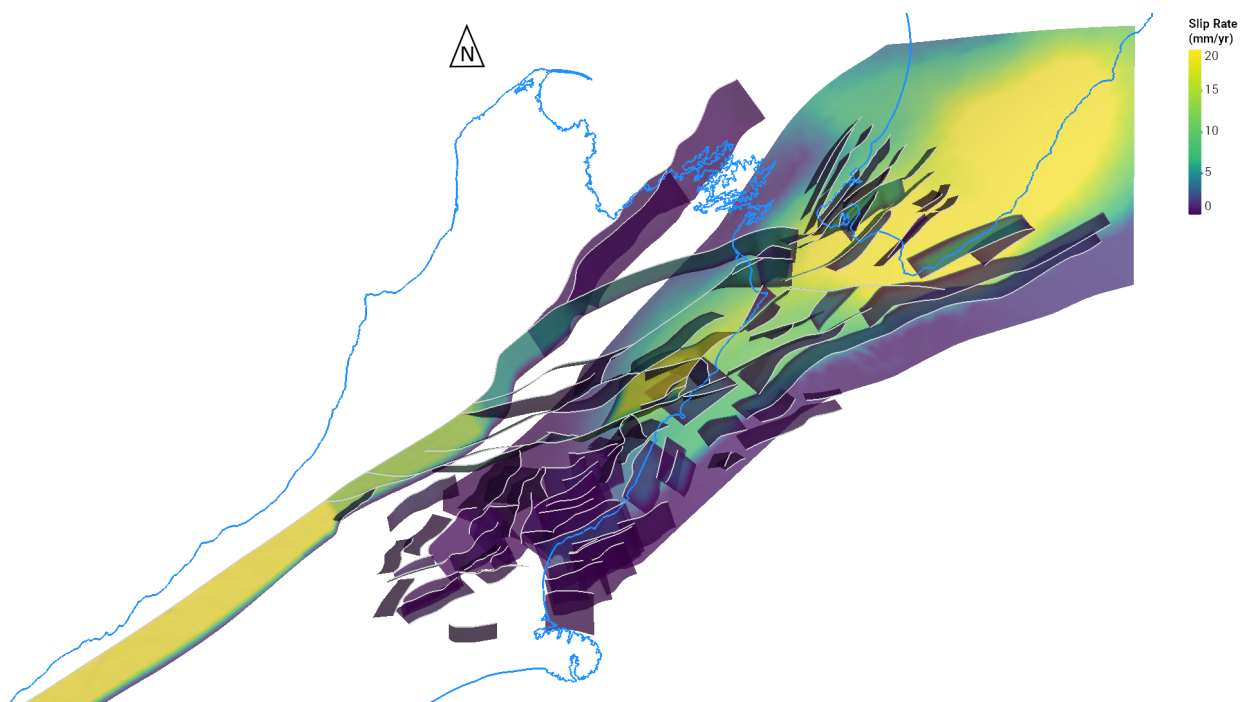
Figure 2: 3D fault model of Central A-NZ coloured by slip rate. The study area is shown by the box in Figure 1.
