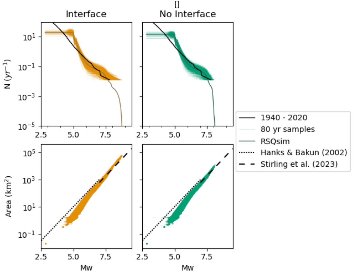
Figure 4. Scaling relationships for RSQsim catalogues (left - with the subduction interface, right - without the subduction interface). Top panels show magnitude-frequency distributions for 80 year samples from these catalogues (bright colours) and the whole catalogue (darker colours). The instrumental record, from Rollins et al. (2024), is plotted in black. Bottom panels show the magnitude - area scaling for events in each catalogue. Dotted black line is the scaling relationship proposed by Hanks (2002), and dashed black line is that proposed by Stirling et al. (2023), for M_w > 8 and used in the New Zealand National Seismic Hazard Model 2022 (Gerstenberger et al., 2024a).
