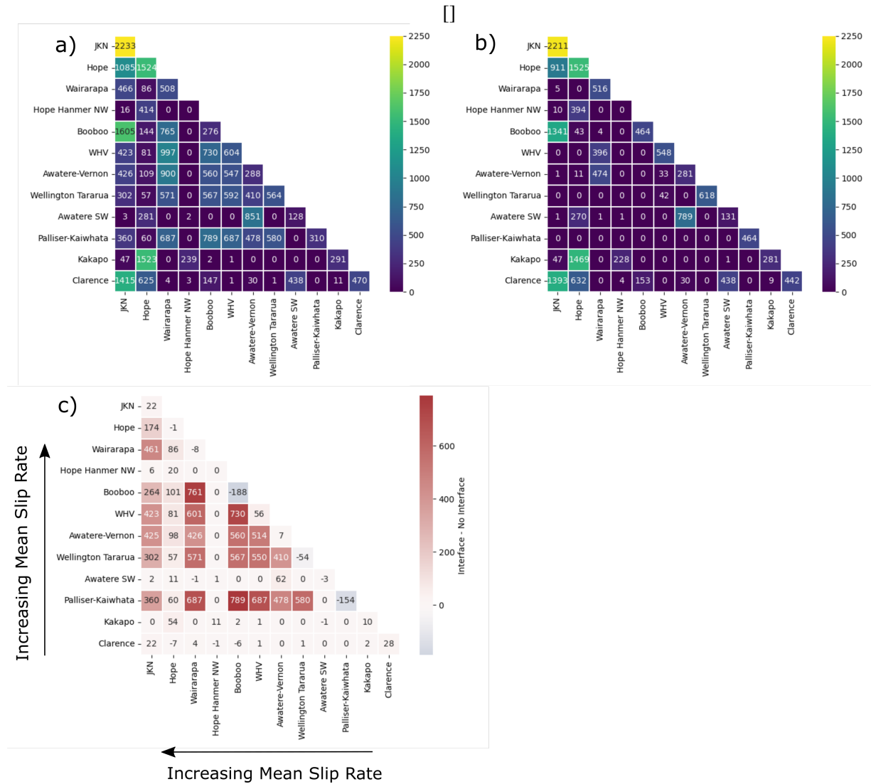
Figure 7. Occurrences of co-ruptures on high slip rate faults. a) and b) show the number of co-ruptures of faults in the ‘Interface’ and ‘No Interface’ models, respectively. Diagonal squares show the number of single fault earthquakes on each fault. Catalogues are filtered to synthetic earthquakes with M_w > 6.5 . Note that because some earthquakes involve more than two faults, the sum of the numbers across the whole heat map is greater than the total number of synthetic earthquakes with M_w > 6.5 in each catalogue. c) shows the difference in the number of co-ruptures between these two models (‘Interface’-‘No Interface’, i.e. a)-b)). The diagonal squares show the change in the number of single-fault earthquakes on that fault between the two models.
