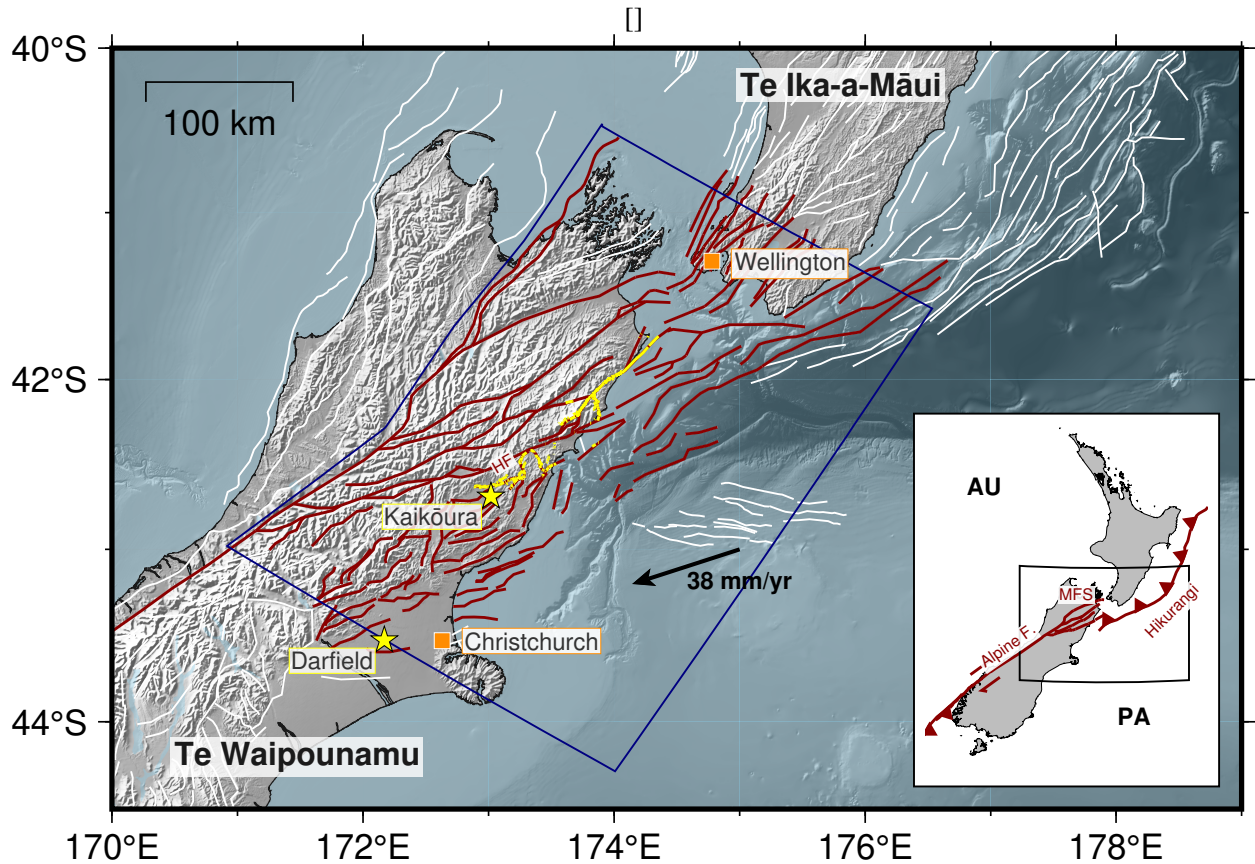
Figure 1. Map of the study area, which spans the northern South Island | Te Waipounamu and southern North Island | Te Ika-a-Māui of A-NZ. Fault traces from the New Zealand Community Fault Model (Seebeck et al., 2022, 2023) are shown in white, whilst those used in our modelling are shown in red. The faults used are those within, or which intersect, the blue box. We exclude faults with reported slip rates of 0 \text{ mm yr}^{-1} , except those which are thought to have ruptured in the Kaikōura earthquake (e.g. the Offshore Splay Thrust Fault, Mouslopoulou et al., 2019; Nicol et al., 2023). Surface ruptures from this earthquake (downloaded from https://data.gns.cri.nz/af/ , last accessed 4/12/25) are shown in yellow, which extend from The Humps fault (the epicentre of the earthquake, shown by the yellow star labelled Kaikōura) to the Needles fault in the north east. The plate motion vector is taken from DeMets et al. (2010). HF is the Hope Fault. Yellow star on the edge of the blue box shows the epicentre of the 2010 Darfield earthquake. Inset shows the overall tectonics of A-NZ, on the boundary between the Pacific (PA) and Australian (AU) plates, transitioning from the Hikurangi subduction zone in the north-east, through the Marlborough fault zone (MFS) to the Alpine Fault and the Puysegur subduction zone in the south-west. Black box shows the location of the main figure.
