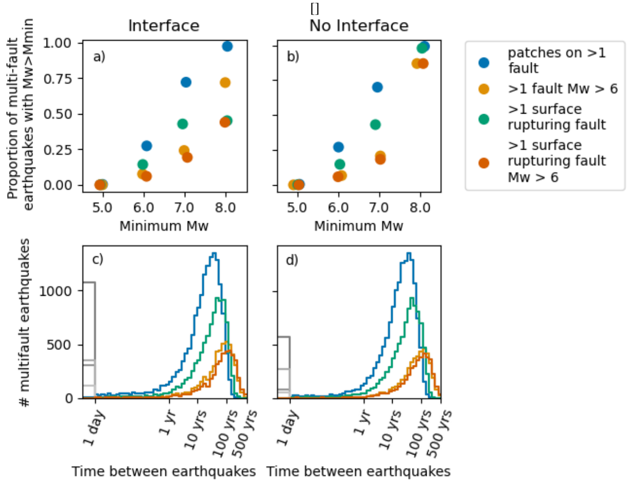
Figure 5. Effects of choosing different definitions of ‘multi-fault’ on the proportion of multi-fault earthquakes in catalogues with (left panels) and without (right) the subduction interface. Top panels show the proportion of multi-fault earthquakes with M_w > M_w^{min} using different definitions. Bottom panels show histograms of the times between multi-fault events with M_w > 7 using these different definitions.
