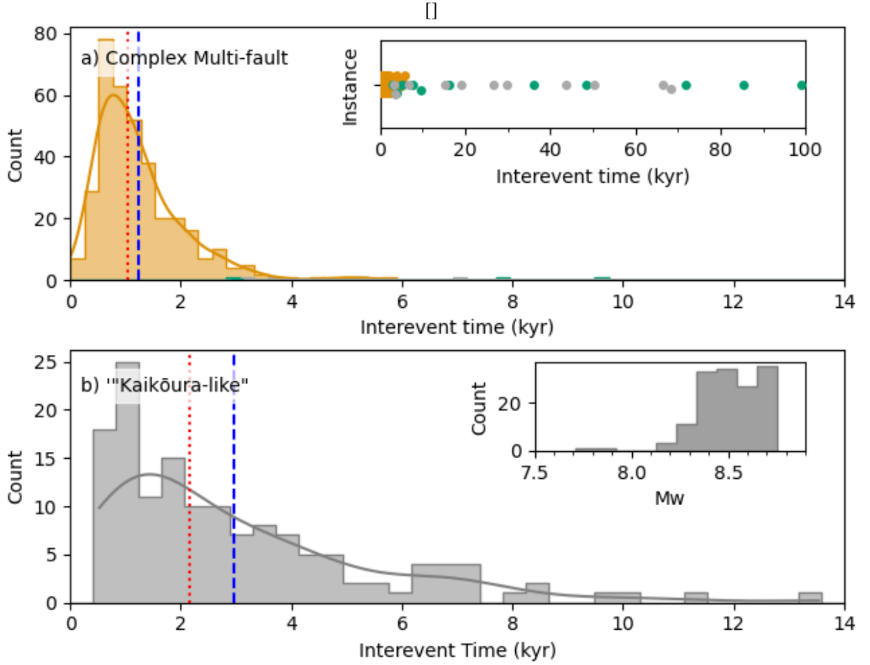
Figure 6. Interevent times for a) complex multi-fault synthetic earthquakes ( M_w > 7.5 , involving \geq 4 faults within 1.5 magnitude units of the highest moment release fault, section 3.4, defined to capture key features of the Kaikōura earthquake). Counts are dominated by earthquakes which involve the subduction interface ( n=357 , orange histogram and kernel density estimate plot) which have a mean interevent time of 1.2 kyr and a coefficient of variation of 0.66. Complex multi-fault events which involve only crustal faults are shown in green ('Interface' catalogue) and grey ('No Interface' catalogue). Inset panel shows the time between events of each type for longer interevent times (up to 100 kyr), which are typically for events not involving the subduction interface, whereas the maximum interevent time for a complex multi-fault earthquake involving the subduction interface is \sim 6 kyr. Note that because these plots are for a class of earthquakes, not events on a particular fault, the interevent times are not directly comparable to paleoseismic interevent times on a single fault. b) shows the interevent time distribution for the subset of complex multi-fault event which have moment release equivalent to at least M_w 7 on the Jordan-Kekerengu-Needles (JKN) fault, which we term 'Kaikōura-like'. The inset shows the distribution of magnitudes for such 'Kaikōura-like' earthquakes. Blue and red lines in a) and b) show the mean and median interevent times respectively. ALT-TEXT: Two panels each show a histogram with a KDE plot overlaid. Plots are of count against interevent time.
