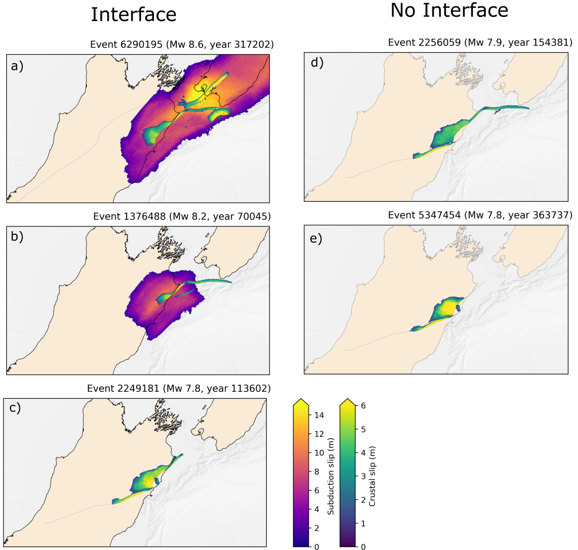
Figure 10. Examples of ‘Kaikōura-like’ earthquakes from the ‘Interface’ (a, b, c) and ‘No Interface’ catalogues (d, e). c) shows a rare (n=2) Kaikōura-like event in the ‘Interface’ catalogue which does not involve the subduction interface.
