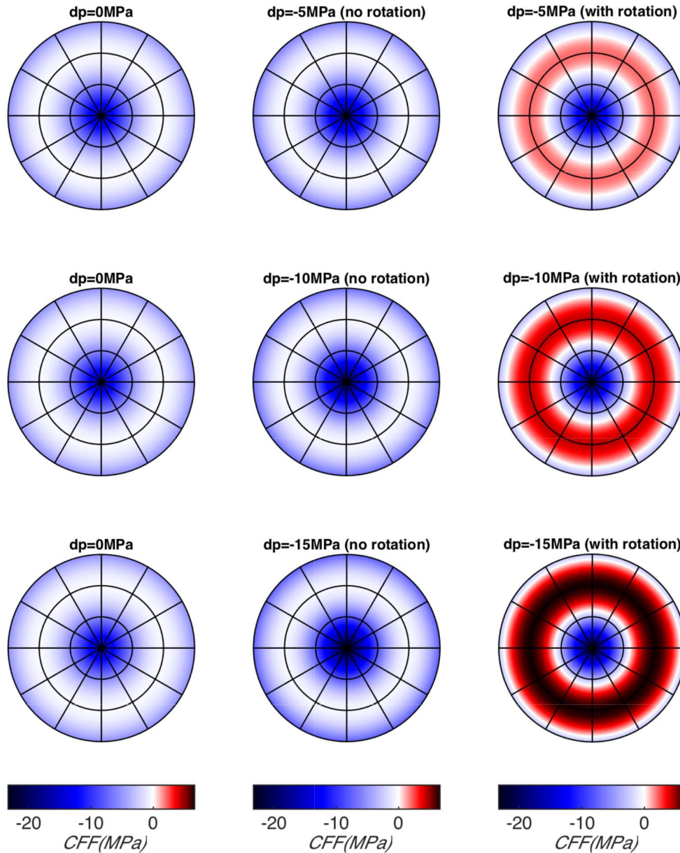
Figure 5: Changes of the Coulomb Failure Functions. Left: Before depletion; middle: after depletion without rotation (depletion occurs on both sides of the fault); right: after depletion with rotation (depletion occurs on one side of the fault). Pore pressure depletions are -5MPa (upper), -10MPa (middle) and -15 MPa (lower). Blue indicates the orientation of a stable fault, while red indicates the orientation of a fault that will be induced to slip due to depletion. All
