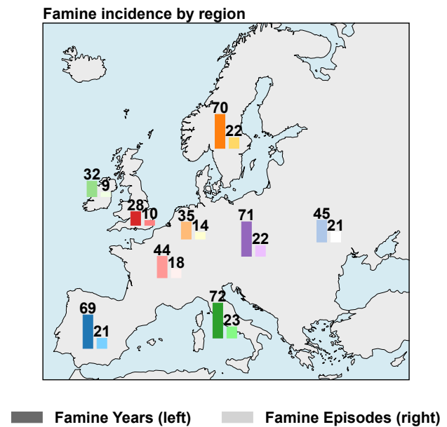
Figure 1: ENSO and famines in Early Modern Europe. (A) ENSO index (NINO3.4 Region boreal winter SST anomalies relative to the 1801–1900 mean), with extreme values (red dots > 1°C) overlain by key societal crises (pink: 1590s and 1690s Catastrophic Famines; blue: Famines in Central Europe; purple: 1647–1652 Europe-wide Famines). (B) The top panel presents famine episodes across different regions. Each horizontal bar represents a continuous famine episode within a given region, spanning from the estimated onset year to its termination. The bottom panel shows the annual number of concurrent famine years aggregated across all regions. (C) Map of all nine regions covered by the Ljungqvist et al. [7] famine data. Number of famine episodes (right bars) and total years spent in famines (left bars) within each region (bars located in the center of each region).
