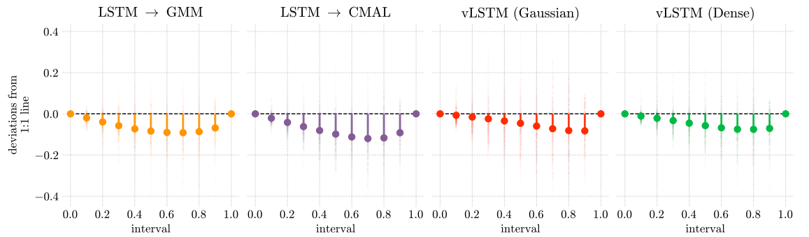
Figure 12. Calibration plot based on the PICP method shown as the deviation from the 1:1 line using lollipops. Background markers represent individual coverage at each interval for each marker, while the foreground lollipop shows the mean coverage across all basins.
