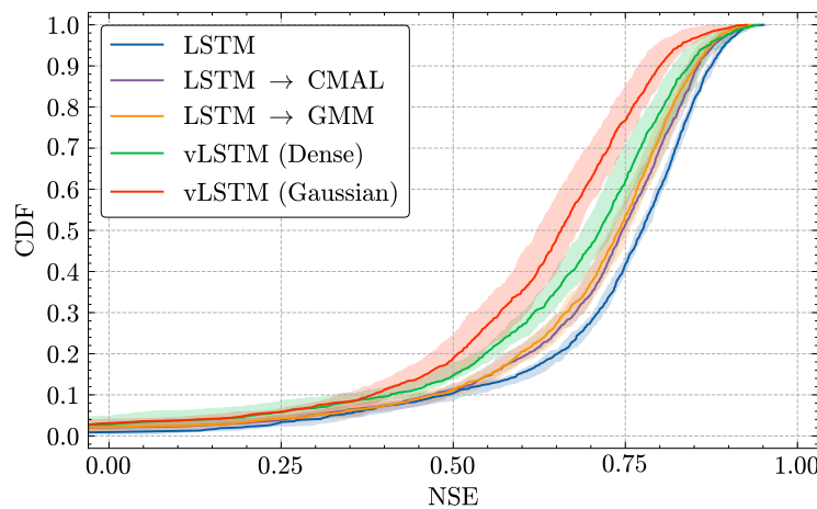
Figure 8. Cumulative NSE distribution for the testing set. NSE is calculated for each basin in the testing set and the result for each basin is accumulated along the x-axis. The solid line represents the median for each model and a 95% interval is shown representing the variability in the result due to random initialization of the model.
