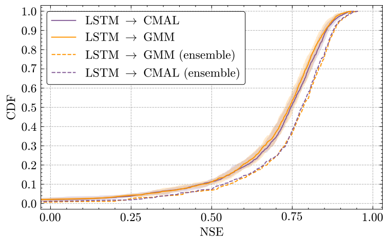
Figure 17. Comparison of the MDN models shown in the main manuscript with the original benchmark.
