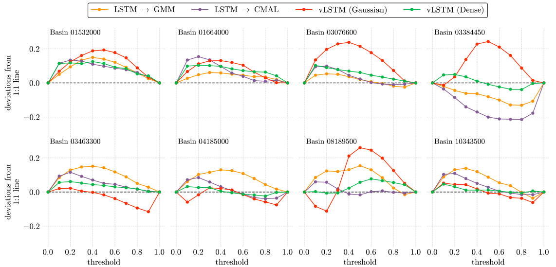
Figure 11. Calibration plots based on the PIT method shown as deviations from the 1:1 line for individual basins, illustrating model behavior across different hydrological regimes.
