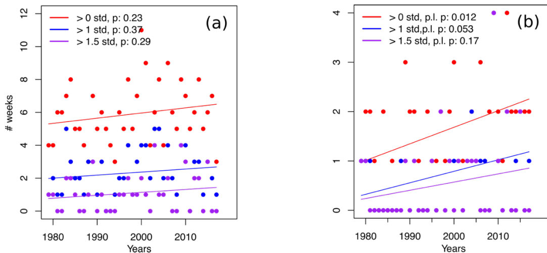
Figure 4. Recent trends in the occurrence of the wave-7 teleconnection. (a) Number of weeks per summer season (JJA, 1979-2017) with wave-7 amplitude above average (>0 \sigma ), 1 \sigma and 1.5 \sigma irrespective of phase position. (b) Number of weeks per summer season (JJA) where wave-7 is in its preferred phase position (see Fig. S4) and the amplitude of wave-7 is above average (>0 \sigma ), >1 \sigma and >1.5 \sigma .
