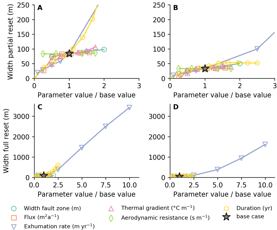
Figure DR6: Sensitivity of the size of the zone adjacent to one side of the hydrothermally active normal fault where AHe ages are partially reset. The analysis was performed for six parameters: duration, fluid flux, fault damage zone width, background thermal gradient, aerodynamic resistance and exhumation rate. For each line in the graph, one parameter was changed while all other parameters were set to their base values. Base values (star) are 400 \text{ m}^2 \text{ a}^{-1} for the fluid flux, 10 \text{ m} for the fault damage zone, 0.04 \text{ }^\circ\text{C m}^{-1} for the thermal gradient and 1 \times 10^{-4} \text{ m a}^{-1} for the exhumation rate. Lateral flow in shallow layers connected to the fault was not taken into account. The most sensitive parameter is exhumation rate. An increase in exhumation rates leads to an exponential growth of the partial reset zone. The sensitivity for fluid flux, thermal gradient and fault damage zone are in a similar order of magnitude. Fluid flux and thermal gradient are more sensitive for small values and less sensitive for larger values. Fault damage zone and aerodynamic resistance are the least sensitive parameters.
