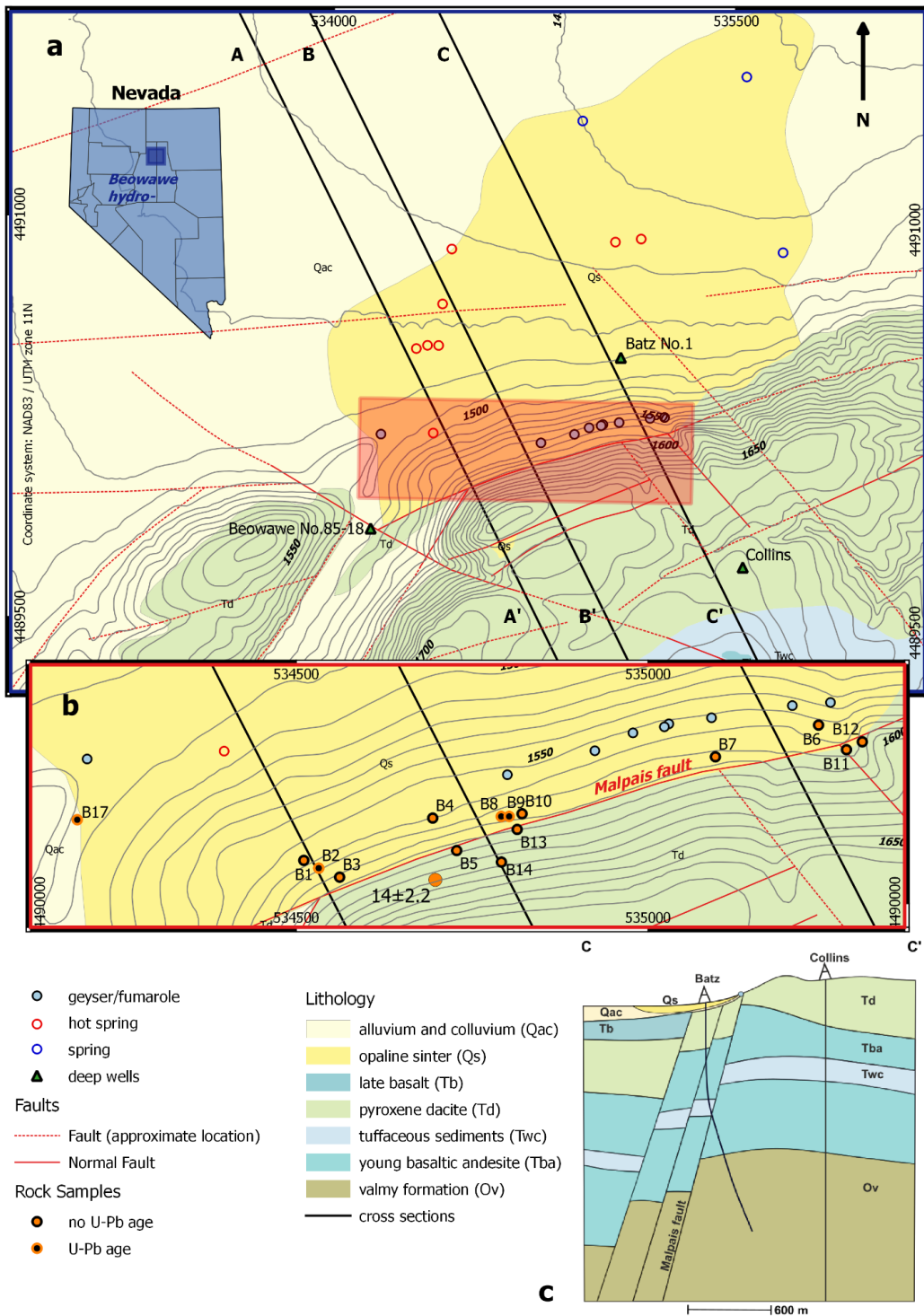
Figure DR1 (a) Geological map of the Beowawe geothermal area, locations of wells and the geysers and hot springs that were active prior to geothermal development in the 1960s. (b) Close-up of the hydrothermally active Malpais fault and the AHe and U-Pb sample locations. (c) Geologic cross-section showing the Batz and Collins wells relative to the Malpais fault zone. t
