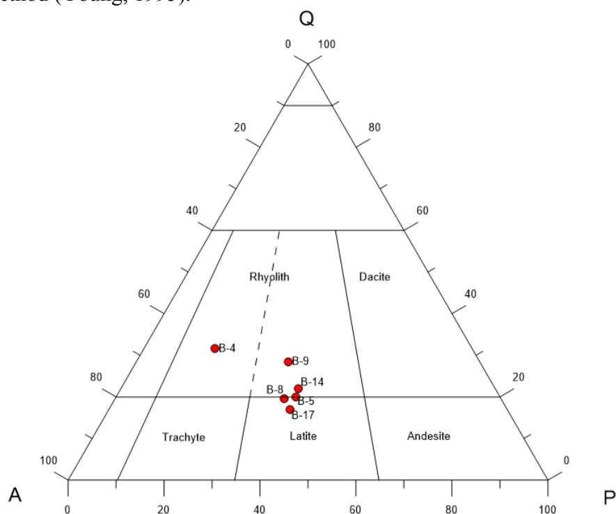
Figure DR3 Streckeisen diagram showing the total weight percentage of all quartz, potassium feldspar and plagioclase mineral phases in the analyzed samples.
