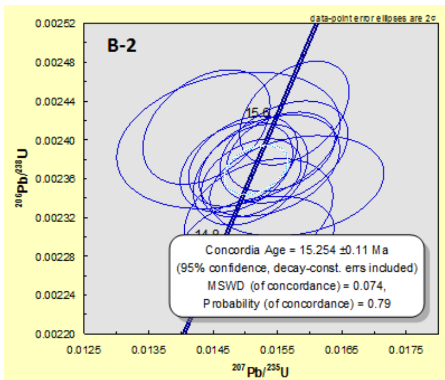
Figure DR5 Concordia plots of U-Pb age of samples B-2, B-8 and B-9
