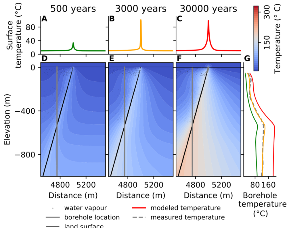
Figure 2. Comparison of modeled temperatures over time and borehole temperature record for borehole 85-18 indicates that fluid flow in this section of the fault is around 3000 years old (panel G). Panels A, B, and C show the surface temperature over time, panels D, E and F show the modeled temperature field and the location of the borehole. The measured borehole temperature data and the modeled temperatures for three time-slices are shown in panel G.
