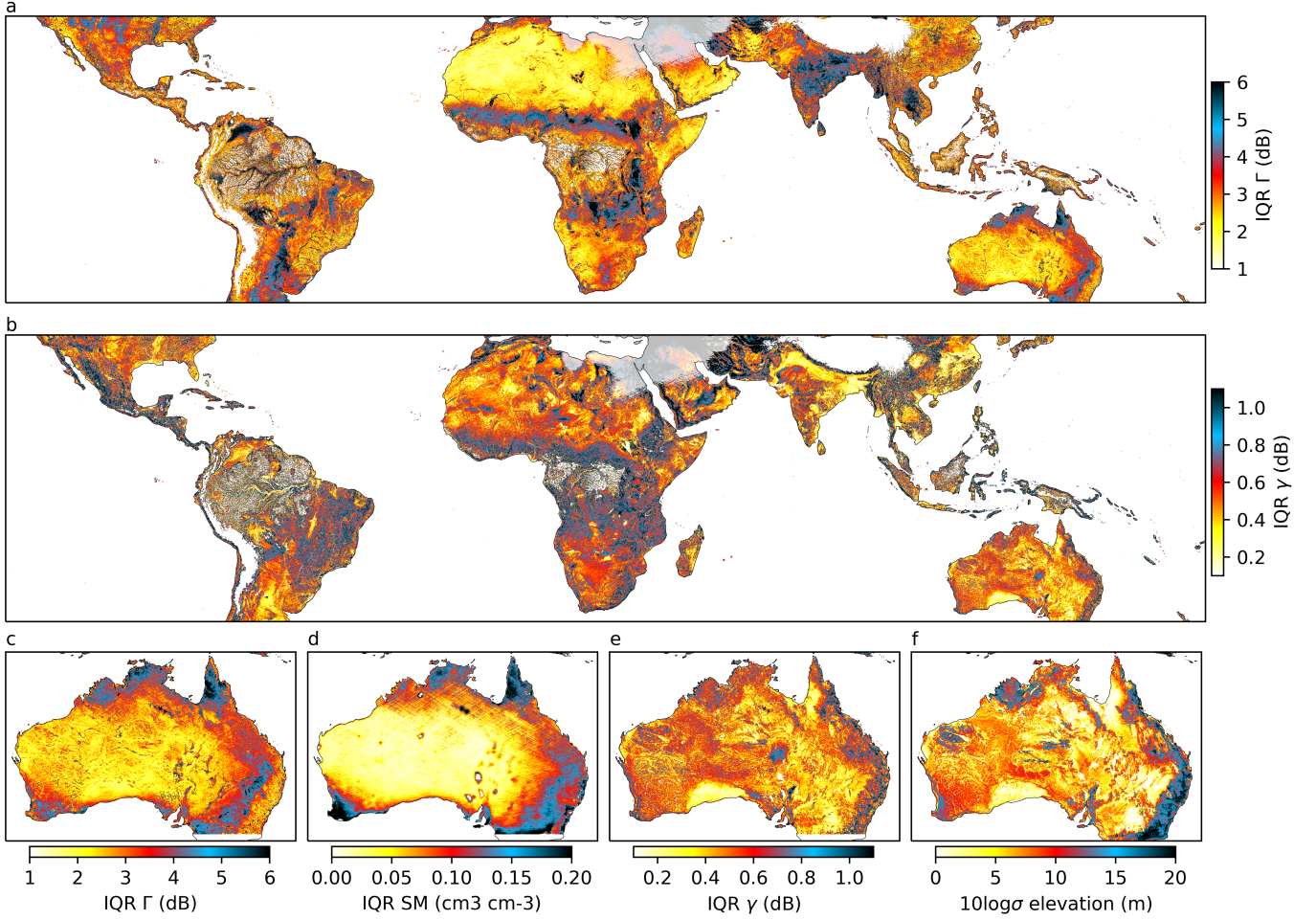
Fig. 5. Inter-quartile ranges (IQR) for \Gamma (a) and \gamma (b) calculated using observations between 2020 - 2024. Regions exceeding 3000 m surface elevation have been masked out, and regions in the Middle East that commonly experience RFI are semi-transparent. (c) Same as (a) but only for Australia. (d) IQR of soil moisture for 2020 - 2024 for Australia. (e) Same as (b) but only for Australia. (f) The standard deviation of elevation within each 3 km grid cell for Australia, in dB.
