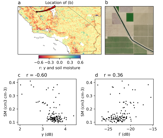
Fig. 7. (a) Same as Figure 6c, but focused on California below 38 degrees latitude. The red arrow indicates the location of the pixel in (b). (b) A Sentinel-2 image of a 3 x 3 km pixel where \gamma and soil moisture are negatively correlated. The California aqueduct bisects the pixel. Modified Copernicus Sentinel data [2024] processed by the Copernicus Browser. (c) Relationship between \gamma and soil moisture for the pixel. (d) Relationship between \Gamma and soil moisture for the same pixel.
