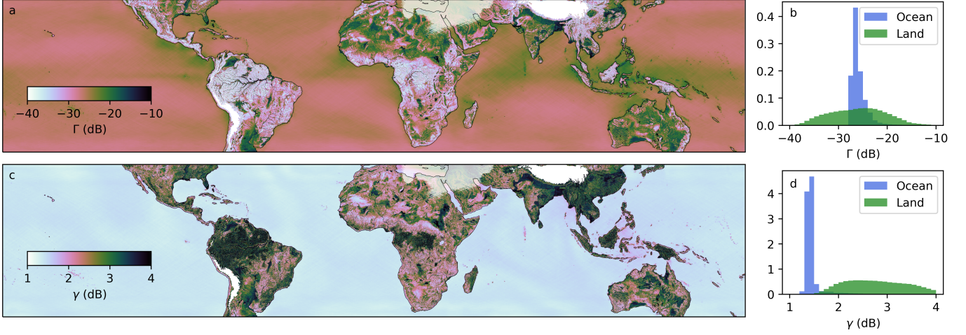
Fig. 3. (a) Long term average (2020 – 2024) of CYGNSS surface \Gamma . Observations over the ocean were gridded to 36 km, and observations over the land surface were gridded to 3 km. (b) Distributions of (a) binned by land and ocean. (c) Long term average (2020 – 2024) of \gamma . (d) Distributions of (c) binned by land and ocean. In panels (a) and (c), regions with surface elevation in excess of 3000 m have been removed (i.e., Tibetan Plateau and the Andes Mountains), and regions that experience significant RFI in the Middle East are semi-transparent. CYGNSS data are constrained to \pm 38 degrees latitude due to its orbital inclination.
