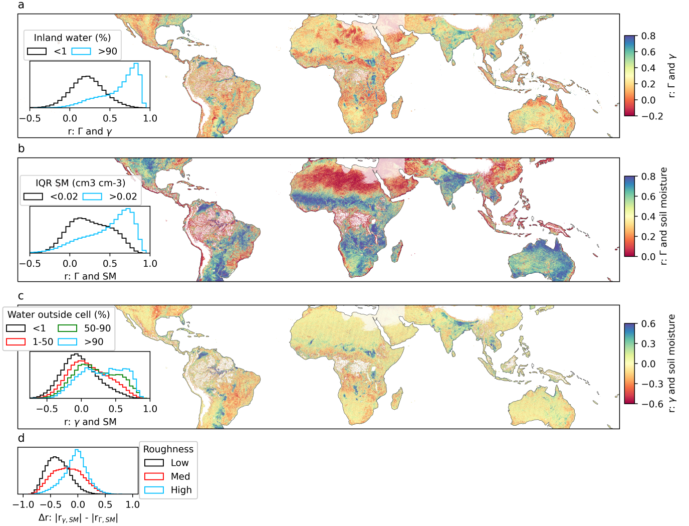
Fig. 6. (a) The correlation between daily matchups of \Gamma and \gamma during 2020 - 2024. Inset figure shows distributions of the correlation when there is <1 percent surface water fraction in the grid cell (black) and >90 percent surface water fraction (blue). (b) The correlation between \Gamma and soil moisture for the same time period. Inset figure shows distributions of the correlation when the observed IQR of soil moisture is \leq 0.02 cm 3 cm -3 (black) and >0.02 cm 3 cm -3 (blue). (c) The correlation between \gamma and soil moisture for the same time period. Inset figure shows distributions of the correlation as surface water fraction in cells surrounding the reflection point increase from <1 percent (black), to 1-50 percent (red), 50-90 percent (green), and >90 percent (blue). (d) Histograms of the difference in the absolute value of the correlation between \gamma and soil moisture and \Gamma and soil moisture. In all figures, regions with surface elevation exceeding 3000 m have been masked out, and regions in the Middle East that commonly experience RFI are semi-transparent.
