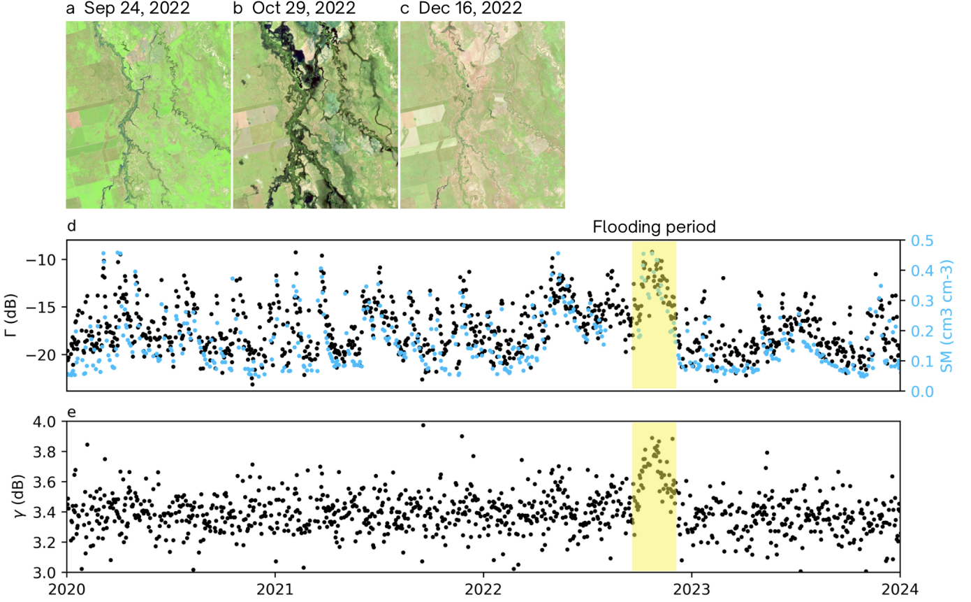
Fig. 8. Shortwave infrared (SWIR) Copernicus Sentinel images [2022] processed by the Copernicus Browser for a region in New South Wales, Australia, before (a), during (b), and after (c) a significant flood event in 2022. (d) Time series of \Gamma (black) and soil moisture (blue) for this location. (e) Time series of \gamma for the same location. The yellow semi-transparent box indicates the flooding period.
