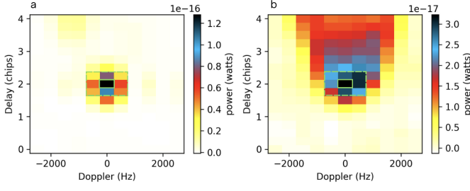
Fig. 1. Two examples of DDMs and how \Gamma and \gamma are calculated. \Gamma is the value of the peak pixel (green solid box), after antenna gain and geometric range corrections. \gamma is the difference between \Gamma and the mean value of all eight pixels surrounding the peak (dashed green box) when pixel values are in dB. The DDM in (a) was recorded over inland surface water and (b) was recorded over the open ocean. Note the difference in magnitude between the two colorbars.
