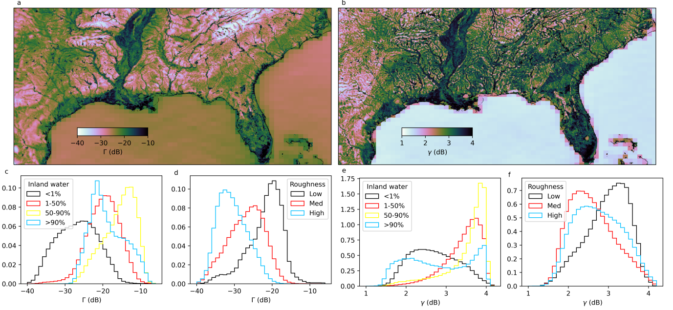
Fig. 4. (a,b) Same as Figure 3(a,c), but constrained to the eastern half of the United States. (c) Distributions of \Gamma for the entirety of CYGNSS' coverage when binned by surface water fraction. (d) Distributions of \Gamma when binned by topographic roughness. Low values of roughness are defined when 10\log\sigma \leq 5 , medium values when 5 < 10\log\sigma \leq 15 , and high values when 10\log\sigma > 15 . (e,f) Same as (c,d), but for \gamma .
