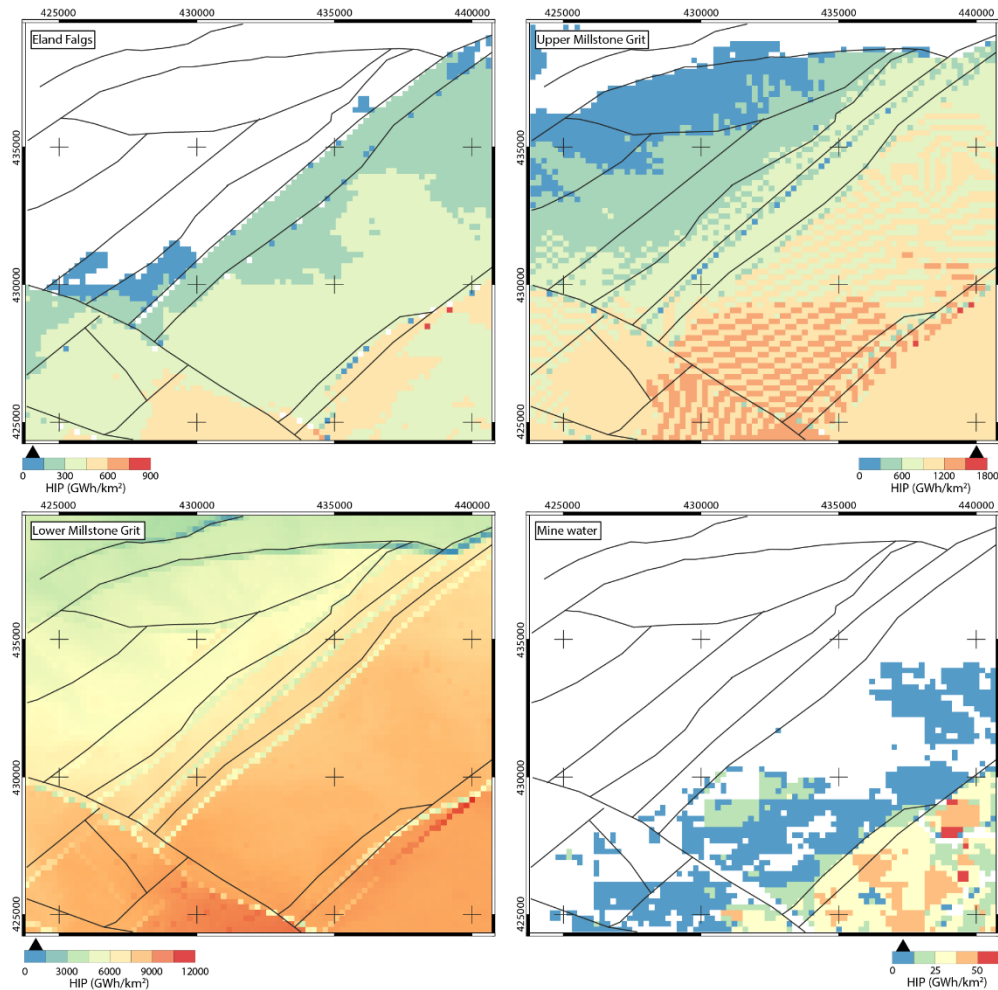
Figure 12 - Heat-in-place (HIP, GWh/km 2 ) distribution for the Eland Falgs, Upper Millstone Grit, Lower Millstone Grit, and mine water, based on the P50 stochastic model.
