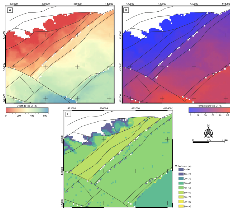
Figure 9 - Characteristics of the Elland Flags geothermal reservoir. A: Depth to top EF. B: Temperature at the top of the EF. C: Thickness of the EF.
