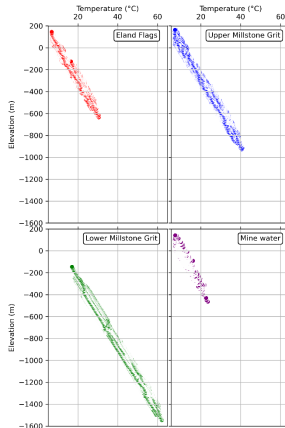
Figure 8 - Temperature distribution within the modelled geothermal reservoirs. Elevation is calculated with respect to the mean sea-level and temperatures is derived from the modelled temperature-depth equation shown in Figure 7.
