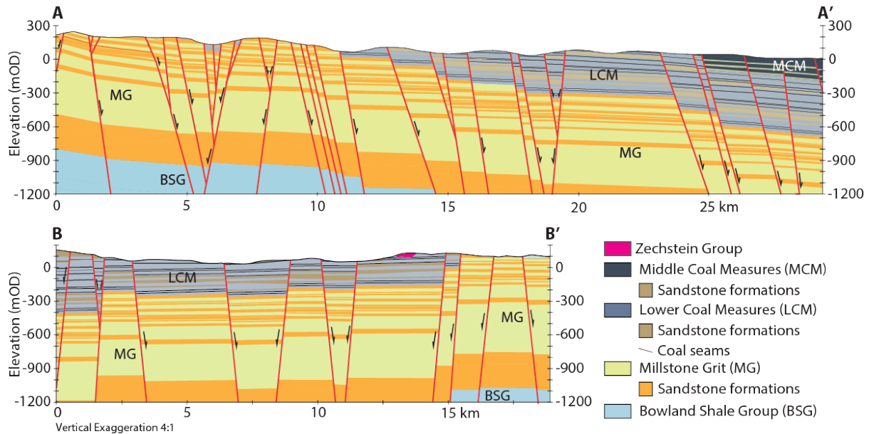
Figure 3 - Geological cross-sections across the Leeds area, illustrating the stratigraphic and structural architecture in Leeds' subsurface. The cross-sections AA' and BB' are oriented NW-SE and SW-NE, respectively. They were constructed using the BGS geological maps (1:50,000; BGS, 1998, 2000, 2003a, 2003b) and legacy well data. See Figure 2 for location of the cross-sections and well data.
