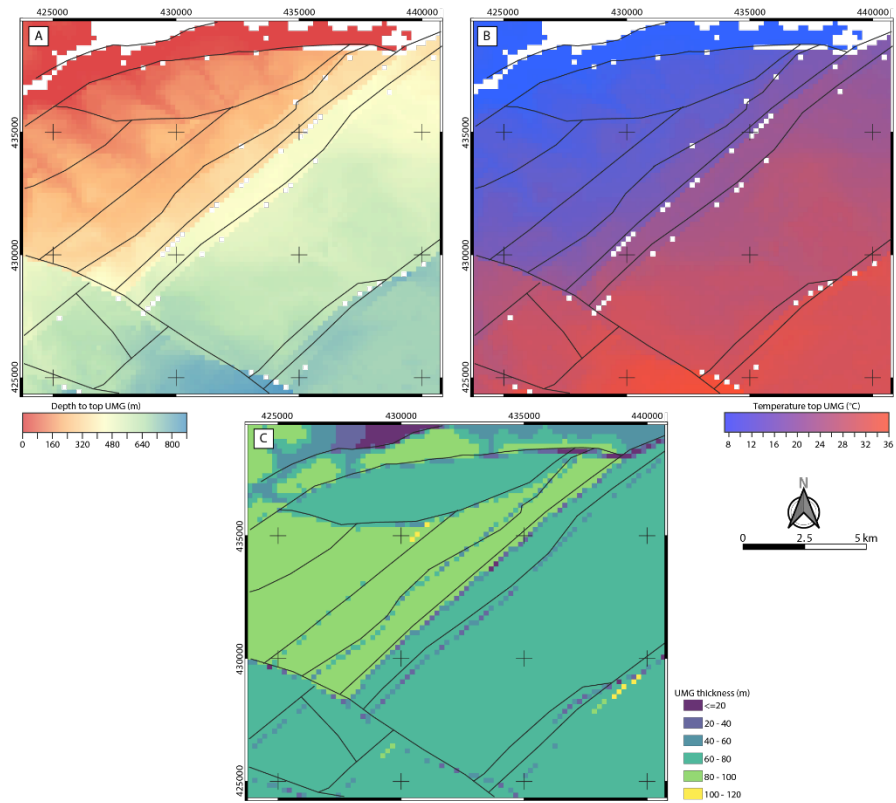
Figure 10 - Characteristics of the Upper Millstone Grit (UMG) geothermal reservoir. A: Depth to top UMG. B: Temperature at the top of the UMG. C: Thickness of the UMG.
