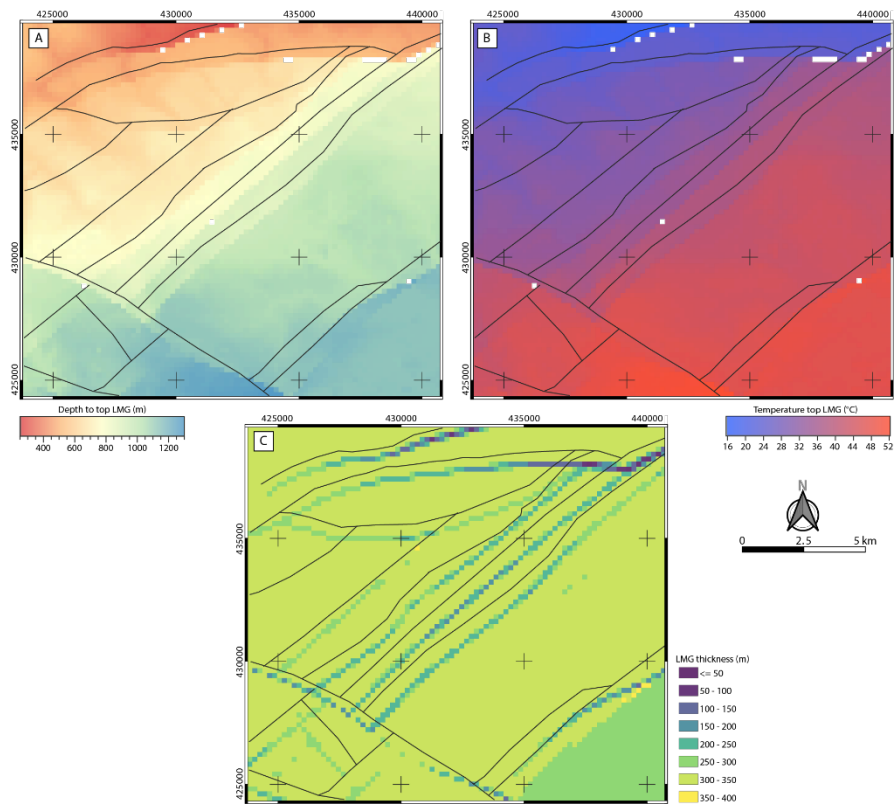
Figure 11 - Characteristics of the Lower Millstone Grit (LMG) geothermal reservoir. A: Depth to top LMG. B: Temperature at the top of the LMG. C: Thickness of the LMG.
