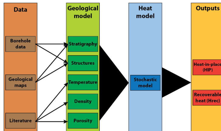
Figure 4 - Subsurface characterization and geothermal resource modelling workflow.
