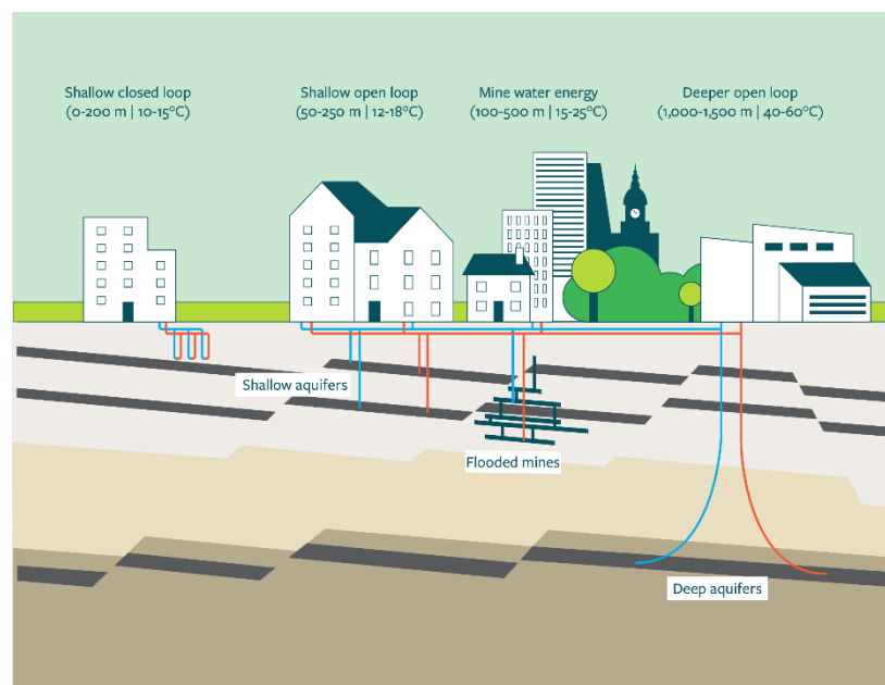
Figure 1 - Shallow subsurface geothermal solutions.
