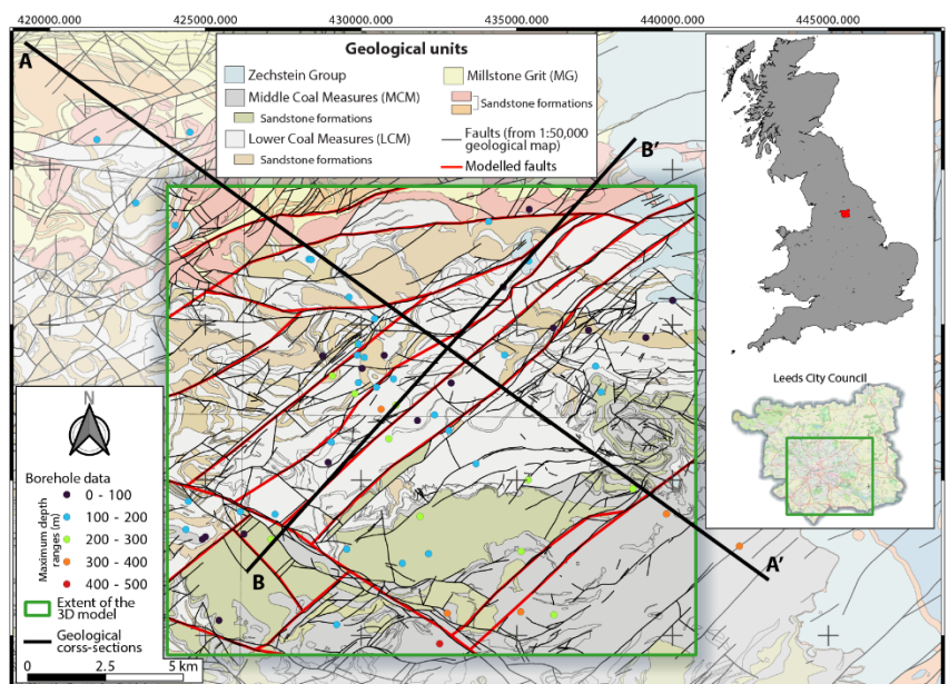
Figure 2 - Map of the study area showing the bedrock geology (BGS, 1998, 2000, 2003a, 2003b), the location of the boreholes used to build the geological model, and the location of the two geological cross-section across the Leeds' area shown in Figure 3.
