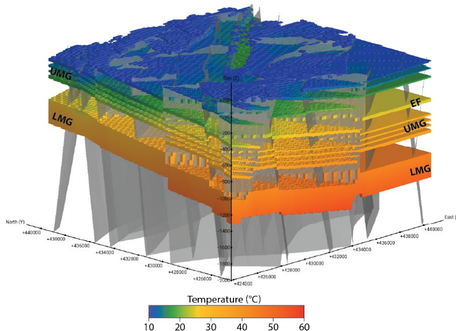
Figure 6 - View (looking toward the NE) of the 3D geological model, showing the temperature within modelled sandstone aquifers and the faults in grey. EF: Elland Flags; UMG: Upper Millstone Grit; LMG: Lower Millstone Grit.
