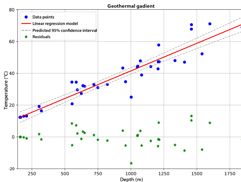
Figure 7 - Borehole temperature data and the calculated geothermal gradient derived by linear regression.
