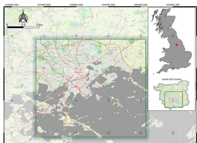
Figure 5 - Map of the Leeds area showing the spatial distribution of underground workings.
