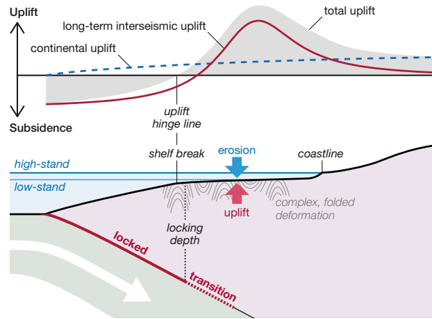
Figure 2: An erosive continental shelf requires wave-base erosion and rock uplift. These conditions are met landward of the uplift hinge line set by the combined patterns of interseismic and continental uplift (top). The shelf break is anchored at the hinge line, and the shelf can grow landward by coastal retreat (bottom). The interseismic deformation is controlled by the pattern of locked, transitional, and creeping segments of the megathrust.
