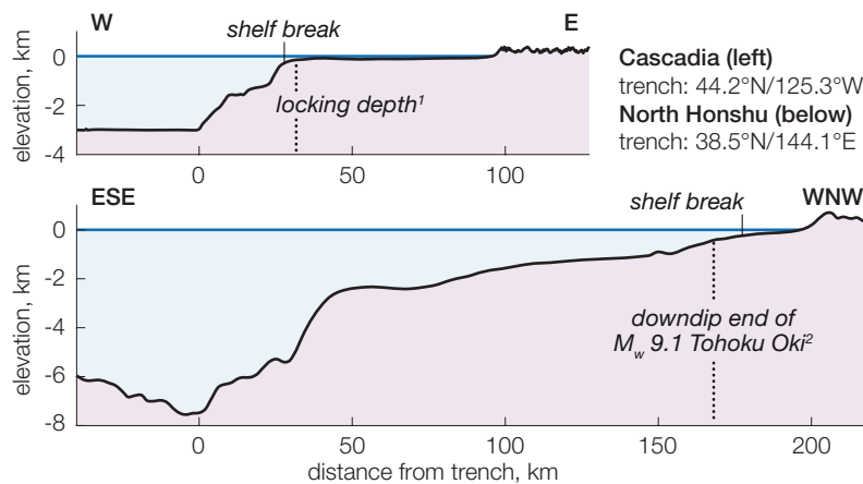
Figure 5: Profiles across the Cascadia and North Honshu margins. In Cascadia, the shelf break is a sharp and salient feature while in North Honshu the shelf break is lost in the upper continental slope. Both figures share the same scale. 1: Burgette et al. (2009); 2: Lay et al. (2011)
