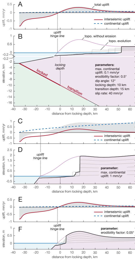
Figure 3: The numerical model is forced by an uplift field (A) derived from an interseismic back-slip calculation (adapted from Savage, 1983; Okada, 1992) of a locked fault (B) and by ocean energy causing wave-base erosion (Anderson et al., 1999). A-B shows a reference case with a wide shelf. The vertical scale is exaggerated from -200 to 1000 m in B. The model C-D has the same parameters but a ten times greater continental uplift, and model E-F has a ten times smaller rock erodibility factor. Note that these two models both have narrower shelves, and that in model C-D, the total uplift hinge-line is displaced seaward by the fast continental uplift.
