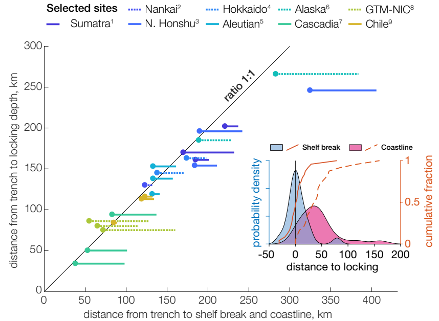
Figure 4: Position of the locking depth with respect to the shelf break and the coastline relative to the trench in selected sites (inspired by Ruff and Tichelaar (1996)). The inset distribution shows that shelf breaks are tightly distributed around the locking depth at a mean distance of 4.7 km (10 th /90 th percentiles at -18/22 km) while coastlines are removed and spread landward from it at a mean distance of 43.1 km (10 th /90 th percentiles at 3.2/76.6 km). Sources are 1: Briggs et al. (2006); Natawidjaja et al. (2007); 2: Park et al. (2002); 3: Hashimoto et al. (2009); Lay et al. (2011); 4: Hashimoto et al. (2009); 5: Johnson et al. (1994); 6: Johnson (1998); Sykes et al. (1981); 7: Burgette et al. (2009); Schmalzle et al. (2014); 8: Ye et al. (2013); 9: Lay et al. (2014); Yue et al. (2014); Li et al. (2016).
