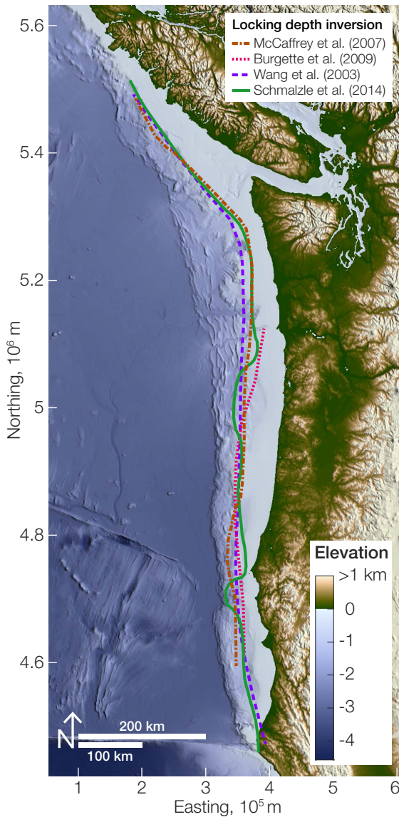
Figure 1: Solutions for the down-dip end of seismic coupling in Cascadia, derived from GPS (Wang et al., 2003; McCaffrey et al., 2007; Schmalzle et al., 2014) and road leveling (Burgette et al., 2009), follow the edge of the continental shelf and are removed from the coastline. The locking depth is outlined for a value of \sim 80\% locking. Color map from Cramer (2018).
