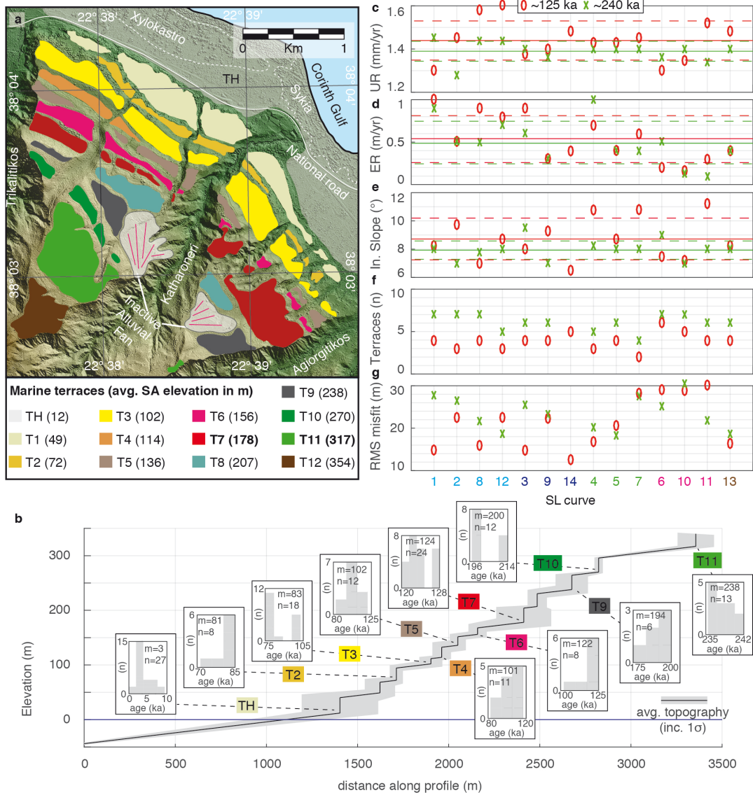
Figure 4. Modeling the marine terrace sequence at Xylokastro. (a) Map of Xylokastro marine terrace sequence. SA = shoreline angle. (b) Profile of the terrace sequence. The black line shows average-derived terrace topography (see methods) with 1\sigma uncertainty (grey envelope) and range of possible terrace ages indicated by the different SL curves, including median age (m) and number of curves (n) reproducing a given marine terrace. (c-g) Different parameters and outcomes resulting from finding the lowest RMS-misfit over the two time-scales, shown for all 14 RSL curves. Models over 125 ka and 240 ka are shown in red and green, respectively. Numbers below plot correspond to SL curve numbering and colors of Fig. 1, and are sorted by type of SL curve for easy comparison. Solid and dashed lines indicate average values and 1\sigma uncertainty. (c) Uplift rates required by the different SL curves to match the correct elevations of the dated T7 (red) and T11 (green) terraces. (d) Erosion rate for lowest RMS-misfit result. (e) Initial slope for lowest RMS-misfit result. (f) Total number of terraces for lowest RMS-misfit result. (g) Lowest RMS-misfits.
