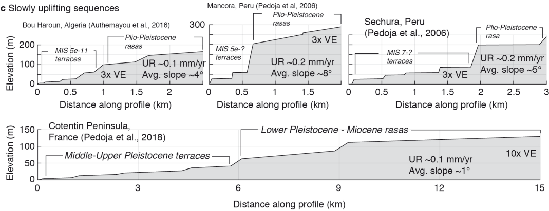
Figure 2. Marine terrace/rasa sequences. (a) Worldwide occurrence of marine terrace sequences (red), with white dots showing locations where rasas of Early to Mid-Pleistocene age or older have been described in the literature. (b) Examples of rapidly uplifting marine terrace sequences, as shown in the literature. (c) Examples of slower uplifting and older marine terrace/rasa sequences. UR = uplift rate
