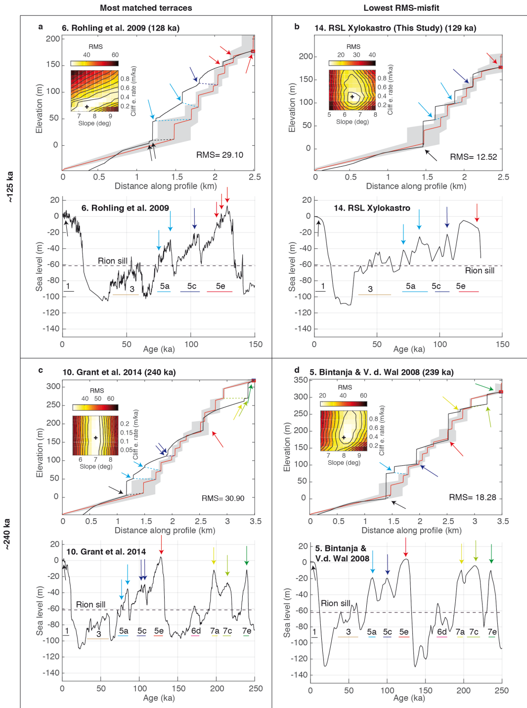
Figure 3. Examples of modeling the Xylokaastro terrace sequence. (a) for the most matched terraces over ~125 ka; (b) for the lowest RMS-misfit over ~125 ka; (c) for the most matched terraces over ~240 ka, and; (d) for the lowest RMS-misfit over ~240 ka. In profile plots (above), red lines show average-derived terrace topography (see methods) with 1\sigma uncertainty (grey envelope), black lines the modeled topography, and arrows indicate which SL highstand corresponds to which shoreline angle. Dashed lines connecting shoreline angle of modeled and observed shoreline angles indicate the correlation used for Fig. 4b. In the SL plots (below), numbers indicate MIS and letters are substages as defined by Railsback et al. (2015).
