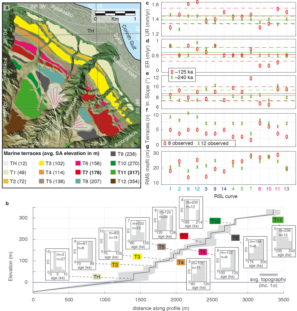
Figure 2. Modeling the marine terrace sequence at Xylokastro. (a) Map of the terraces. SA = shoreline angle. (b) The black line shows the average-derived terrace topography (see methods) with 1\sigma uncertainty (grey envelope) and range of possible terrace ages indicated by the different SL curves, including median age (m) and amount of curves (n) reproducing a given marine terrace (c-g) Different parameters and outcomes resulting from finding the lowest RMS-misfit over the two time-scales. Models over 125 ka are shown in red, and those over 240 ka in green, numbers below plot correspond to SL-curve numbering and colors of Fig. 1. Solid and dashed lines indicate average values and 1\sigma uncertainty. (c) Uplift rates required by the different SL curves to match the correct elevations of the dated T7 (red) and T11 (green) terraces. (d) Erosion rate for lowest RMS-misfit result. (e) Initial slope for lowest RMS-misfit result. (f) Total number of terraces for lowest RMS-misfit result. (g) Lowest RMS-misfit for different SL curves.
