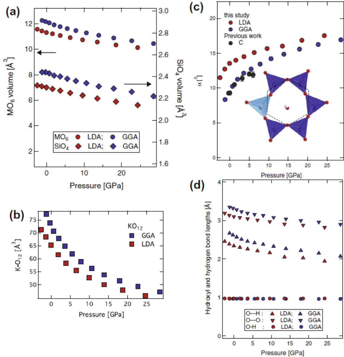
Fig. 4. Plot of volume of polyhedral units vs. pressures- (a) tetrahedral units- TO4 are represented in the right-ordinate axis; the octahedral units MO6 are represented in the left-ordinate axis; (b) the interlayer with 12-fold coordination (KO12) vs. pressure. The first principle simulations with LDA and GGA are shown in ‘red’ and ‘blue’ symbols respectively. (c) Plot of \alpha vs. pressure. The \alpha angle characterizes the in-plane rotation of tetrahedral units as shown in the inset- a perfect hexagon, shown in dashed line, the angle between consecutive oxygen atoms would be 120° and hence \alpha = 0^\circ . In contrast, for a di-trigonal ring of tetrahedral units, the angle between consecutive oxygen atoms is either greater than or less than 120° resulting in a \alpha > 0^\circ . Under compression the di-trigonal distortion characterized by \alpha , increases with pressure. The first principle simulations with LDA and GGA are shown in ‘red’ and ‘blue’ symbols respectively.
