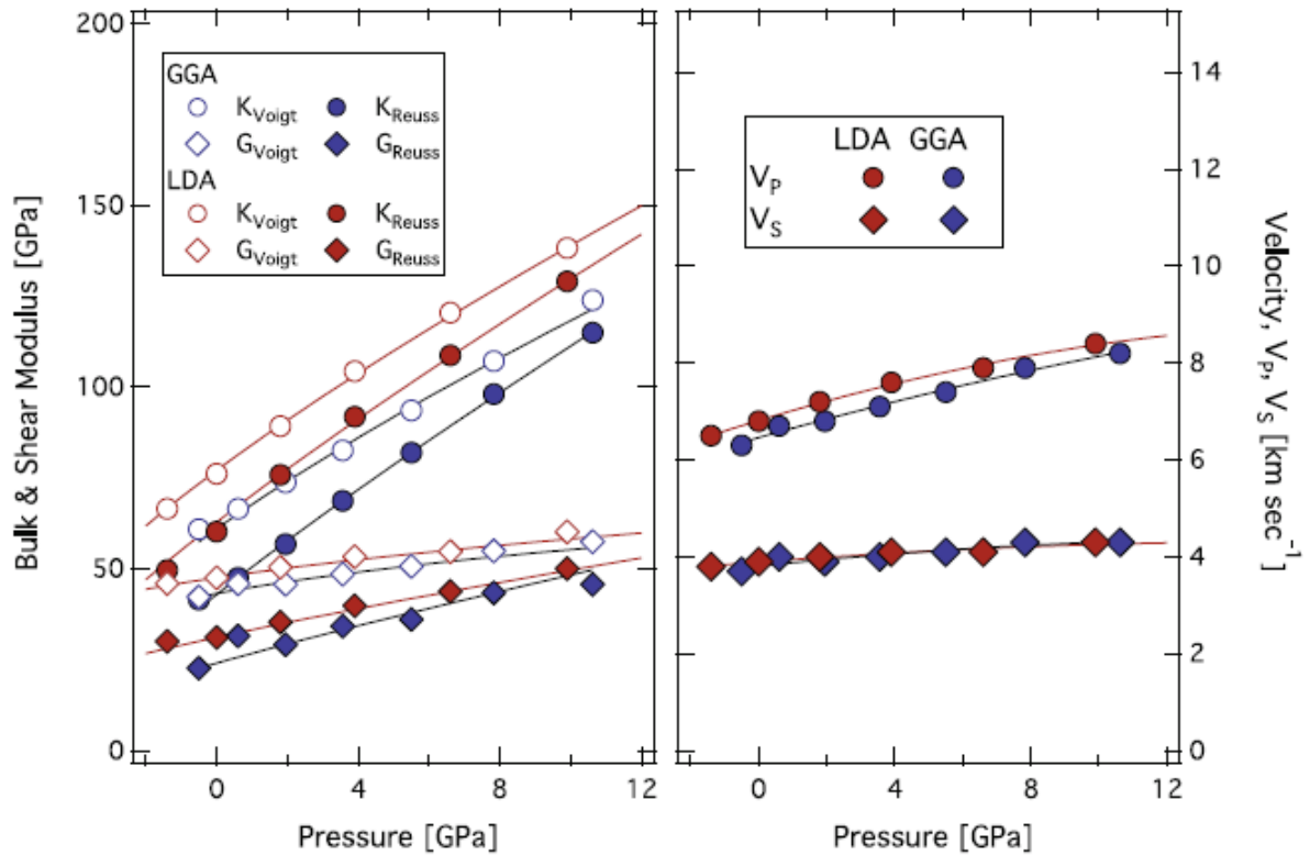
Fig. 6. (a) Plot of bulk and shear modulus vs. pressure. Both Voigt and Ruess bounds are shown. (b) Plot of compressional ( V_p ), shear ( V_s ) sound velocity vs. pressure. The ‘blue’ and ‘red’ filled symbols from first principles simulation with GGA and LDA respectively. (For interpretation of the references to color in this figure legend, the reader is referred to the web version of this article.)
