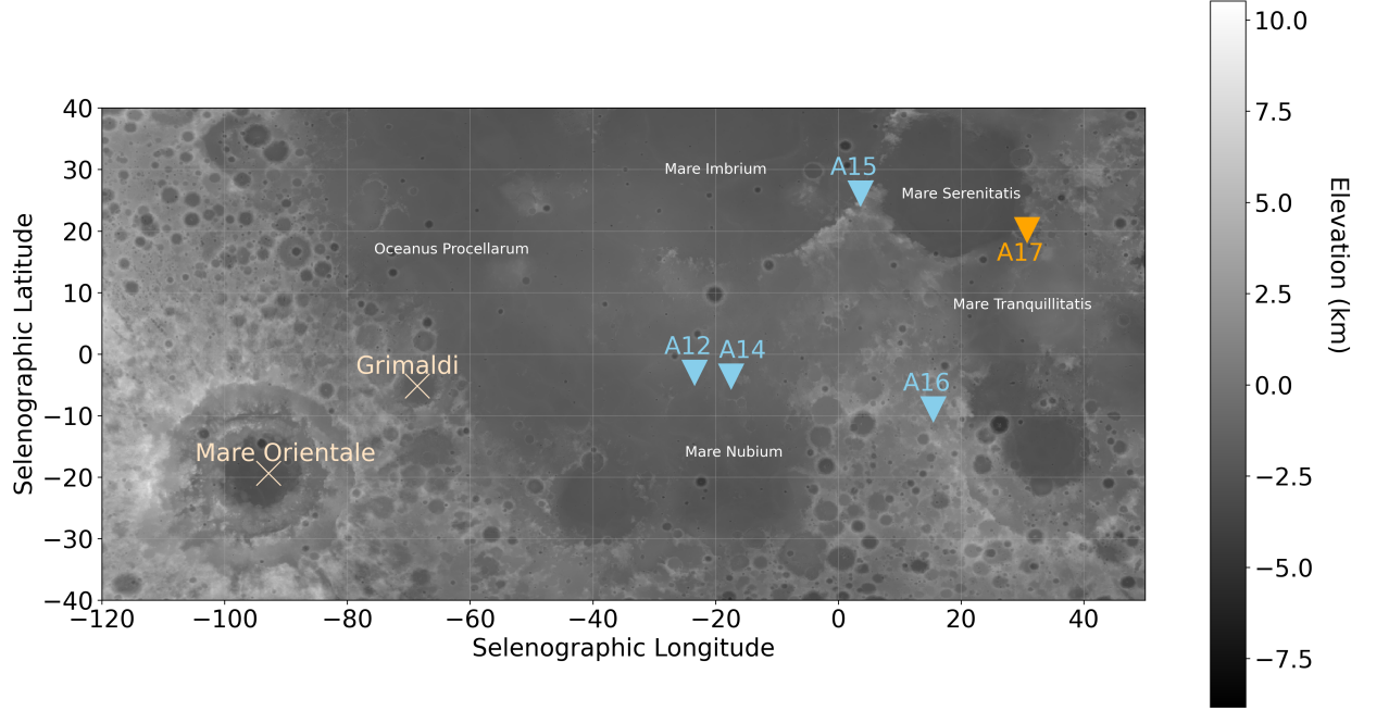
Figure 1. Identified impact flash locations from astronaut descriptions: Grimaldi Crater (Flash 2) and Mare Orientale (Flash 3). As Flash 1 occurred below the horizon, no precise location is given. Seismometers are marked with as blue triangles and the nearby major lunar mare are labelled. Apollo 11's PSE station is not shown as it had ceased recording by 1972. The eventual landing site of Apollo 17 in the Taurus-Littrow valley is also shown in orange. The background map in this image is from the Lunar Orbiter Laser Altimeter on the Lunar Reconnaissance Orbiter (Smith et al., 2010).
