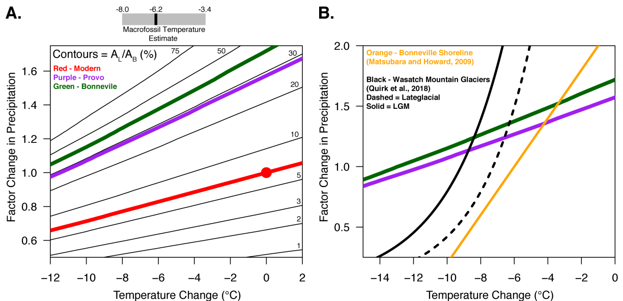
Figure 1. Hydroclimate change inferred from Lake Bonneville shoreline areas.
