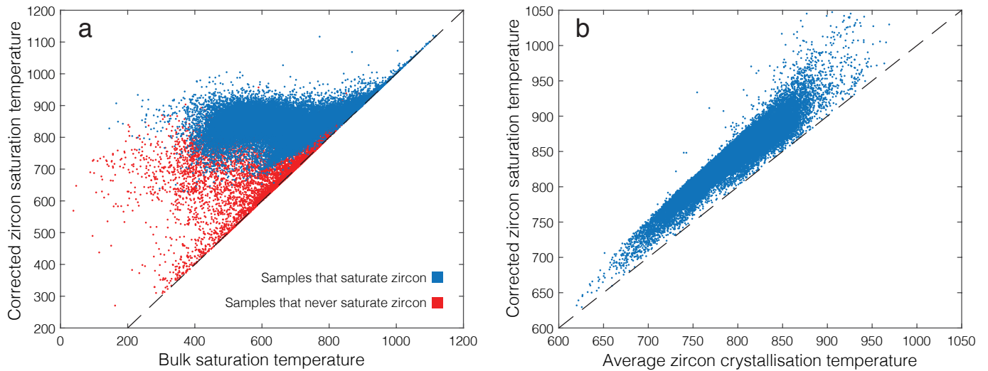
Supplementary Figure 2: The relationship between bulk zircon saturation temperatures, corrected zircon saturation temperatures, and average zircon crystallisation temperatures during closed-system equilibrium crystallisation for 52,300 whole-rock compositions. Bulk saturation temperature is the result of applying the equation of Boehnke et al. (2013) directly to each whole-rock composition. (a) Corrected zircon saturation temperature adjusts for differentiation during in-situ crystallisation, resulting in consistently higher saturation temperatures relative to bulk saturation temperature, as observed in panel. For samples that do not ever saturate zircon, the highest saturation temperature of any differentiated melt is reported. (b) For samples which do saturate zircon, average zircon crystallisation temperature is the weighted average of the zircon crystallisation temperature distribution, resulting in temperatures closely correlated with but necessarily colder than the adjusted zircon saturation temperature. While not highly sensitive to pressure or water content, the values shown here are calculated for shallow, water saturated conditions (2 kbar and 4wt % H 2 O).
