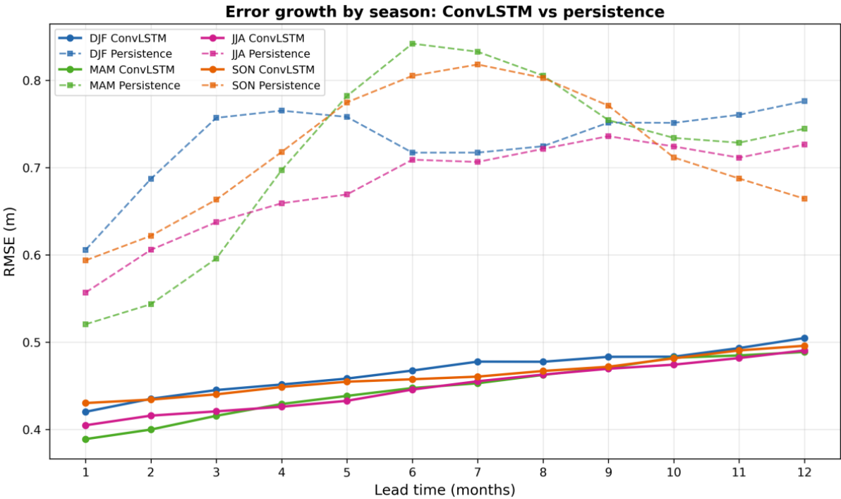
810 Figure 10. Error growth curves stratified by target season (DJF, MAM, JJA, and SON) for both ConvLSTM (solid lines with circles) and persistence (dashed lines with squares). ConvLSTM outperformed persistence at all leads and seasons, with the largest advantage in winter and spring.
