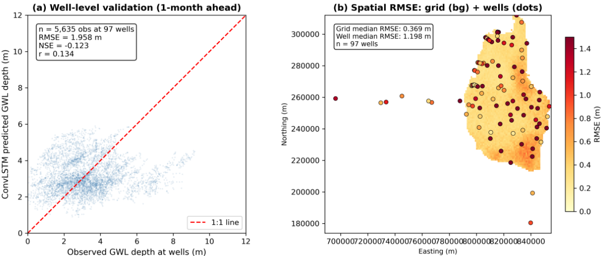
Figure 12. Point-scale well validation: (a) scatter plot of ConvLSTM 1-month-ahead predictions versus raw well observations (n = 5635 pairs at 97 wells); (b) spatial RMSE distribution at grid level (background) with per-well RMSE overlaid (dots).
