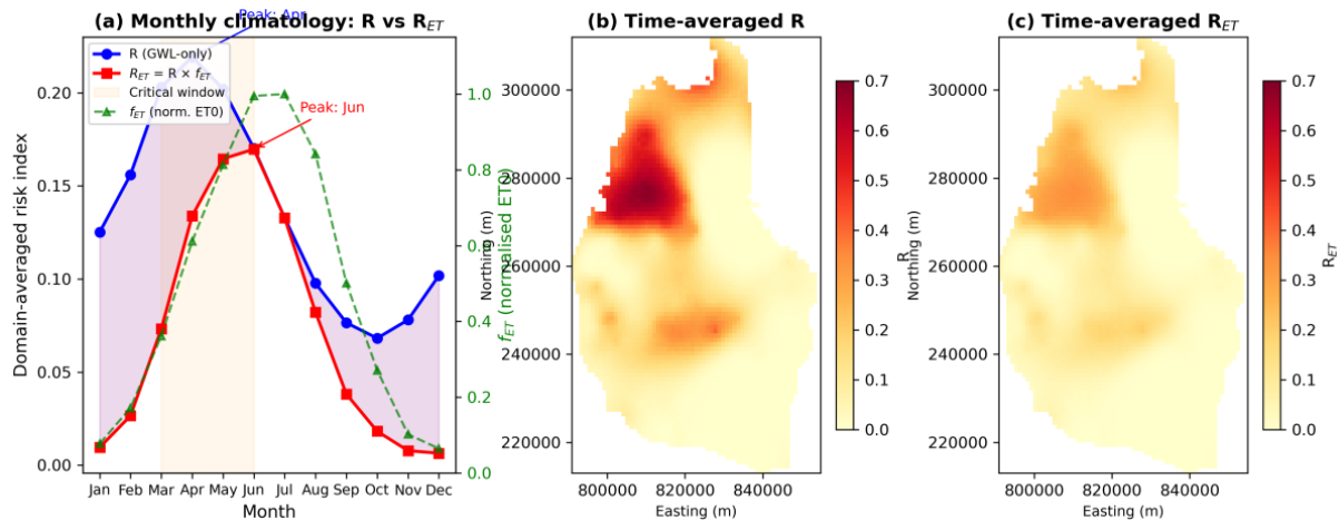
Figure 11. ET-weighted risk sensitivity analysis: (a) monthly climatology of domain-averaged R (blue circles), RET (red squares), and normalized ET0 ( f_{ET} , green triangles, right axis); (b) time-averaged R map; (c) time-averaged RET map. The orange shading in (a) indicates the March–June critical window.
