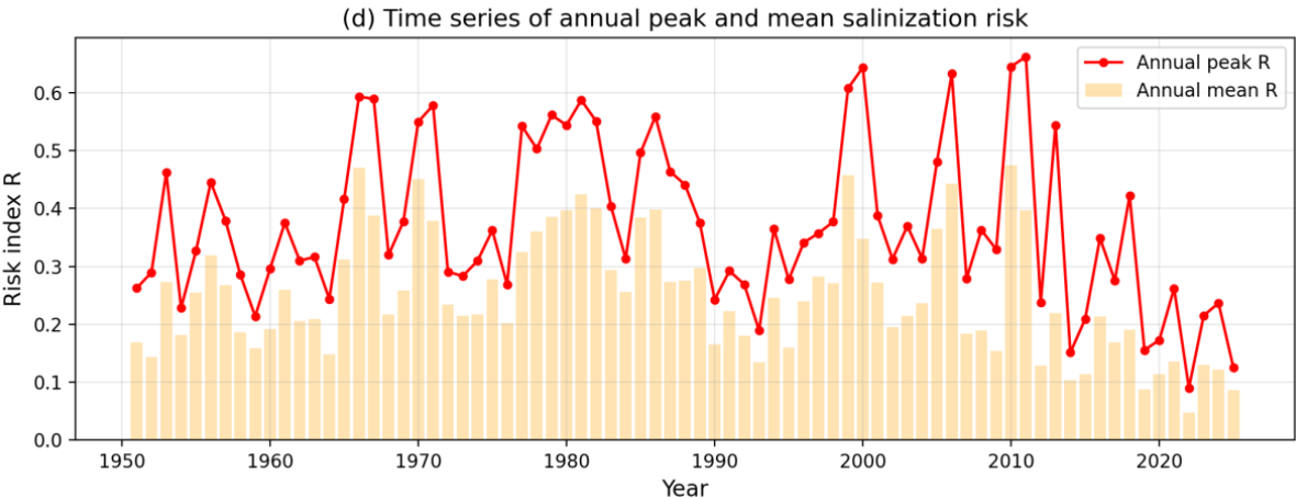
Figure 5d. Time series of domain-averaged annual peak and mean salinization risk (1951–2025). The annual peak R (red line) showed substantial interannual variability overlaid on a weak downward trend. Orange bars indicate annual mean R.
