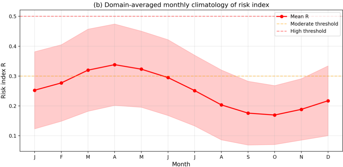
Figure 5b. Domain-averaged monthly climatology of salinization risk index R(t) . The peak in April coincided with the shallowest water table, not with the peak ET demand. Horizontal dashed lines indicate moderate (0.3) and high (0.5) risk thresholds, respectively.
