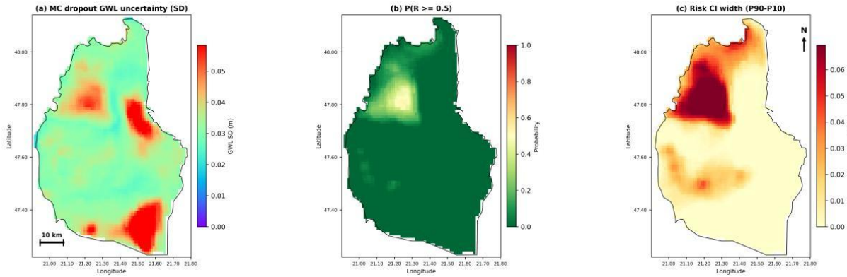
Figure 9. MC dropout uncertainty maps (50 stochastic forward passes, 60 evaluation time steps): (a) time-averaged GWL prediction standard deviation (m), (b) probability of high risk P(R \geq 0.5) , (c) risk credible interval width (P90 – P10). The narrow uncertainty bands confirm robust risk classification across the domain.
