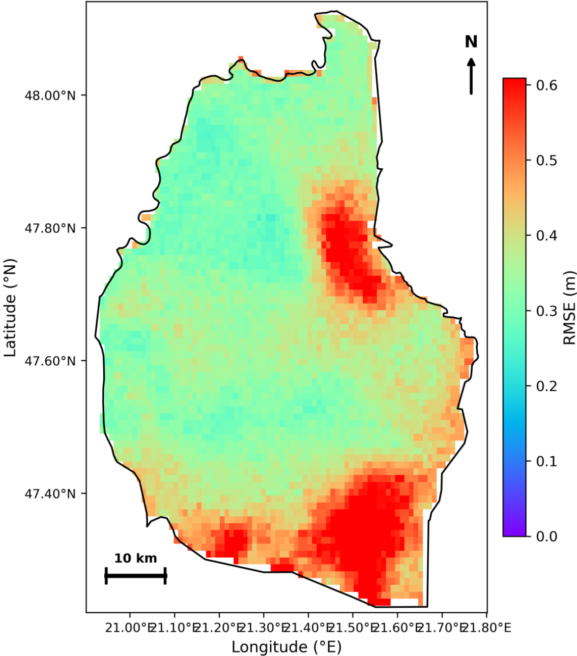
(a) Spatial RMSE - 1-month-ahead forecast
