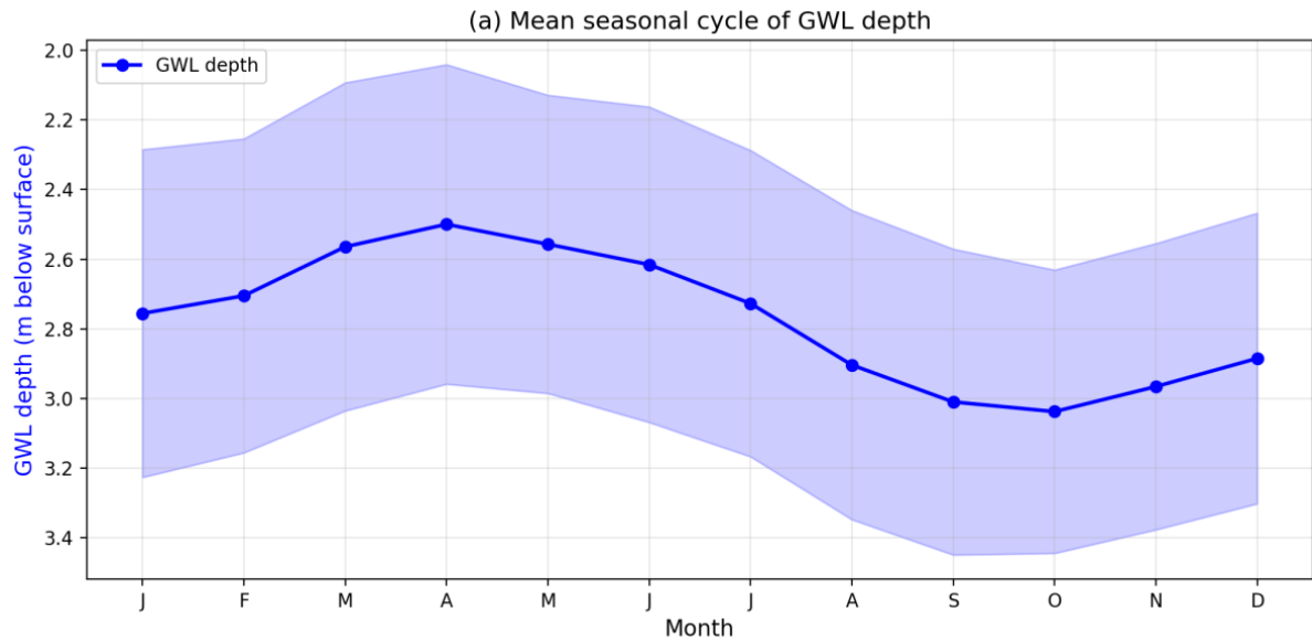
Figure 4a. Domain-averaged mean seasonal cycle of GWL depth (blue, left axis), showing the sinusoidal pattern with shallowest levels in April and deepest in October. Error bands show \pm 1 SD across grid cells.
