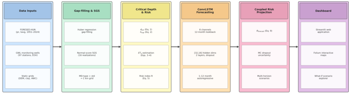
465 Figure 2. Schematic of the methodological framework showing the processing chain: data inputs (FORESEE-HUN climate, GWL monitoring network, static grids) → gap-filling and SGS interpolation → critical depth and risk index computation → ConvLSTM spatiotemporal forecasting → coupled risk projection with MC dropout uncertainty → interactive dashboard.
