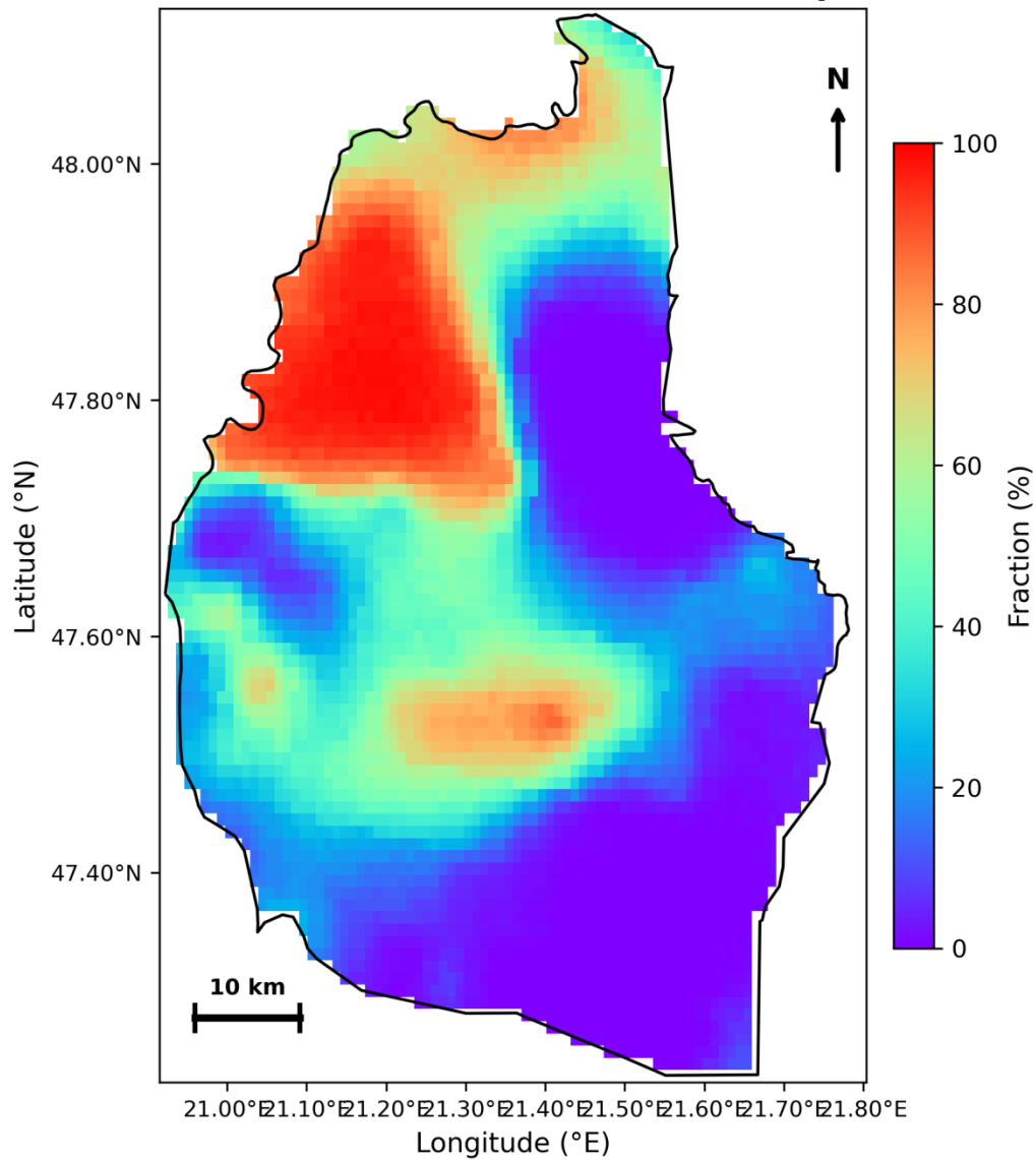
Figure 4c. Fraction of the historical record during which the water table resides above the critical depth d_{crit} ( k_d = 2.5 m). Warm colors indicate chronically elevated risk zones. [Editorial note: the title baked into this raster image reads “extinction depth”; regenerate the source plot with “critical depth d_{crit} ” to match the paper's own terminology note in Sect. 1, which explicitly reserves “extinction depth” for the static Shah et al. (2007)/MODFLOW parameter.]
