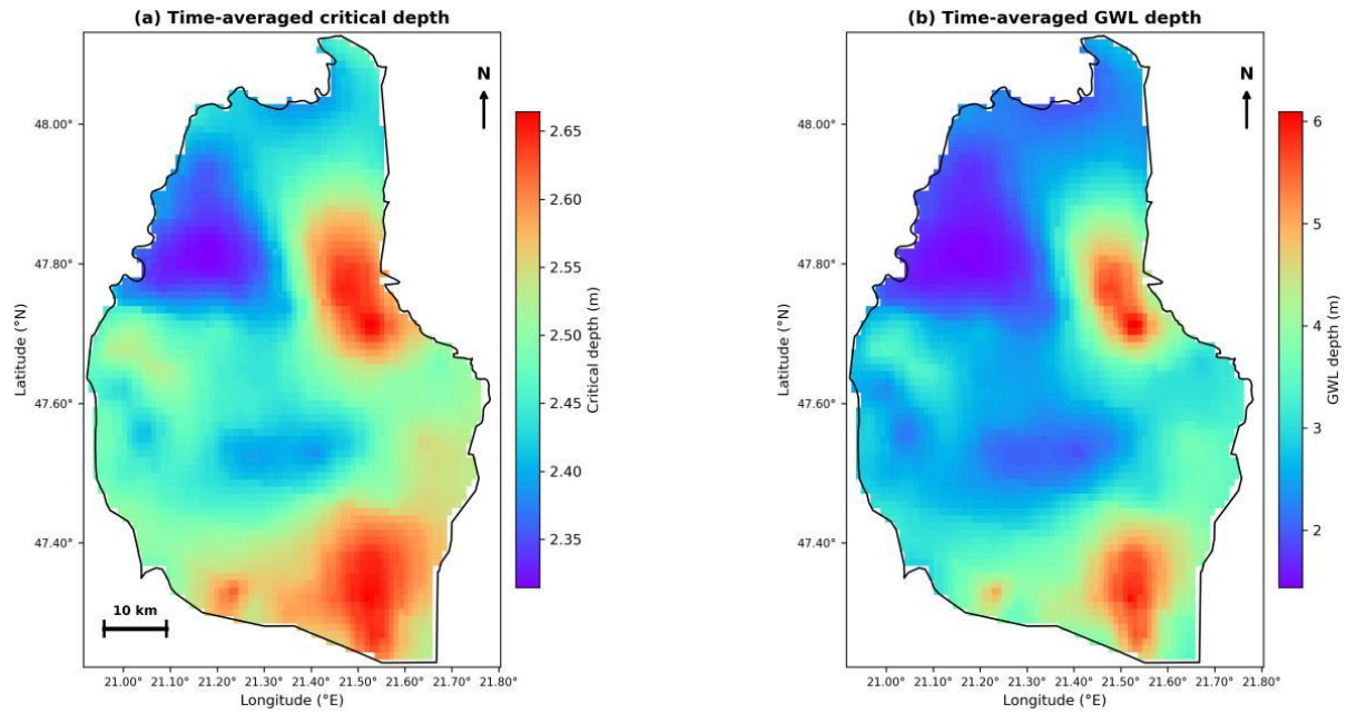
Figure 3. Spatial distribution of critical depth over the TIKEVIR domain: (a) time-averaged critical depth from the GWL-dependent empirical model with k_d = 2.5 m (Eq. 1), (b) time-averaged GWL depth (m below surface).
