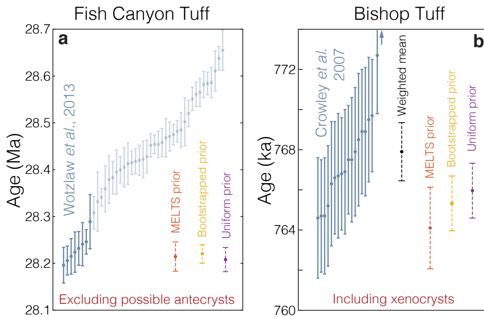
Supplementary Figure 4: Bayesian eruption age estimates for alternate Bishop Tuff and Fish Canyon Tuff datasets: a arbitrarily excluding all zircon ages older than 28.3 Ma in the Fish Canyon dataset, and b including two xenocrysts (one off-scale) in the Bishop Tuff dataset. Compared to a uniform distribution, empirical estimates and MELTS calculations provide more informative relative crystallization distributions – yielding more accurate results in an ideal system, but with increased risk of overfitting. If all zircons were strictly autocrystic, the presence of outliers would suggest that we are incompletely sampling the zircon saturation distribution, and thus overestimating the eruption age. Including xenocrystic outliers in the Bayesian age interpretation thus leads to underestimation of the eruption age and divergence between Bayesian and weighted mean ages for the Bishop Tuff. Consequently, methods for quantitatively identifying xenocrystic grains unrelated to in-situ crystallization of the erupted magma are of particular utility.
