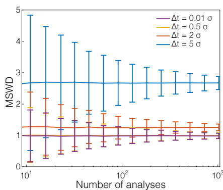
Figure 4: The uncertainty of the MSWD for analytical datasets as a function of N for a range of \Delta t/\sigma . The case of \Delta t = 5\sigma is not distinguishable from instantaneous crystallization with N less than \sim 50 , and \Delta t = 2\sigma is not distinguishable with N less than \sim 700 .
