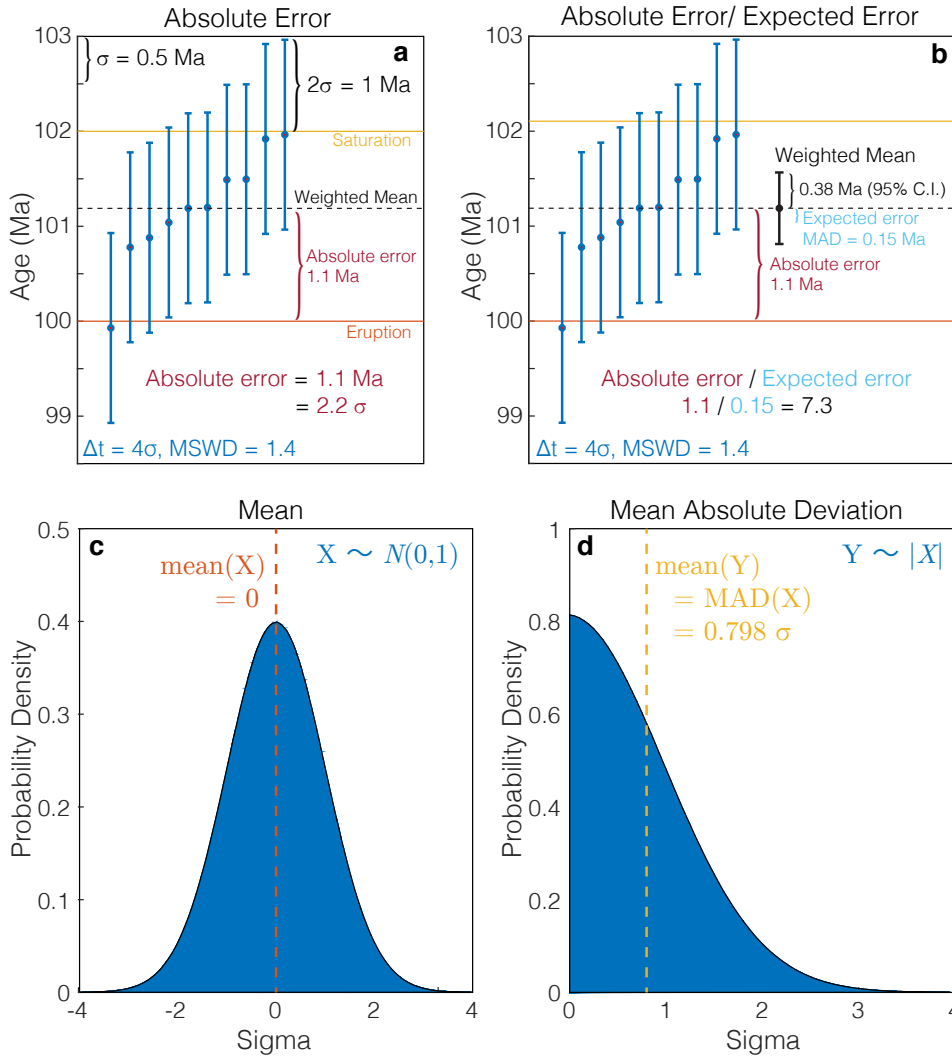
Supplementary Figure 7: Explanation of some of the terms used in Fig. 2. a Illustrates the calculation of absolute error (c.f. Fig. 2a-d) for an example dataset with \Delta t = 4\sigma and average analytical error \sigma = 0.5 \text{ Ma} . For a weighted mean age of 101.1 Ma and a true eruption age of 100.0 Ma, we find an absolute error of 1.1 Ma, equal to 2.2 \sigma . For the same example dataset, the ratio of absolute error to expected error (c.f. Fig. 2e-h) is calculated in b : absolute error is unchanged, while expected error is equal to the mean absolute deviation (MAD) of the resulting weighted mean. Mean absolute deviation is further explained in c and d . The familiar probability density function (PDF) of a standard normal random variable X with mean of 0 and variance 1 is illustrated in panel c . The distribution is symmetric about the mean. The PDF of a corresponding half-normal random variable Y = |X| is shown in d ; the mean of Y is the mean absolute deviation of X . In general, the mean absolute deviation of any Gaussian random variable is equal to 0.798 times the standard deviation.
