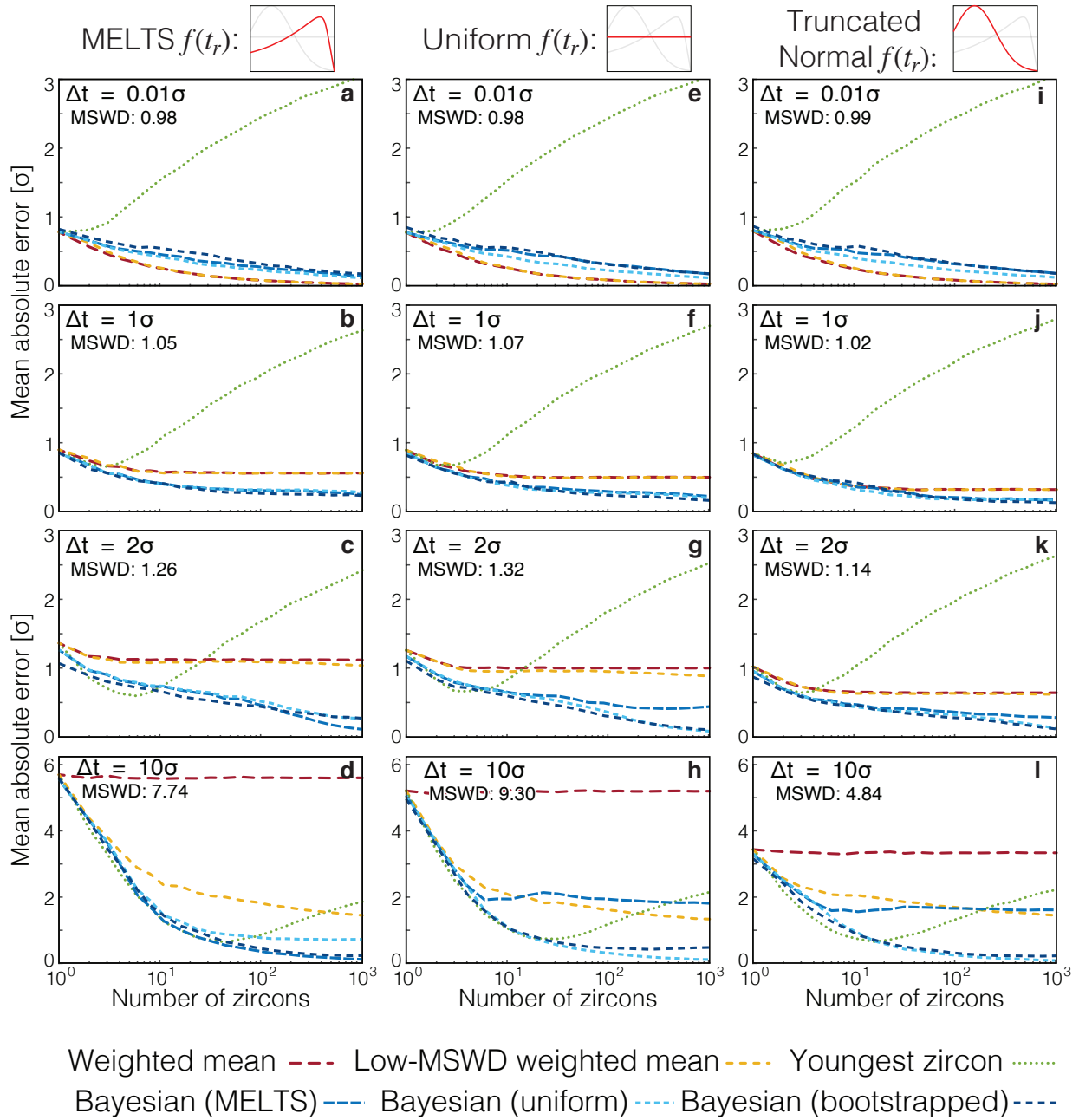
Supplementary Figure 5: A comparison of the absolute error of each age interpretation for synthetic data drawn from different relative crystallization distributions f(t_r) . a-d : MELTS crystallization distribution as in Figure 2. e-h : uniform crystallization distribution. i-l : truncated Normal crystallization distribution. Assuming a uniform crystallization distribution provides the most consistently accurate results at low \Delta t/\sigma , while the “bootstrapped” distribution interpretation (based on a truncated kernel density estimate for each synthetic dataset) consistently performs well at high \Delta t/\sigma . As in Figure 2, mean absolute error is the mean absolute deviation of the model result from the true value, reported in units of analytical uncertainty, \sigma ; lower absolute errors are better. Each datum reflects the mean of 1200 synthetic dataset tests; standard error of the mean is on the order of the line width.
