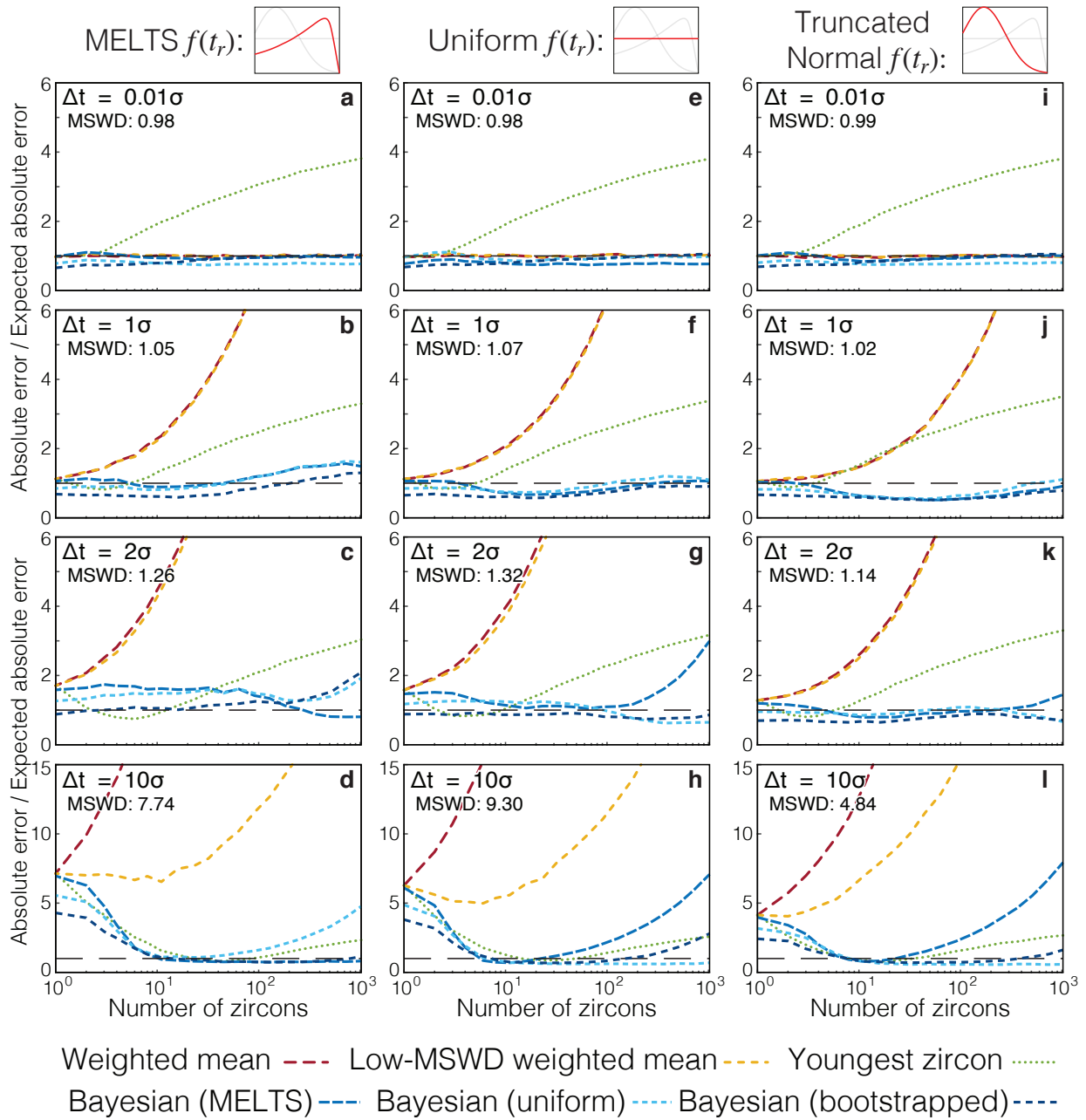
Supplementary Figure 6: A comparison of the relative error of each age interpretation for synthetic data drawn from different relative crystallization distributions f(t_r) . a-d : MELTS crystallization distribution as in Figure 2. e-h : uniform crystallization distribution. i-l : truncated Normal crystallization distribution. Assuming a uniform crystallization distribution provides the most consistently accurate results at low \Delta t/\sigma , while the “bootstrapped” distribution interpretation (based on a truncated kernel density estimate for each synthetic dataset) consistently performs well at high \Delta t/\sigma . As in Figure 2, “error / expected error” quantifies the accuracy of the model uncertainty for each age interpretation. A value greater than one indicates an underestimation of the model uncertainty ( i.e. , overprecision), while a value lower than one indicates an overestimation of the model uncertainty. Each datum reflects the mean of 1200 synthetic dataset tests; standard error of the mean is on the order of the line width.
