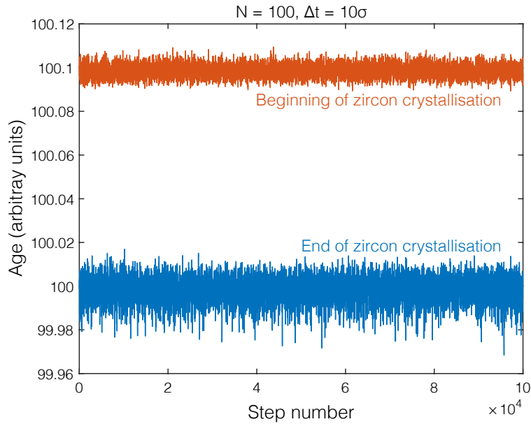
Supplementary Figure 3: Saturation and eruption ages of the first 10^5 steps of of the Markov chain for an MCMC inversion of a synthetic dataset with 100 zircons and \Delta t = 10\sigma . Due to the simple monotonic nature of the likelihood function for such an age inversion, and the availability of accurate initial guesses ( i.e. , the oldest and youngest zircon), the distribution is immediately stationary. A weighted mean age must always plot on the line of instantaneous crystallization.
