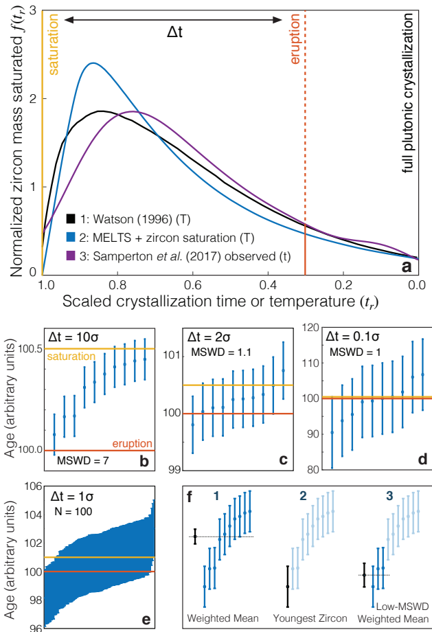
Figure 1: Zircon distributions. a : Theoretical and empirical relative zircon crystallization distributions f(t_r) , scaled from initiation to termination of zircon crystallization. 1: Kinetic model of Watson (1996) , based on zirconium diffusion constraints. 2: Thermodynamic model of Keller et al. (2017) using MELTS calculations. 3: Observed zircon crystallization distributions of Samperton et al. (2017) , shown as a kernel density estimate for all autocrystic zircons, truncated at \pm 1 kernel bandwidth. b-d : Representative synthetic zircon age datasets for a variety of \Delta t/\sigma at N = 10 . e : Example dataset with N=100 at \Delta t = 1\sigma ; note the range is greater than in c despite lower \Delta t . f : Schematic illustration of the three most common volcanic zircon age interpretations.
