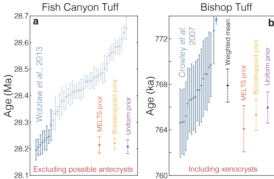
Supplementary Figure 5: Bayesian eruption age estimates for alternate Bishop Tuff and Fish Canyon Tuff datasets: a arbitrarily excluding all zircon ages older than 28.3 Ma in the Fish Canyon dataset, and b including two xenocrysts (one off-scale) in the Bishop Tuff dataset. Compared to a uniform distribution, empirical estimates and MELTS calculations provide more informative relative crystallization distributions – yielding more accurate results in an ideal system, but with increased risk of overfitting. If all zircons were strictly autocrystic, the presence of outliers would suggest that we are incompletely sampling the zircon saturation distribution, and thus overestimating the eruption age. Including xenocrystic outliers in the Bayesian age interpretation thus leads to underestimation of the eruption age and divergence between Bayesian and weighted mean ages for the Bishop Tuff. Consequently, methods for quantitatively identifying xenocrystic grains unrelated to in-situ crystallization of the erupted magma are of particular utility.
