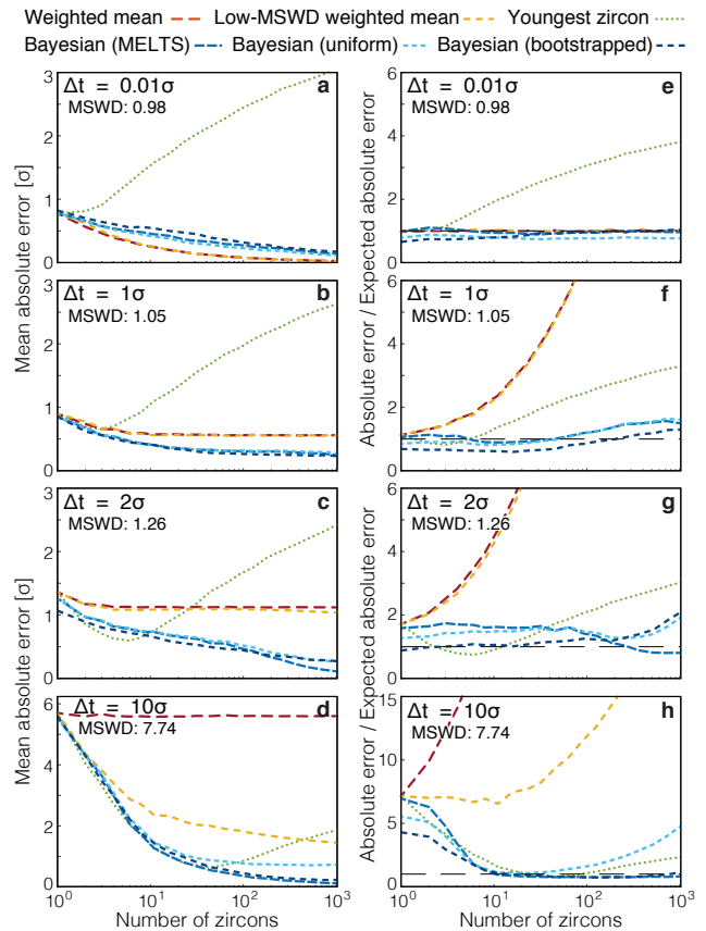
Figure 2: Performance of each age interpretation as a function of N and \Delta t/\sigma . a-d : Mean absolute error is the mean absolute deviation of the model result from the true value; lower absolute errors are better. e-h : Accuracy of the model uncertainty for each age interpretation. A value greater than 1.0 indicates an underestimation of the model uncertainty (i.e., overprecision), while a value lower than 1.0 indicates an overestimation of the model uncertainty. MSWD in each panel is the average mean square of weighted deviation (also known as the reduced chi-squared statistic) for that \Delta t/\sigma over all N . Each datum reflects the mean of 1200 synthetic dataset tests; standard error of the mean is on the order of the line width.
