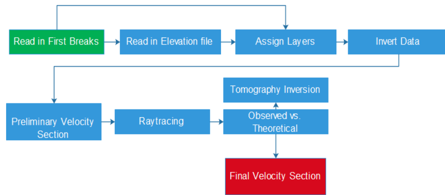
Figure 7: General flow chart of a Time-Term technique
