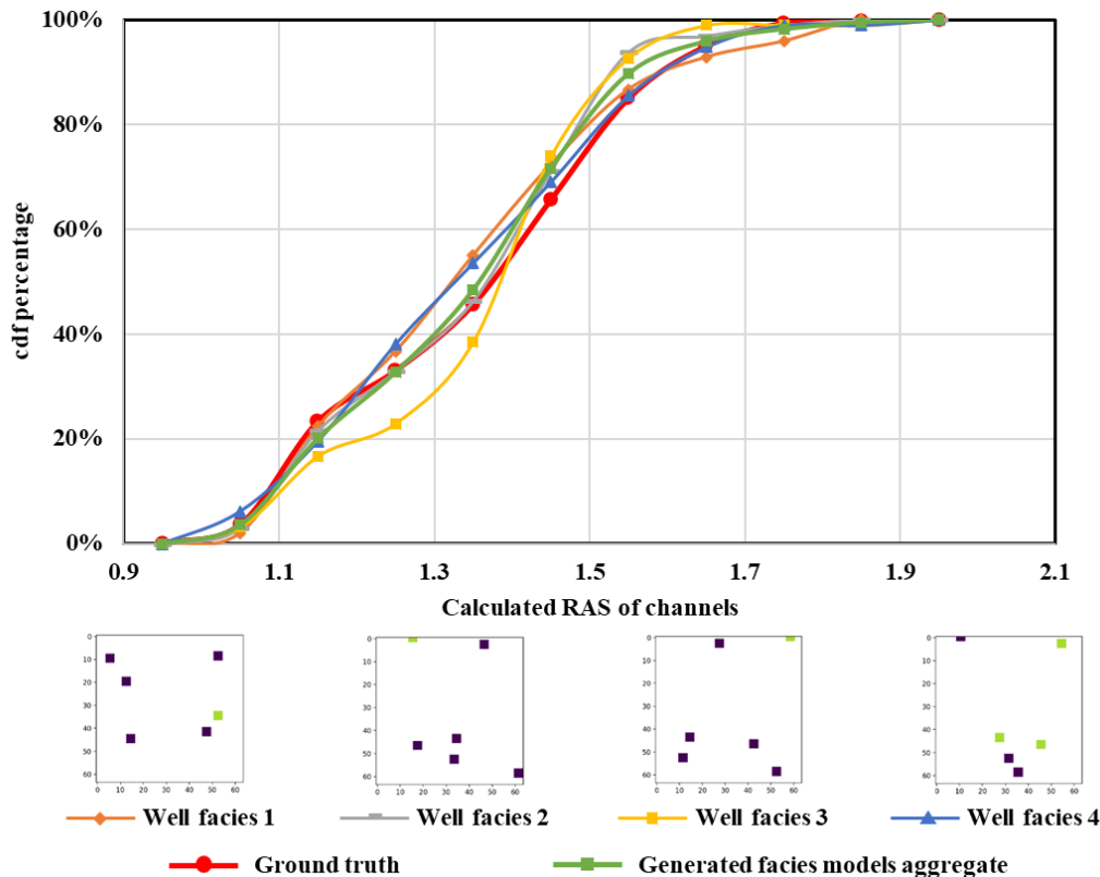
Fig. 22. Channel sinuosity distributions (cdf) of test facies models, generated facies models with
