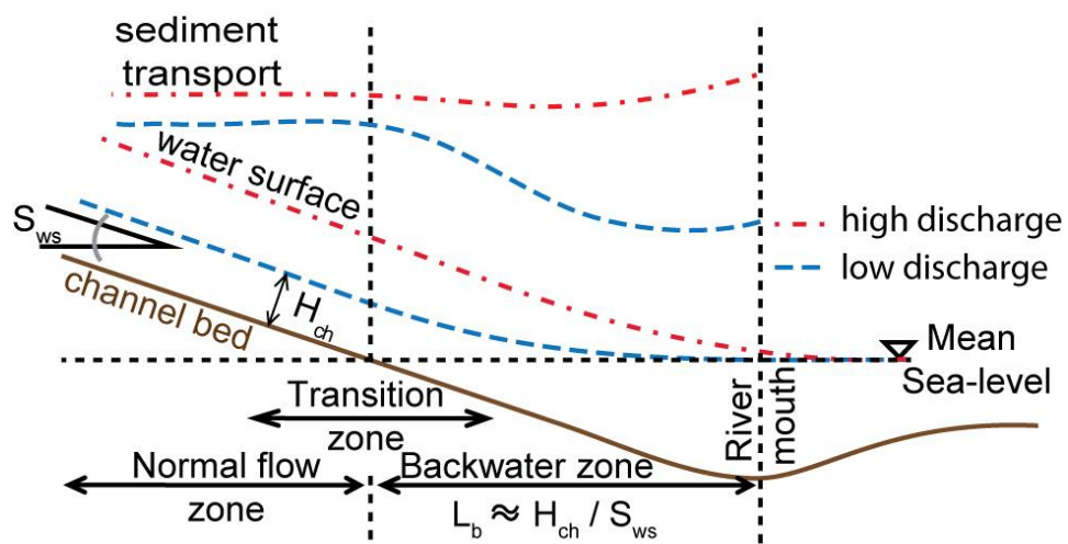
Figure 1: Schematic summarizing spatial and temporal patterns in water surface slope and predicted sediment transport trends (modified from Nittrouer et al., 2012)
