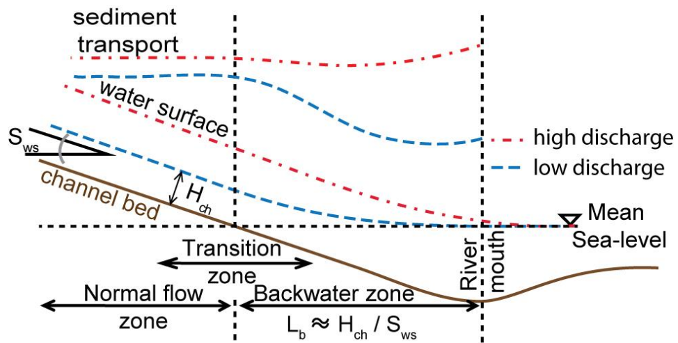
Figure 1: Schematic summarizing spatial and temporal patterns in water surface slope and predicted sediment transport trends (from Nittrouer et al., 2012)
