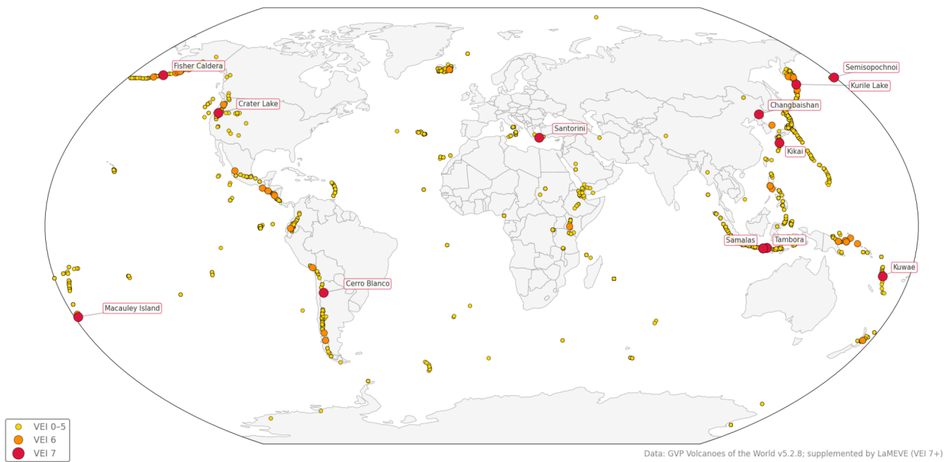
Figure 4: Global distribution of known volcanic eruptions in the Holocene (last 11,700 years) for VEI 0-7. Note due to incomplete volcanic records, especially further back in time, this map does not capture all volcanic eruptions in the Holocene. Colored by Volcanic Explosivity Index (VEI). Based on Global Volcanism Program and Venzke (2025) and Croweller et al. (2012). VEI 7 Holocene eruptions are labelled.
