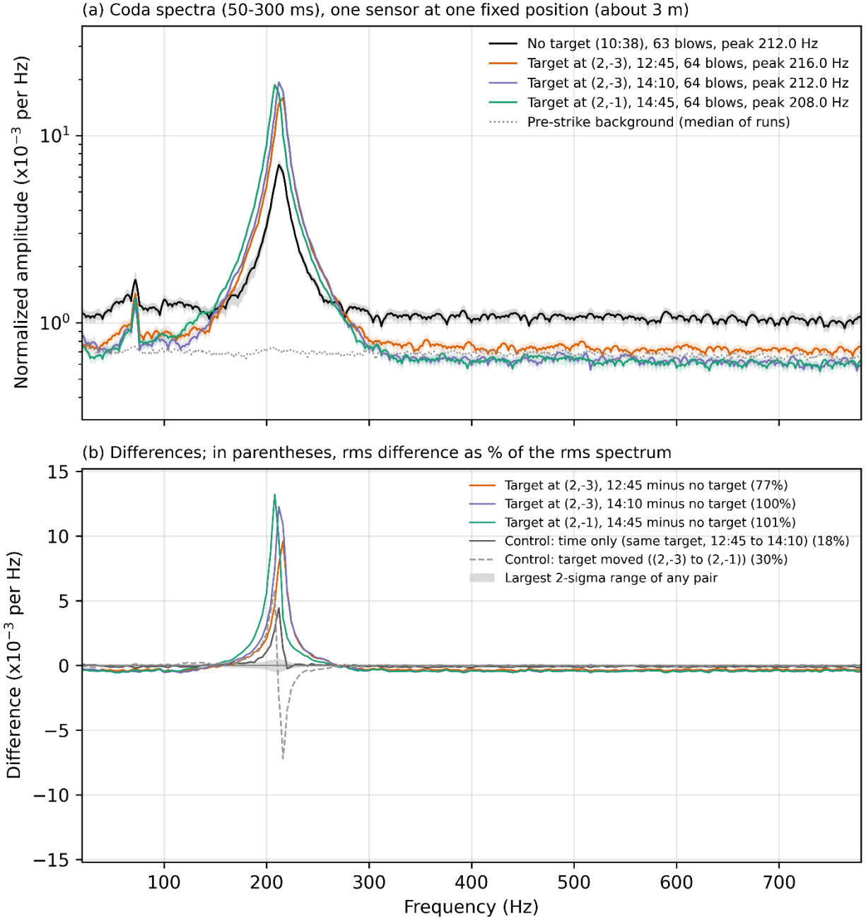
Figure 4. BCDC IPG CLAY coda spectra from one sensor at about 3 m from the source: one run without and three runs with ERW simulants.
