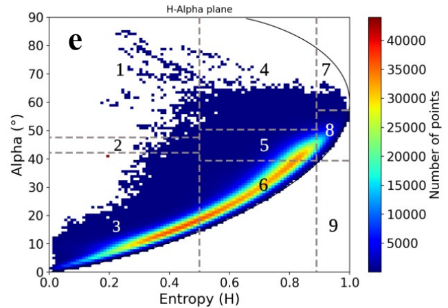
Fig. 7. The H/A/\bar{\alpha} decomposition and Cloude-Pottier classification ( H - \alpha plane) Overall, the classification results are well matched with the Pauli and Span images above. A note on interpretation: entropy describes the degree of randomness in the scattering process, ranging from 0 (a single dominant scatterer) to 1 (multiple, random scattering mechanisms). In the H - \alpha plane, zone 1 corresponds to a quasi-deterministic dihedral reflector ( \alpha > 50^\circ , H < 0.5 ), representing double-bounce scattering (e.g., from trunk-ground and ground-building interactions). Zone 2 identifies quasi-deterministic dipole scattering ( 40^\circ < \alpha \leq 50^\circ , H < 0.5 ), typically associated with volume diffusion in oriented vegetation structures. Zone 3 represents quasi-deterministic Bragg surface ( \alpha \leq 40^\circ , H < 0.5 ), characteristic of calm water or smooth soil. Zone 4 denotes medium entropy double-bounce scattering ( \alpha > 50^\circ , 0.5 \leq H \leq 0.9 ). Zone 5 ( 40^\circ \leq \alpha \leq 50^\circ , 0.5 \leq H \leq 0.9 ) indicates medium entropy (moderately random) anisotropic scattering (vegetation canopy), while zone 6 identifies random surface scattering. The high entropy zones ( H \geq 0.9 , highly random) comprise zone 7 (complex multiple scattering), zone 8 (random anisotropic scattering), and zone 9 (non-feasible quadrant) where low alpha angles are mathematically incompatible with high randomness [24], [34].
