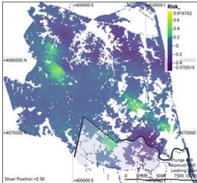
Figure 7. E-type map of the Composite Contamination Index (CCI), derived from 50 SGS realizations of Cl, Fe, and Mn.
