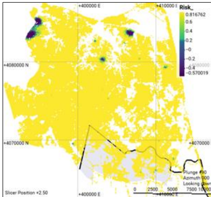
Figure 6. P90 groundwater-level map illustrating conservative scenarios with expanded shallow conditions in central and southern urban areas.
