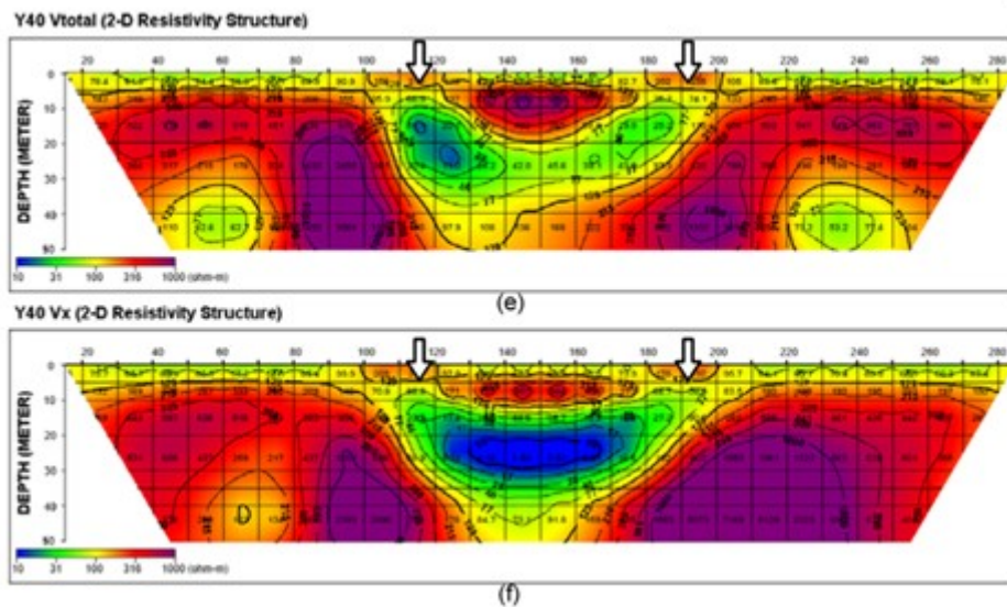
Figure 9(continued). (e)-(f) Y40, \Delta V_{total} and \Delta V_x . Arrows indicate the position of the conductive anomaly.
