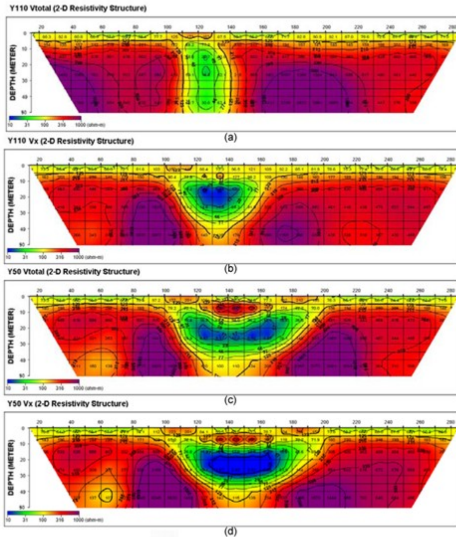
Figure 9. Illustrative 2D inversion results for three representative profiles (Y110, Y50, and Y40) from the model shown in Figure 2a, comparing inversions based on full horizontal potential-difference data ( \Delta V_{total} ) and conventional inline-only data ( \Delta V_x ), with a resistivity contrast of 1000:1. (a)-(b) Y110, \Delta V_{total} and \Delta V_x ; (c)-(d) Y50, \Delta V_{total} and \Delta V_x
